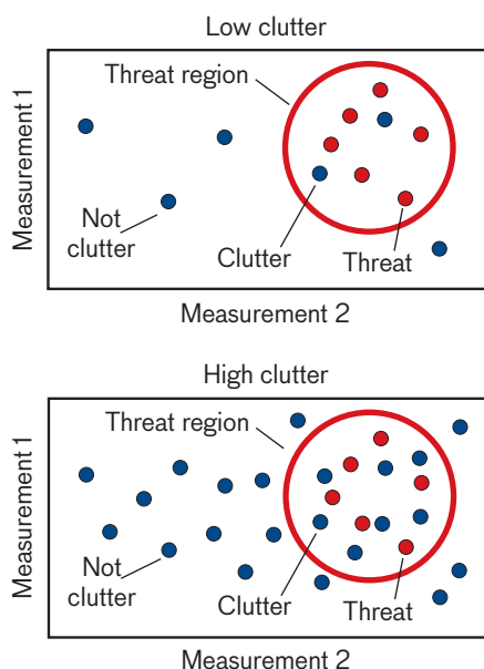
FIGURE 4. Clutter affects the ability of a trigger sensor to discriminate threat particles. Each dot represents a particle and its associated measurements. In this case each has very low noise. The blue dots are nonthreat particles and the red dots are threat particles. The measurement region in which threat particles are expected is shown by the red circle.
