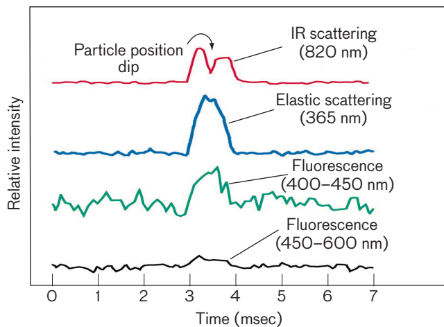
FIGURE 19. Four outputs from the BAST system appear at the same times, indicating that the data are from a single particle. Here, the raw signals are from a single 3 μm Bg spore.
