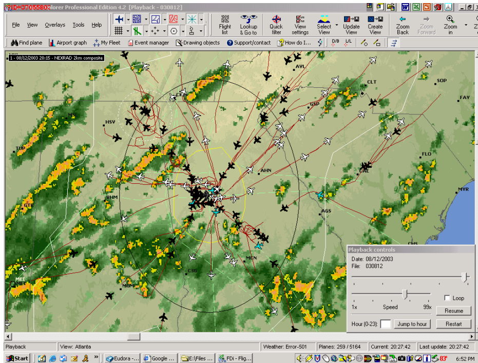
Figure 28. Aircraft tracks and weather at Atlanta on 12 August 2003. Note holding patterns that bracket the 100 nmi distance from ATL.
