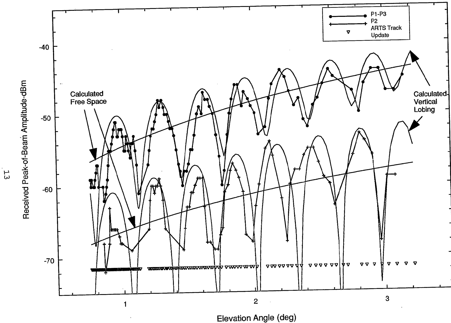
Figure 5. SSR Vertical Lobing Pattern—65-Degree Radial / Altitude = 4000 feet / Bottom AMF Antenna.
