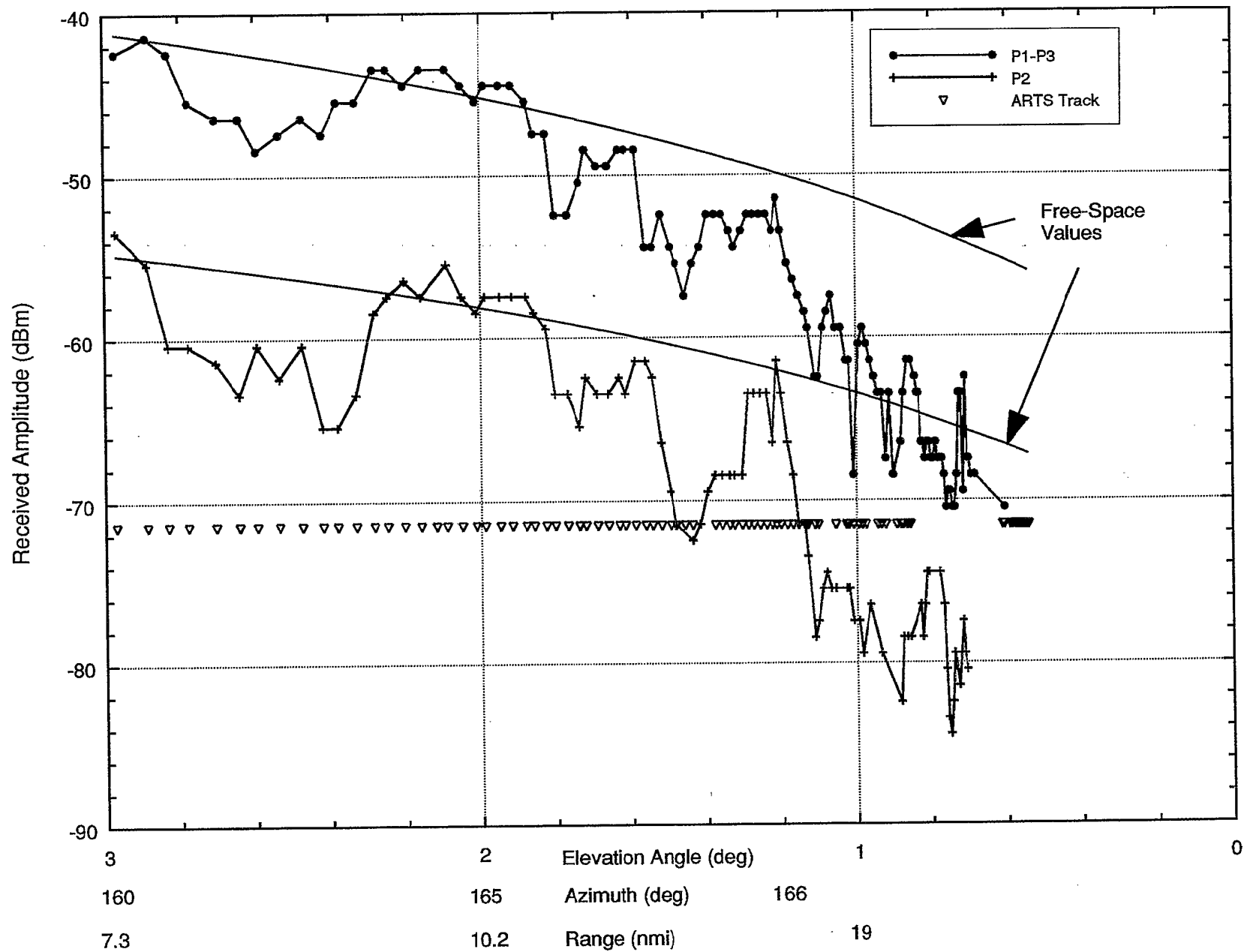
Figure 14. SSR Elevation Pattern—170-Degree Radial / Altitude = 3000 feet / Bottom AMF Antenna.
