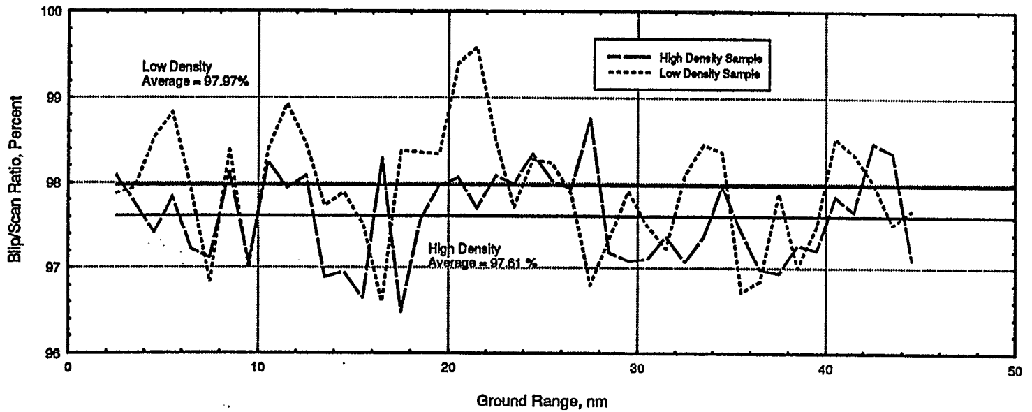
Figure 36. Total Track Reports and Blip/Scan Ratio vs. Ground Range - Both Data Samples.
