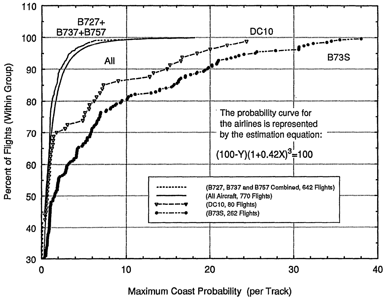
Figure 47. Maximum Single Track Coast Probabilities. Comparison Between Airlines / Chicago CDR Data Sample - 6:42 pm 10/21/91 to 7:13 am 10/23/91.
