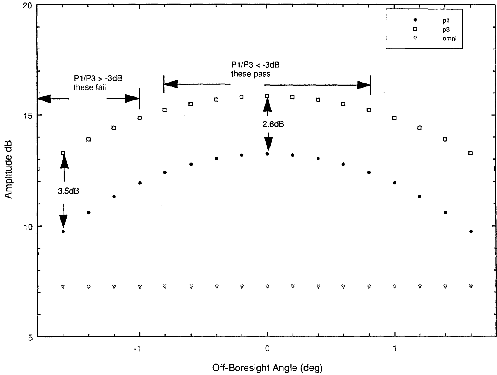
Figure 23. SSR Horizontal Pattern: P1/P2 = 6 dB — Azimuth Sweep at Elevation Angle = .838 degrees Adjusted Differential Feed Phase = 127 Degrees
