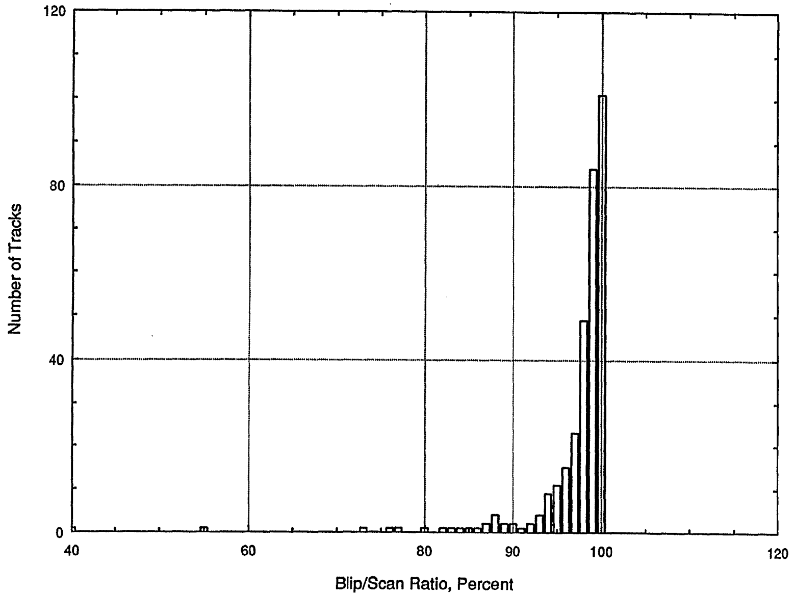
Figure 32. Single Track Blip/Scan Ratios by Major Airlines Histogram - High-Density CDR Sample. Short Tracks Eliminated; No Surveillance Screening Applied
