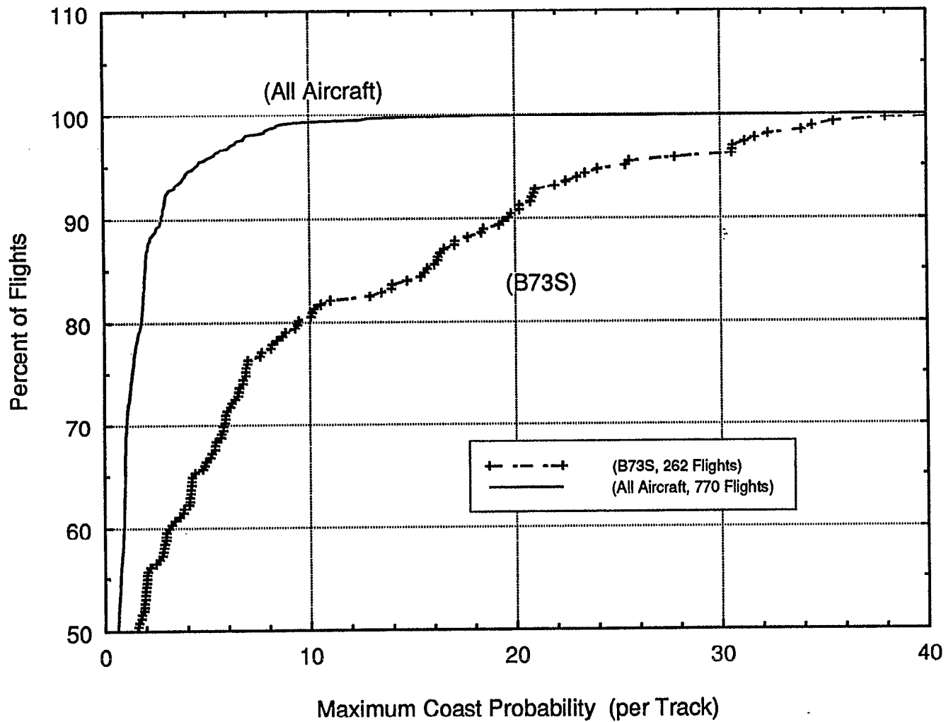
Figure 42. Maximum Single Track Coast Probabilities. Coasting Compared Between B73S and All Aircraft / Chicago CDR Data Sample - 6:42 pm 10/21/91 to Noon 10/23/91.
