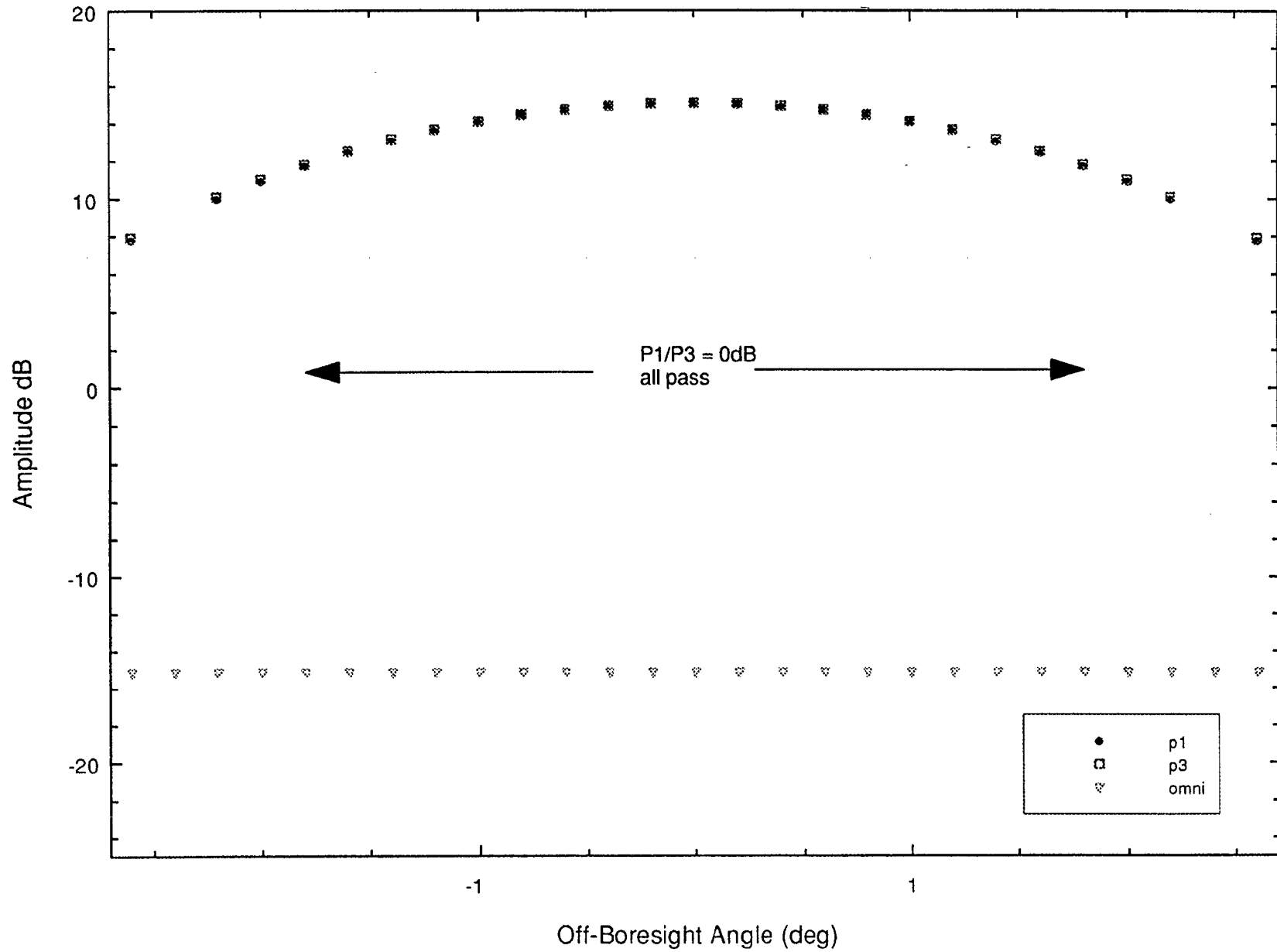
Figure 21. SSR Horizontal Pattern: P1/P2 > 24 dB — Azimuth Sweep at Elevation Angle = 1.08 degrees.
