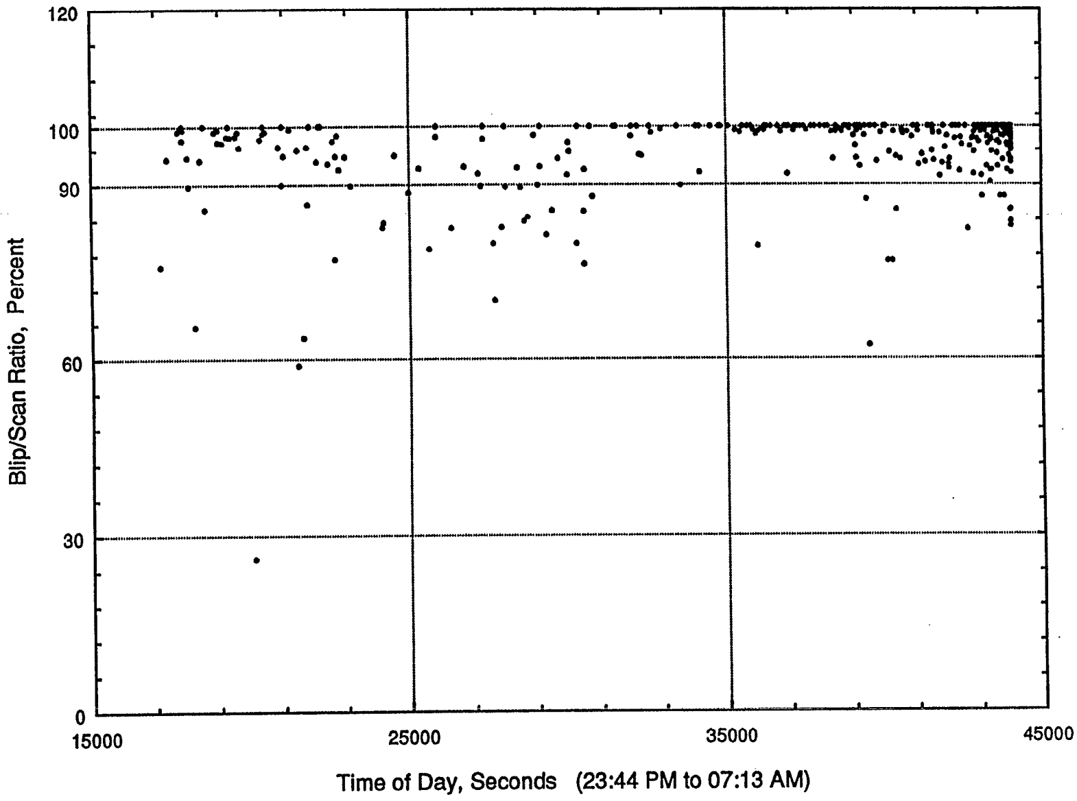
Figure 31. Single Track Blip/Scan Ratios by Airlines - Low-Density CDR Sample. Short Tracks Eliminated; No Surveillance Screening Applied
