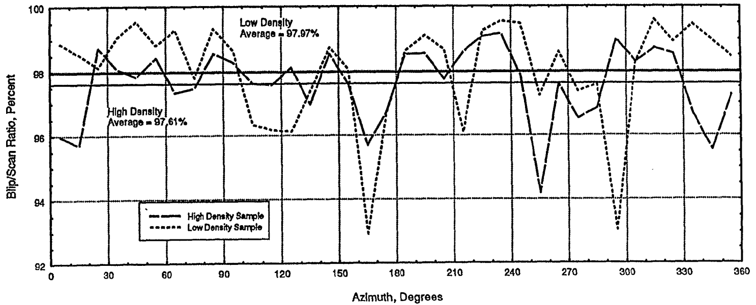
Figure 34. Total Track Reports and Blip/Scan Ratio vs. Azimuth - Both Data Samples.
