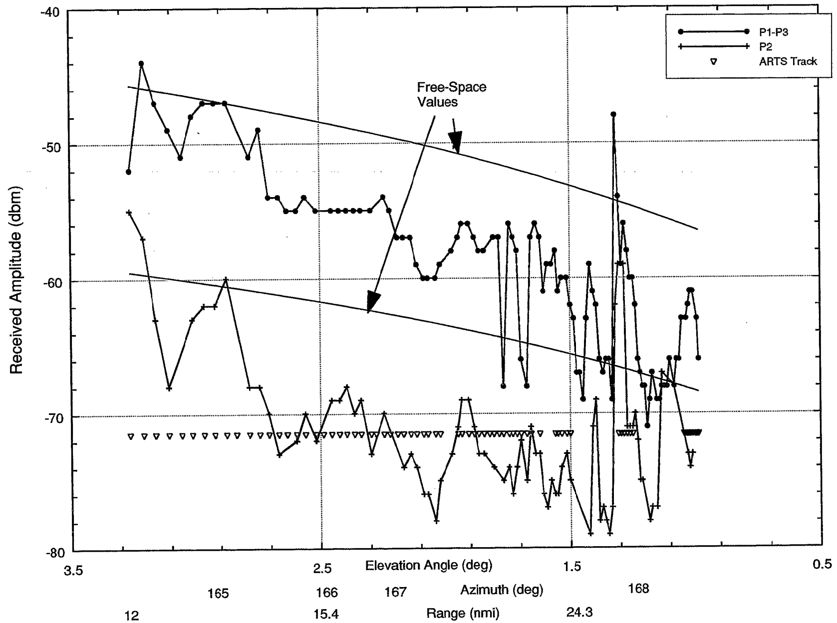
Figure 15. SSR Elevation Pattern—170-Degree Radial / Altitude = 5000 feet / Bottom AMF Antenna.
