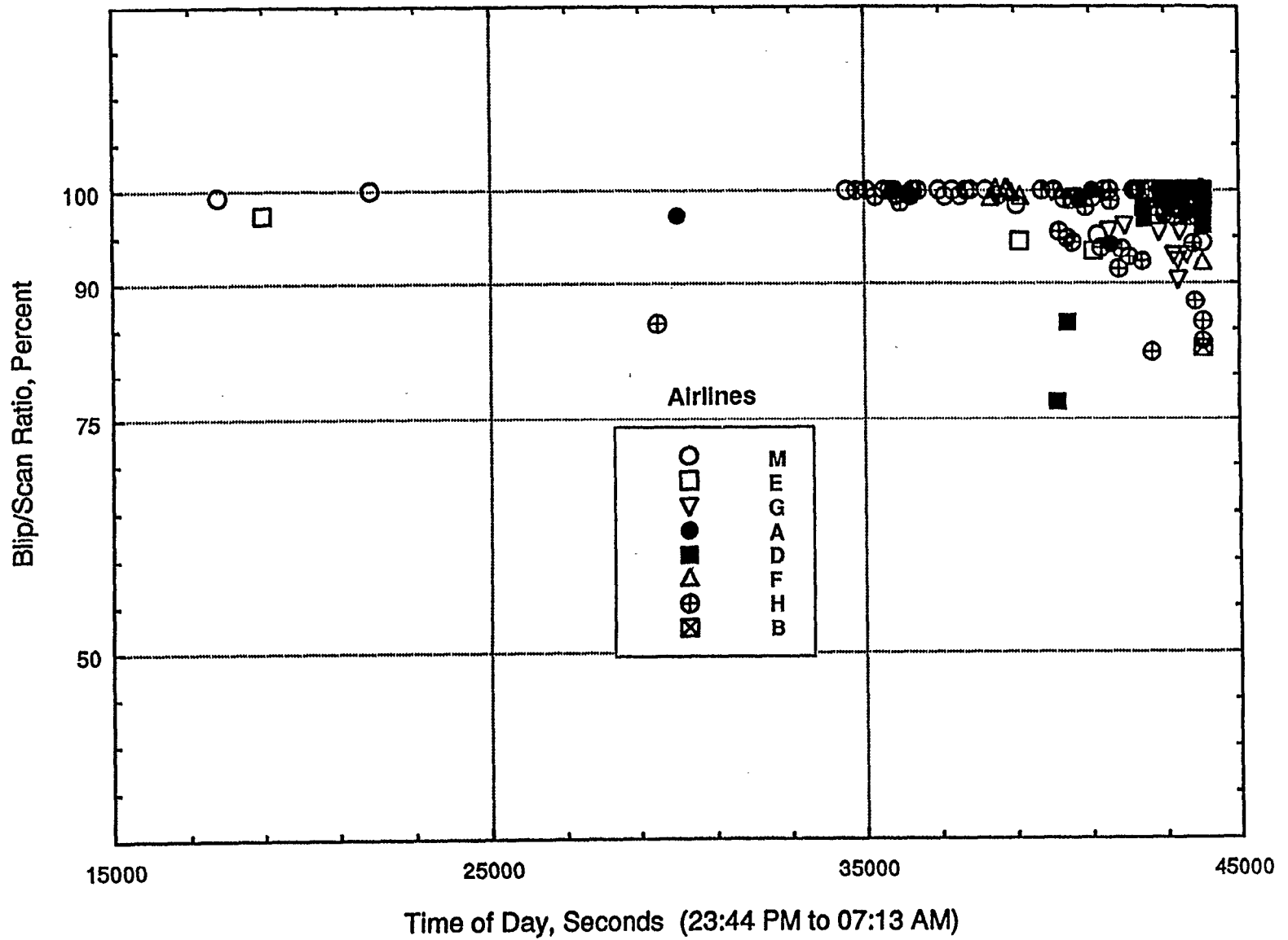
Figure 30. Single Track Blip/Scan Ratios by Major Airlines - Low-Density CDR Sample. Short Tracks Eliminated; No Surveillance Screening Applied
