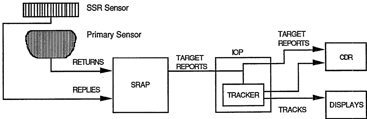
Figure 27. Simple Block Diagram of Radar Data Processing and Storage.
