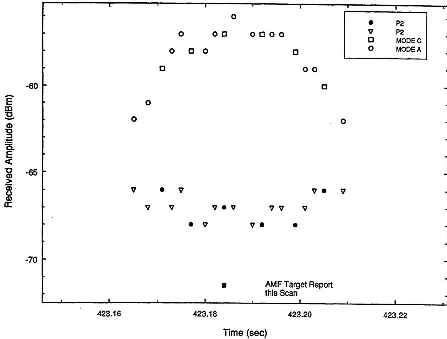
Figure 6. SSR Azimuth Pattern — 1.75-Degree Elevation / 65-Degree Radial / Altitude = 4000 feet.
