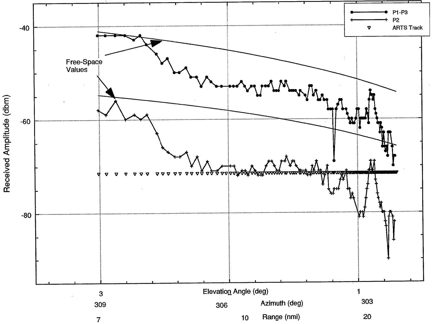
Figure 17. SSR Elevation Pattern—300-Degree Radial / Altitude = 3000 feet / Bottom AMF Antenna.
