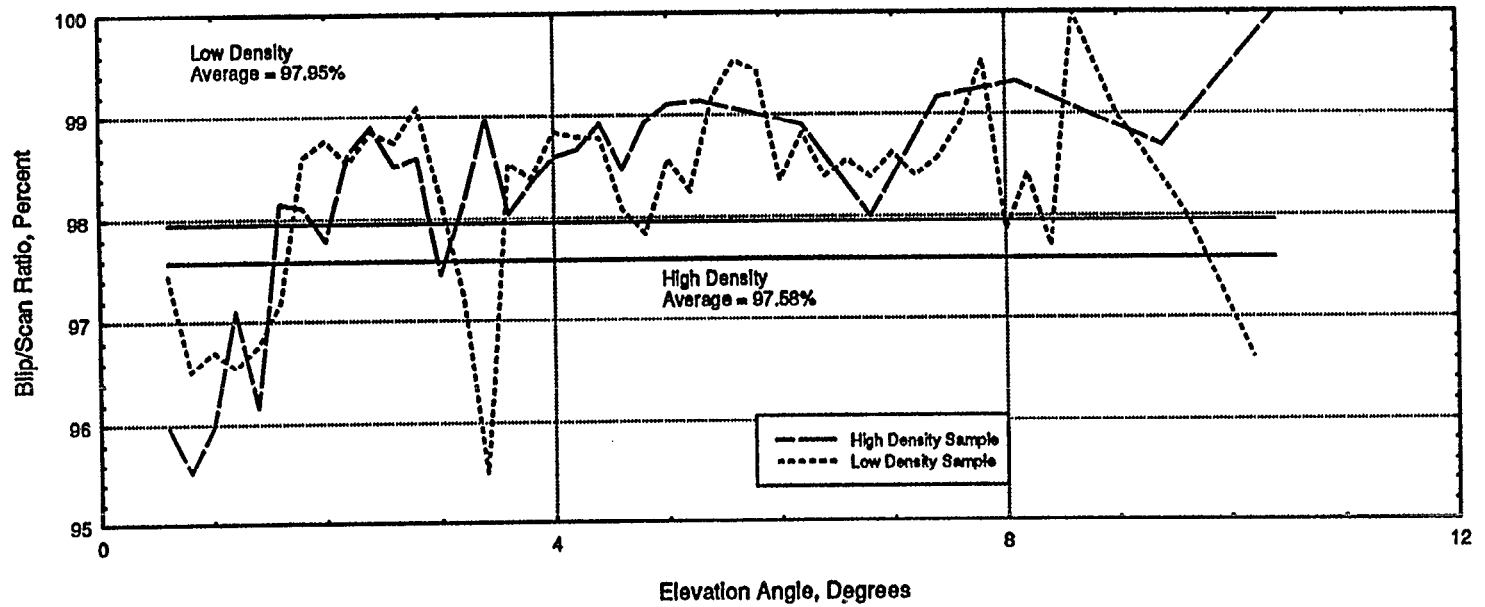
Figure 35. Total Track Reports and Blip/Scan Ratio vs. Elevation Azimuth - Both Data Samples.
