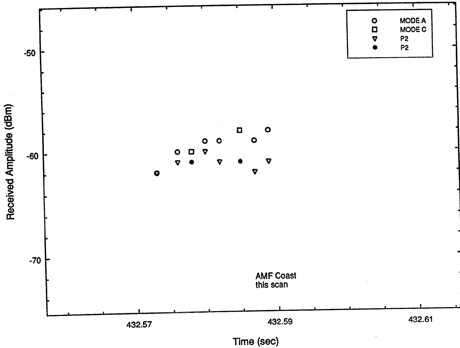
Figure 7. SSR Azimuth Pattern — 1.75-Degree Elevation / 65-Degree Radial / Altitude = 4000 feet.
