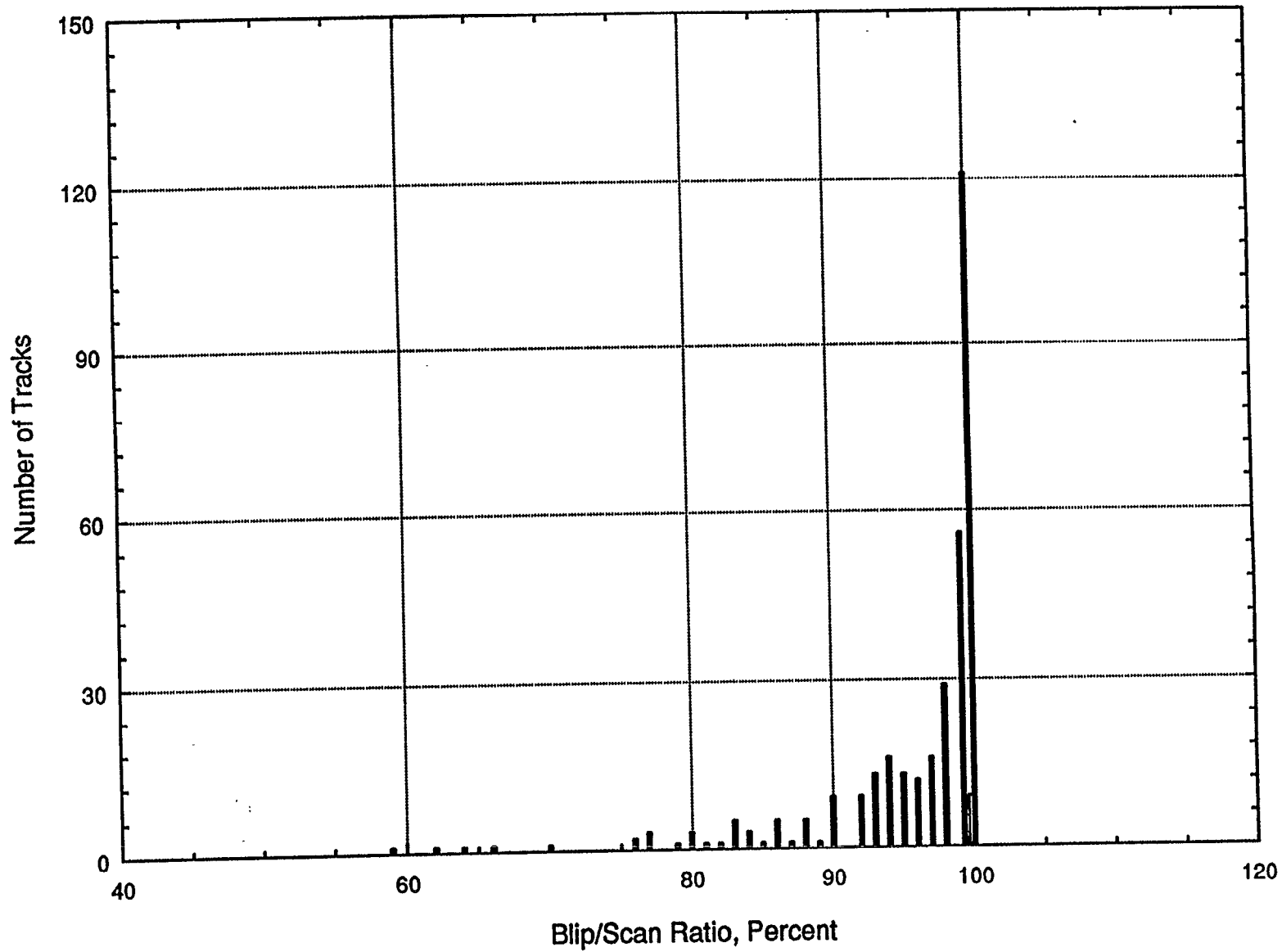
Figure 33. Single Track Blip/Scan Ratios by Airlines Histogram - Low-Density CDR Sample. Short Tracks Eliminated; No Surveillance Screening Applied
