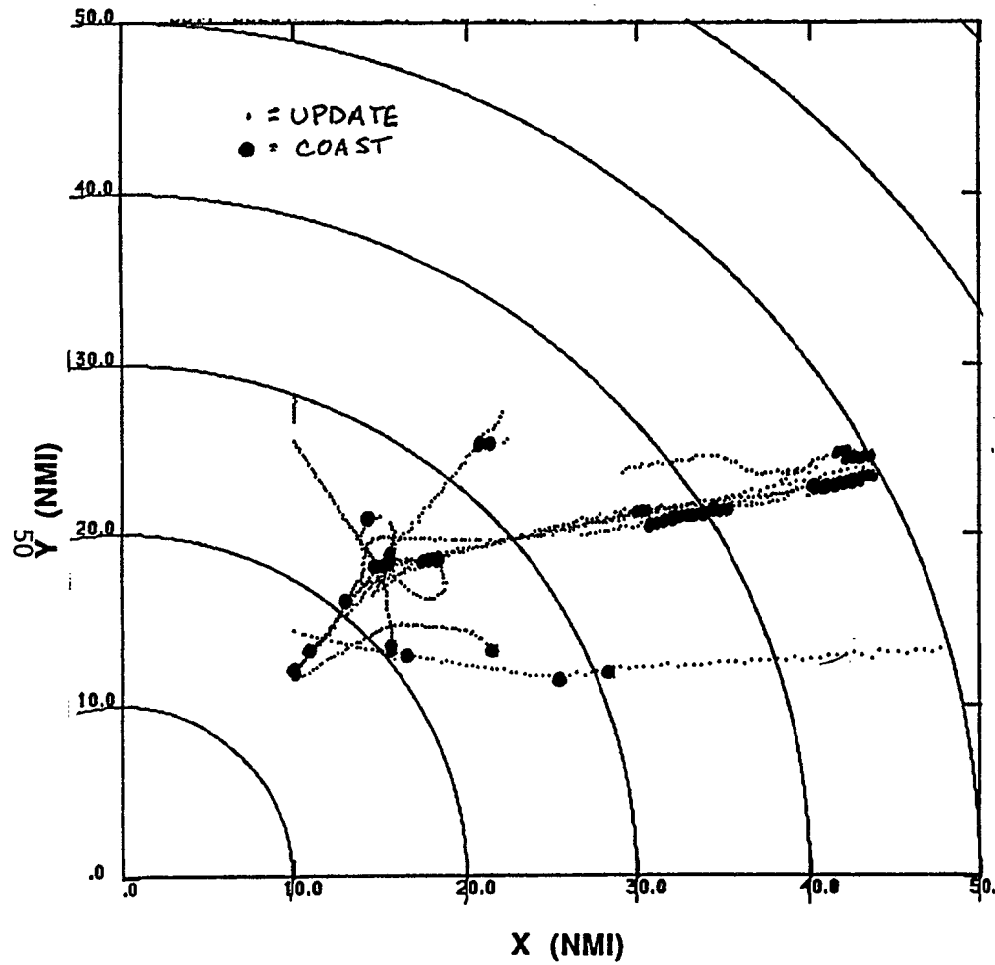
Figure 26a. Radar Tracks Along V84 (from 10/22/91 CDR data).
