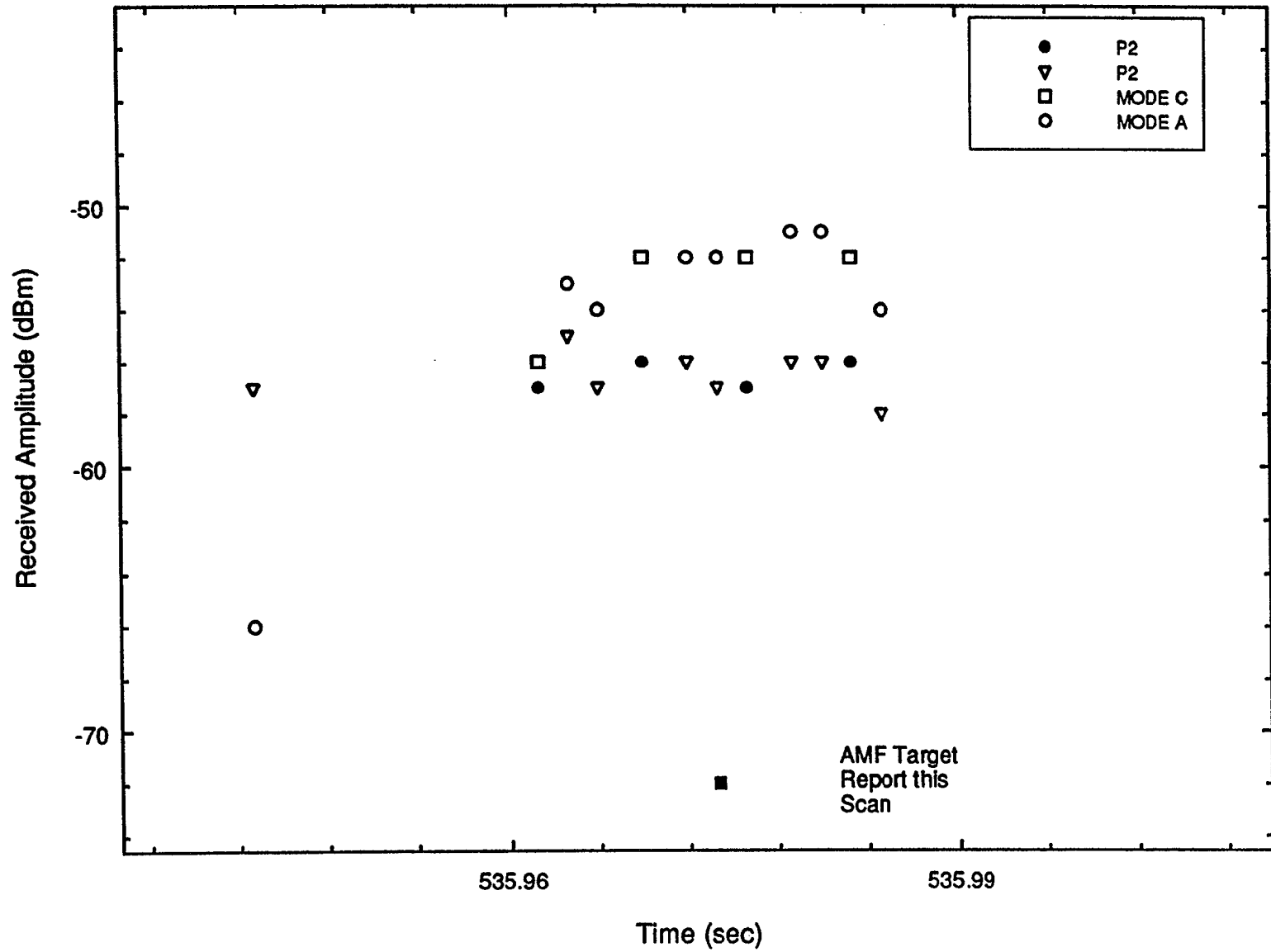
Figure 10. SSR Azimuth Pattern—2.4-Degree Elevation / 65-Degree Radial / Altitude = 4000 feet.
