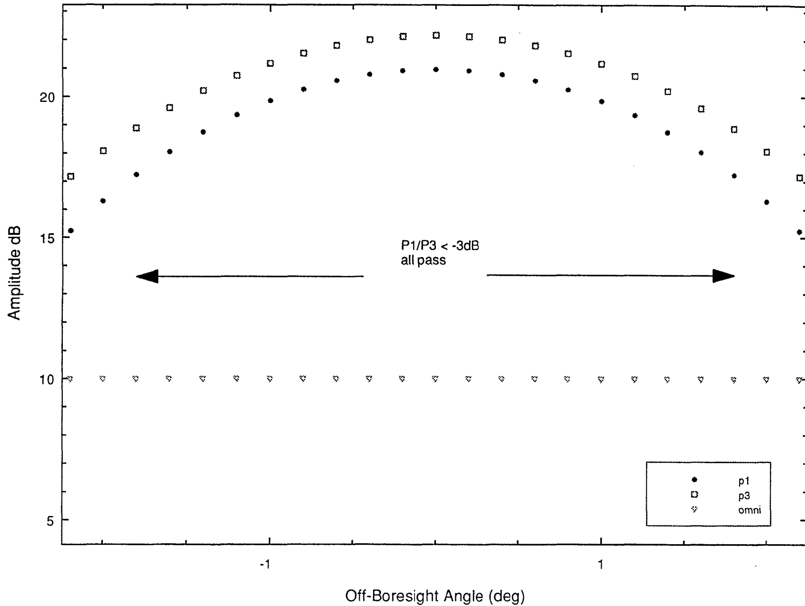
Figure 22. SSR Horizontal Pattern: P1/P2 = 11 dB — Azimuth Sweep at Elevation Angle = .922 degrees Adjusted Differential Feed Phase = 93 Degrees
