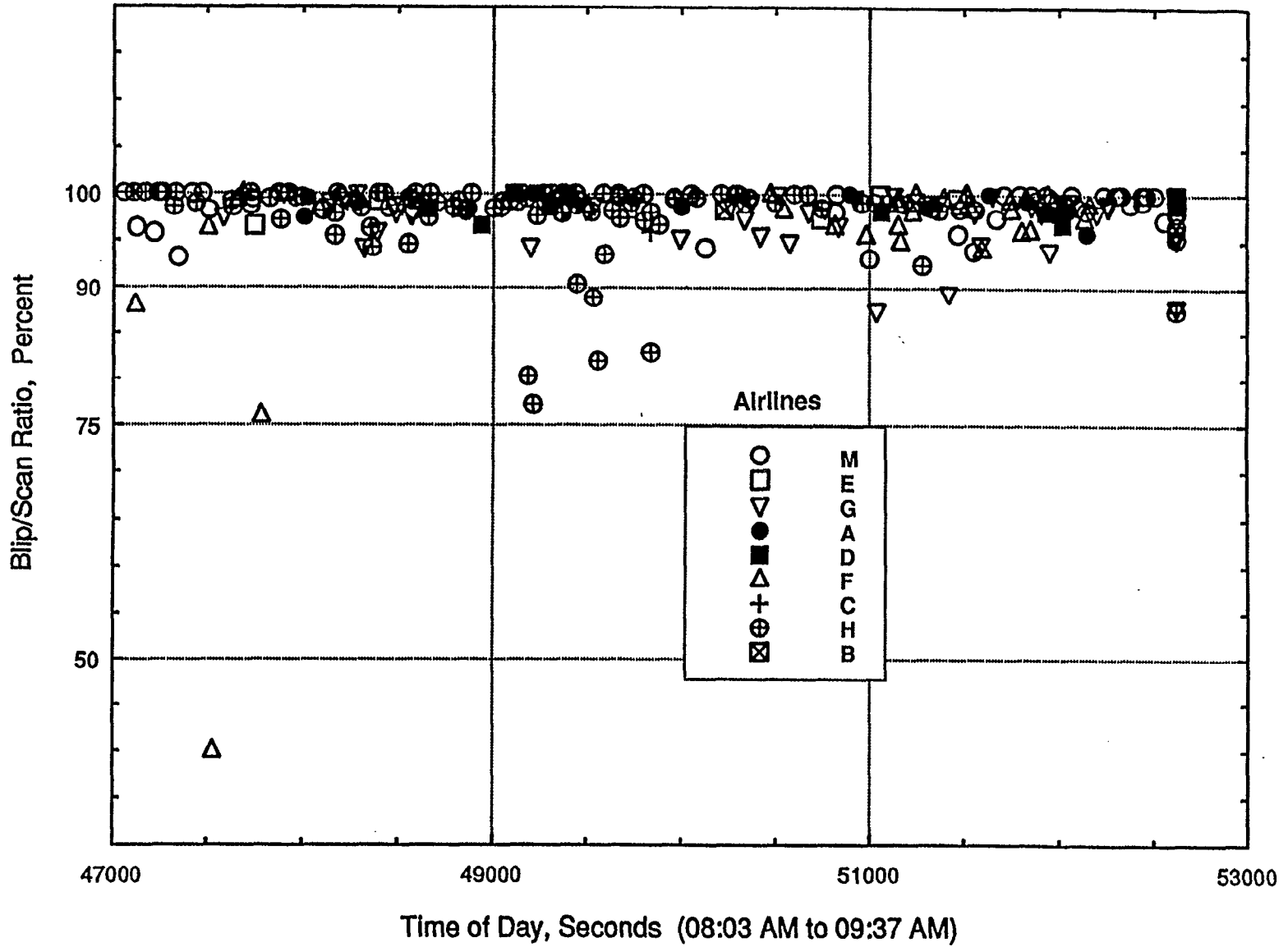
Figure 28. Single Track Blip/Scan Ratios by Major Airlines - High-Density CDR Sample. Short Tracks Eliminated; No Surveillance Screening Applied
