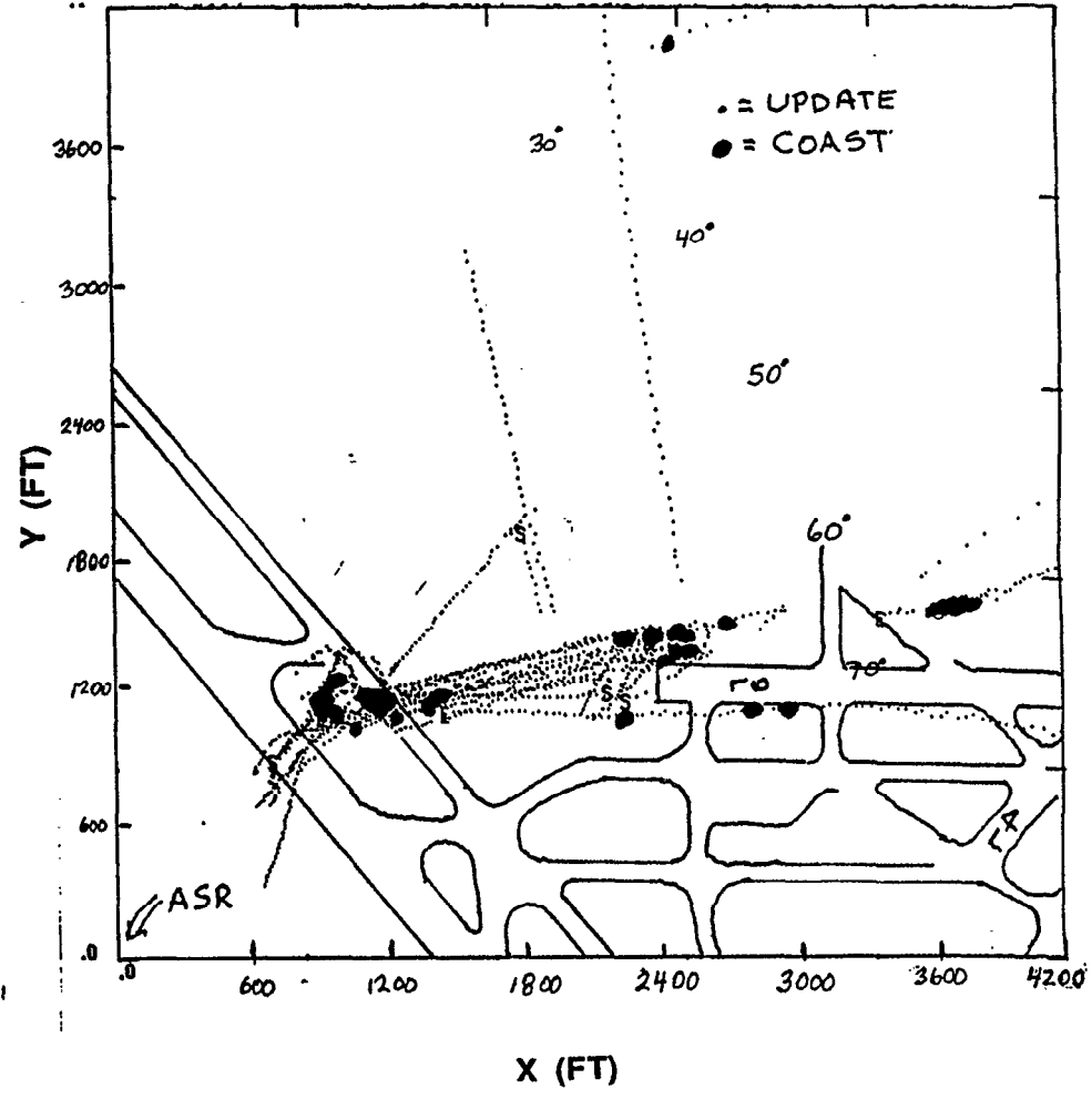
Figure 24b. Fresnel Zone Center Corresponding to Radar Tracks in Figure 24a.
