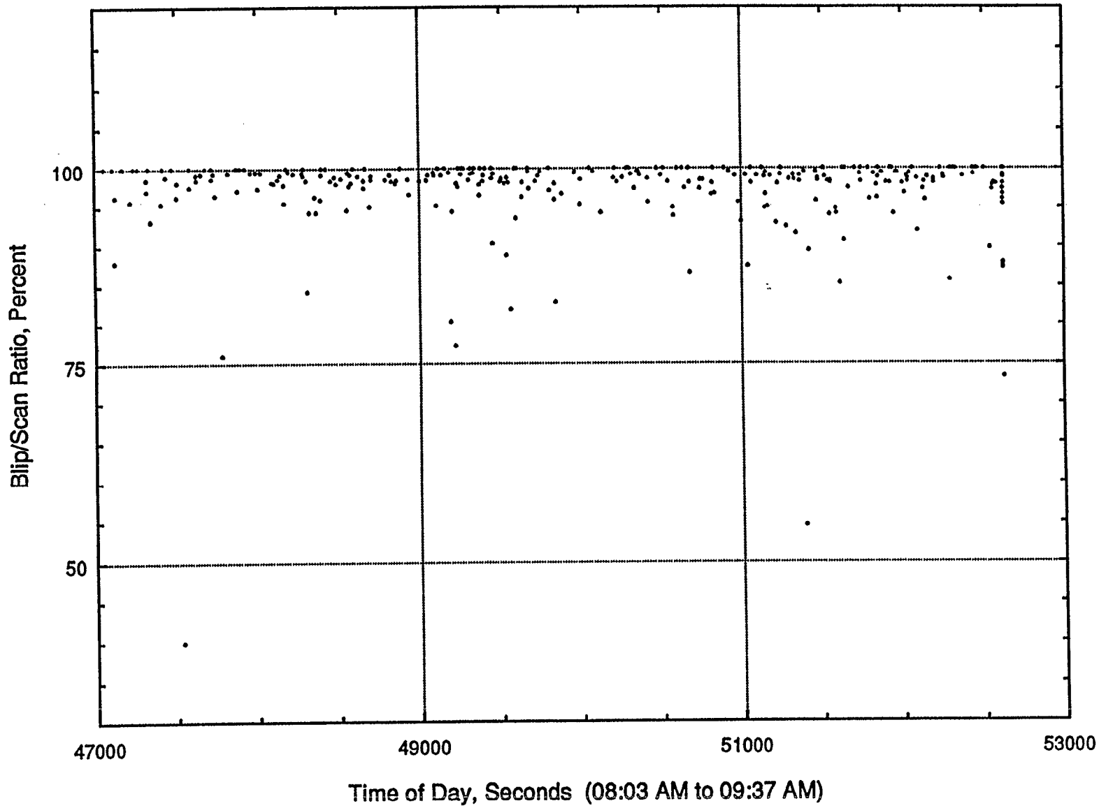
Figure 29. Single Track Blip/Scan Ratios by Airlines - High-Density CDR Sample. Short Tracks Eliminated; No Surveillance Screening Applied
