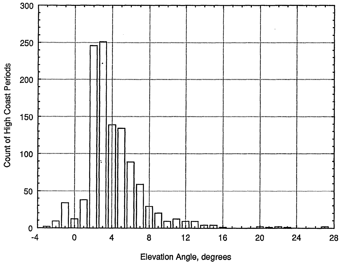
Figure 39. Distribution of High Coast Periods by Elevation Angle. All High Coast Periods - No Surveillance Limits Applied / April to December 1991 CDR Extracts from Chicago.
