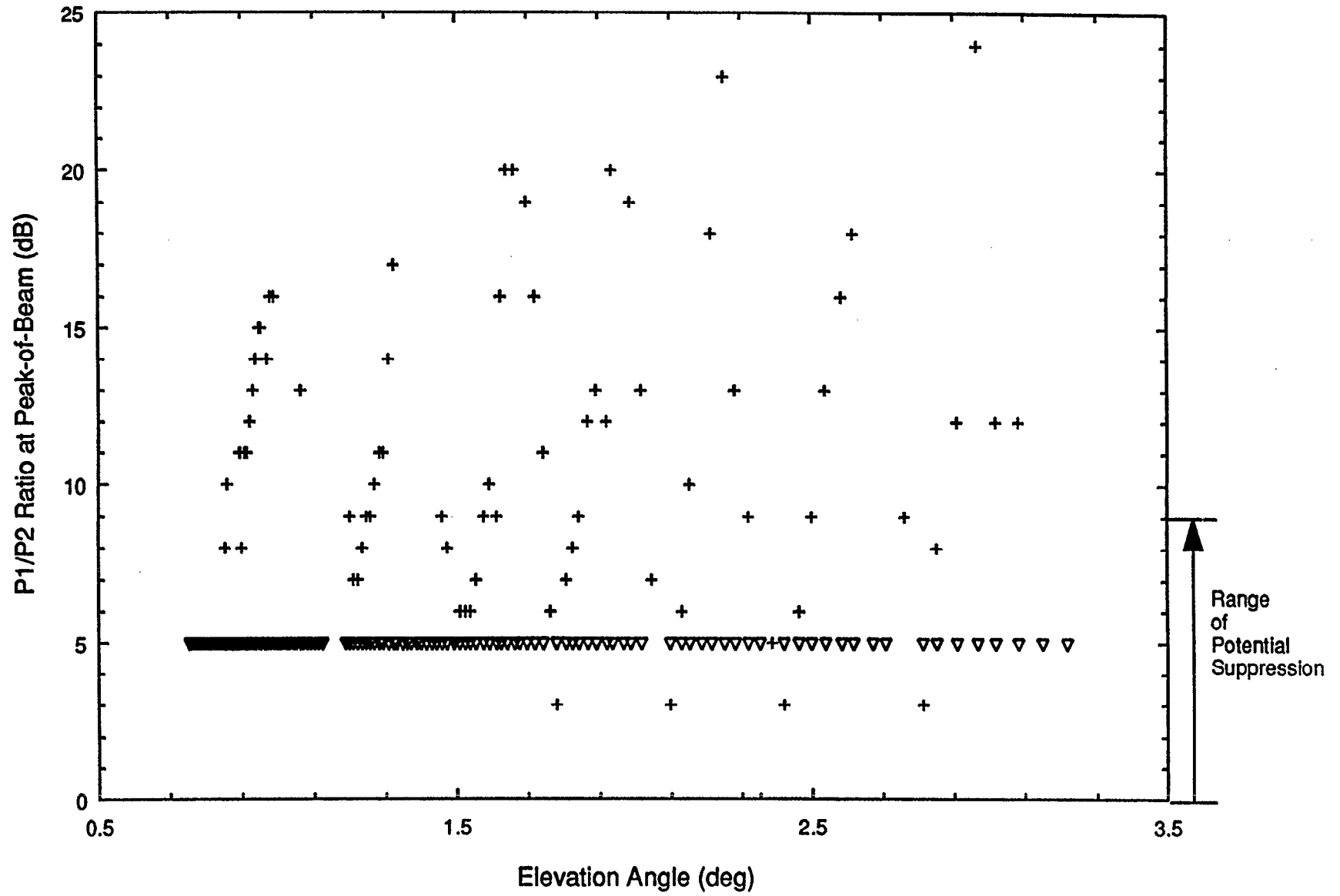
Figure 13. Peak-of-Beam P1/P2 Ratio at AMF vs Elevation Angle / 65-Degree Radial / Altitude = 4000 feet / Bottom AMF Antenna.
