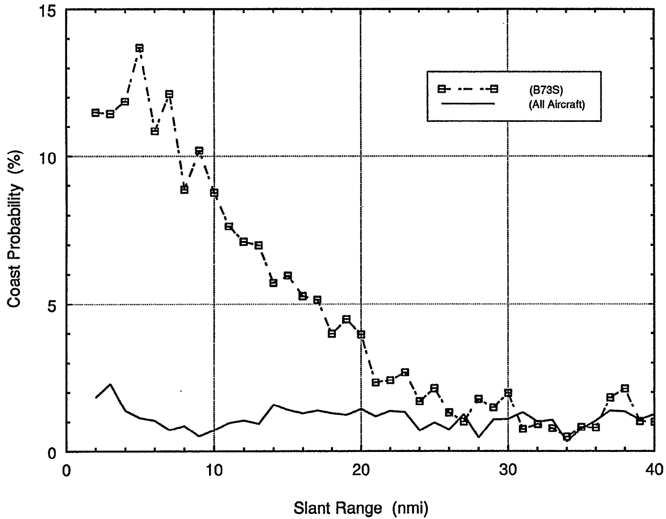
Figure 45. Probability of Coasting vs Slant Range for Selected Airline and Aircraft Type. Comparison Between B73S and All Aircraft / Chicago CDR Sample - 6:42 pm 10/21/91 to Noon 10/23/91.
