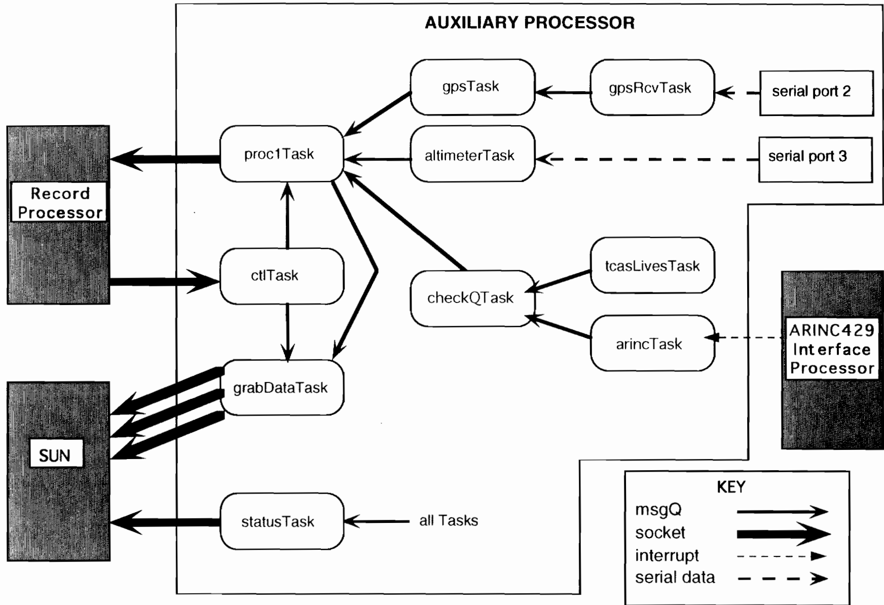
Figure B 2. AMF Auxiliary Processor Communication Channels.
