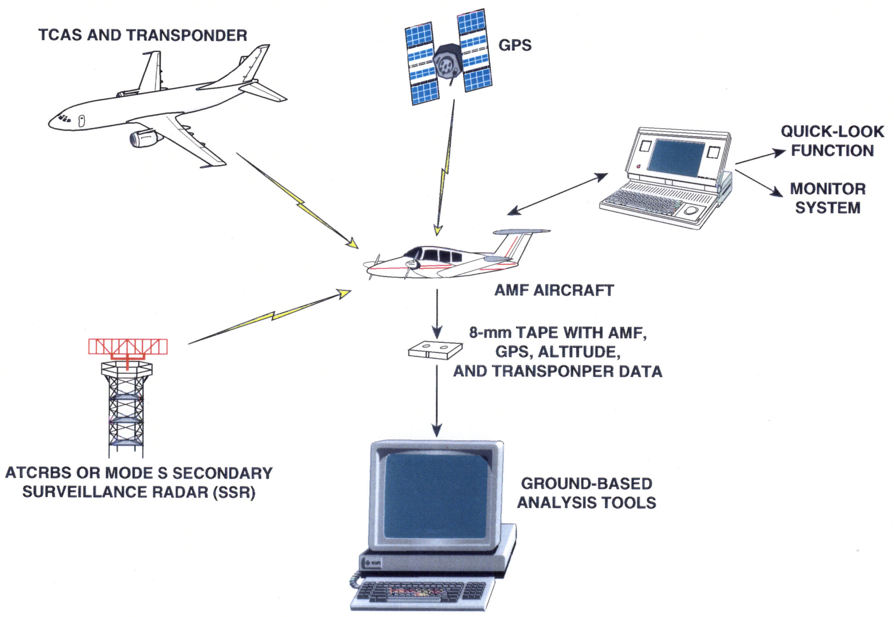
Figure 1. AMF System Concept.
