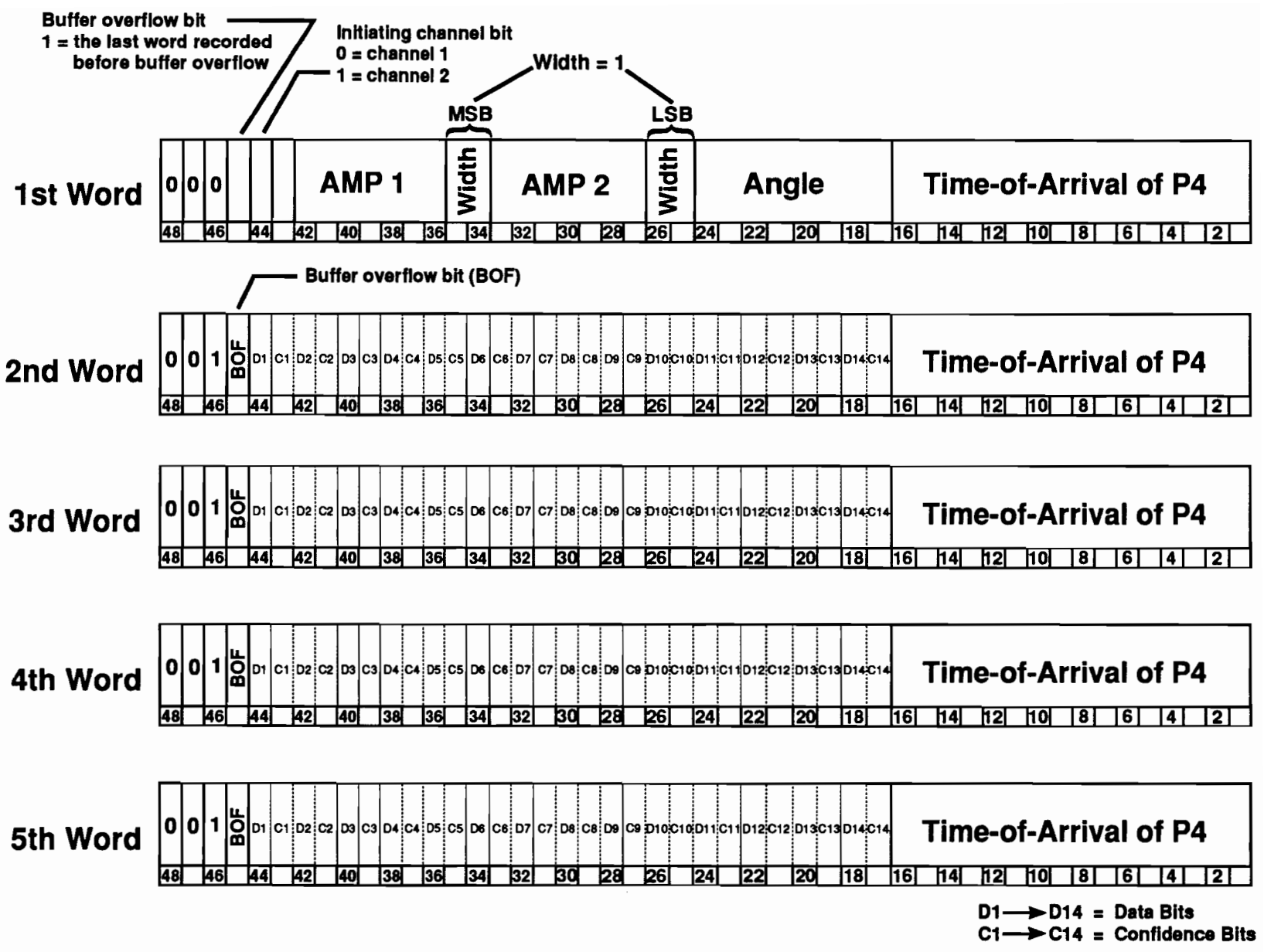
Figure A-3f. Format of Mode S Data Words.
