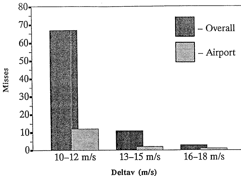
Figure 2-3. Velocity statistics for 1990 Orlando algorithm misses.
