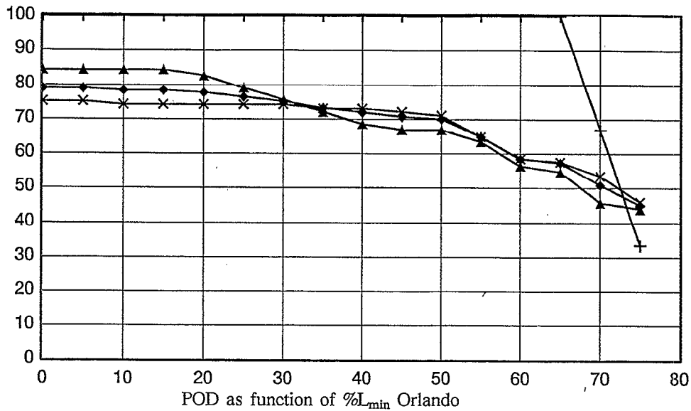
Figure 3-1. Probability of detection as a function of minimum percent of length detected threshold for moderate (x), strong (▲), severe (+) and all (♦) gust fronts.
