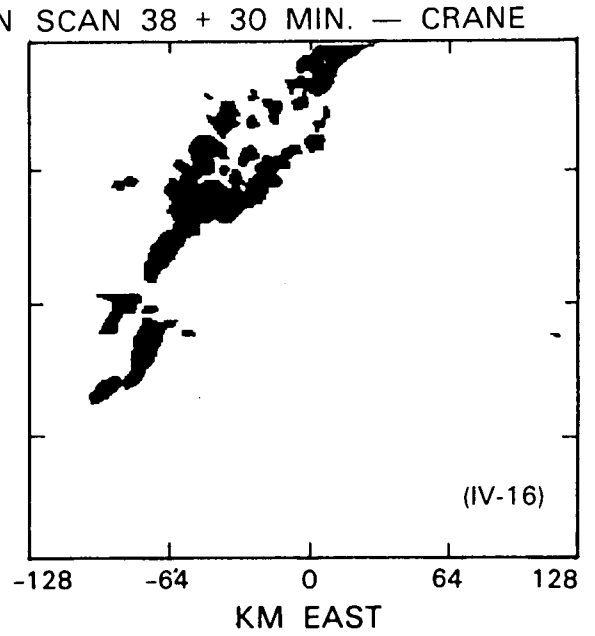
Figure IV-13. to IV-16. M.I.T. 8/11/81 30 dBz.
