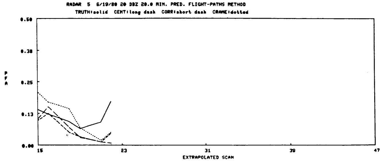
Figure IV-62. 6/19/80 20 min. pred., Flight-paths method.
