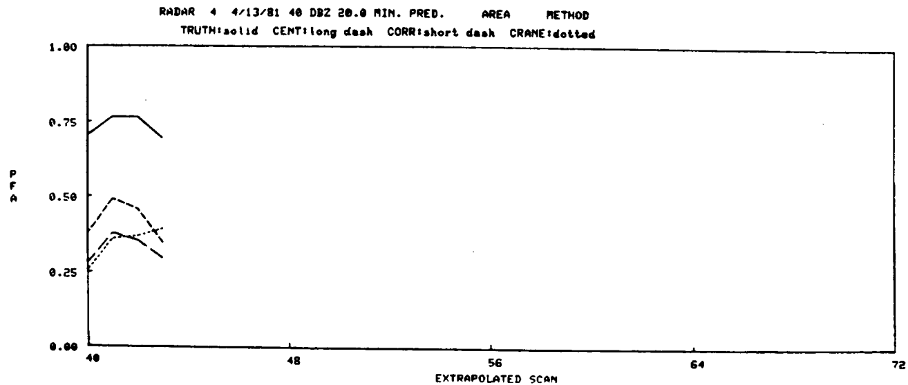
Figure IV-67. 4/13/81 20 min. pred., Area method.
