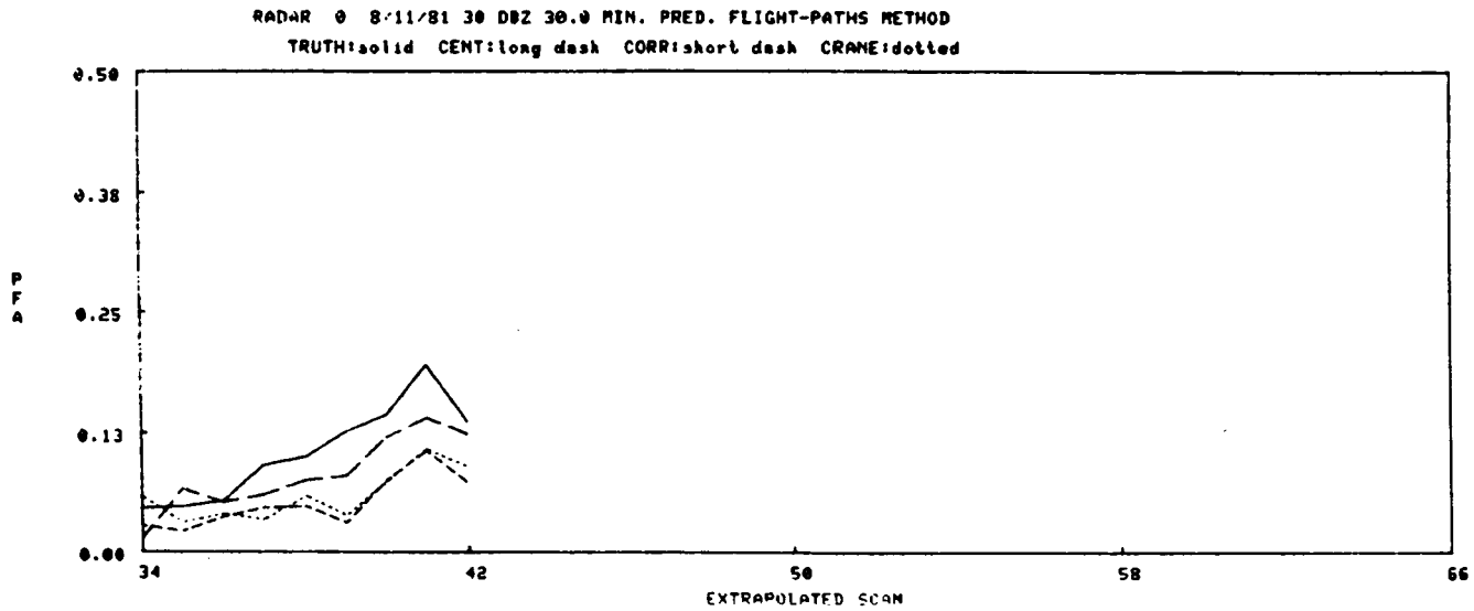
Figure IV-52. 8/11/81 30 min. pred., Flight-paths method.
