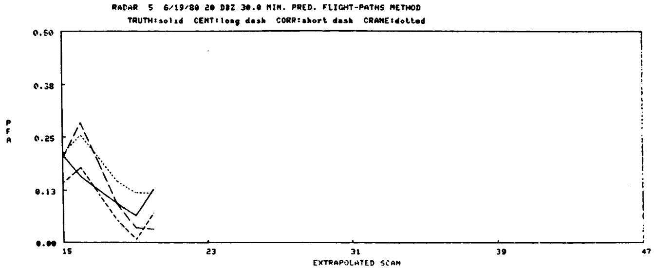
Figure IV-64. 6/19/80 30 min. pred., Flight-paths method.
