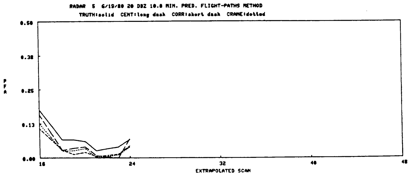
Figure IV-60. 6/19/80 10 min. pred., Flight-paths method.
