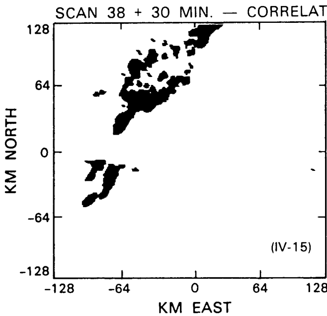
Figure IV-13. to IV-16. M.I.T. 8/11/81 30 dBz.
