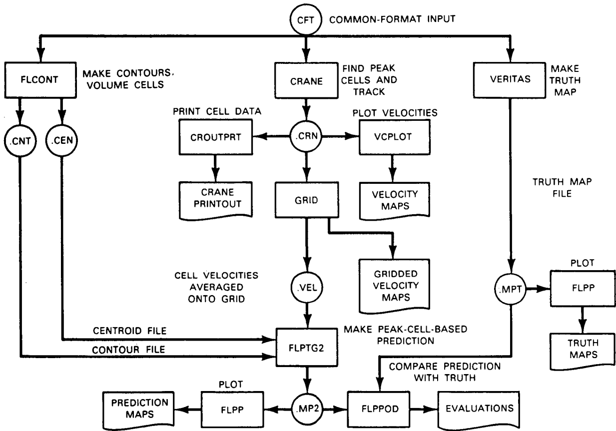
Figure B-3. Crane-tracker flowchart.
