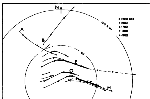
The paths of several cumulonimbus near Oklahoma City on the afternoon of 26 May 1963, as determined by radar situated at the center of the range rings. The thickened lines indicate where the storms were severe and had hook echoes (191).
