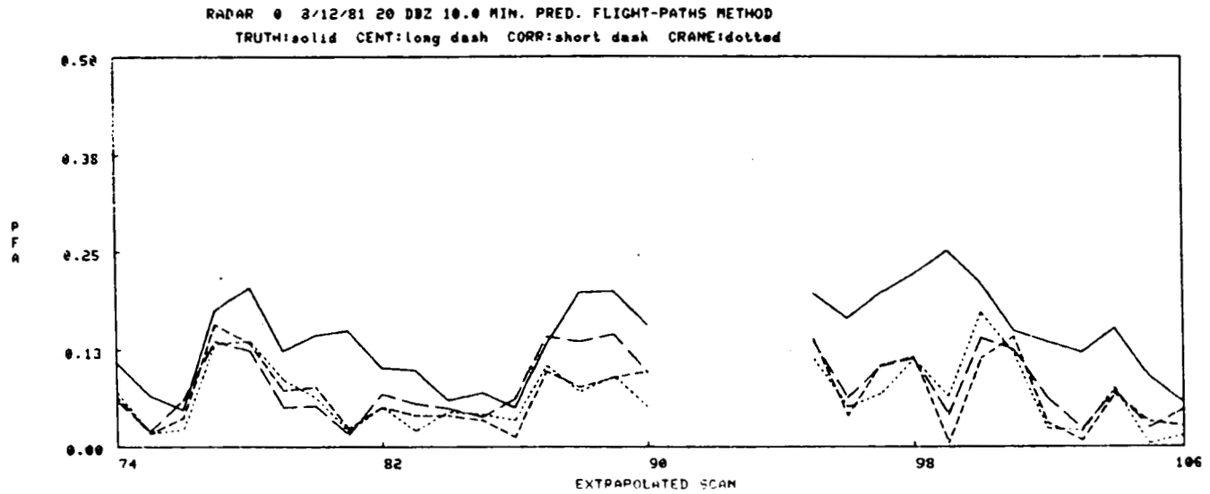
Figure IV-54. 8/12/81 10 min. pred., Flight-paths method.
