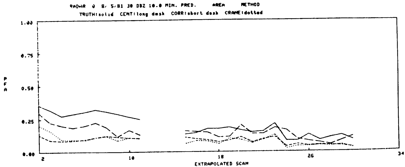
Figure IV-41. 8/5/81 10 min. pred., Area method.
