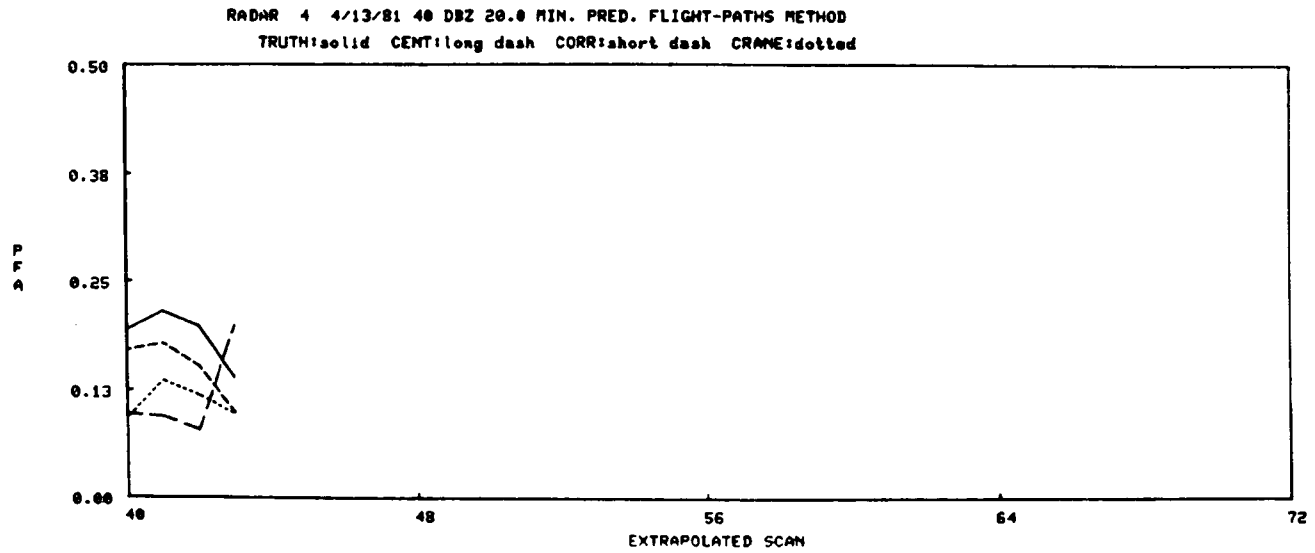
Figure IV-68. 4/13/81 20 min. pred., Flight-paths method.
