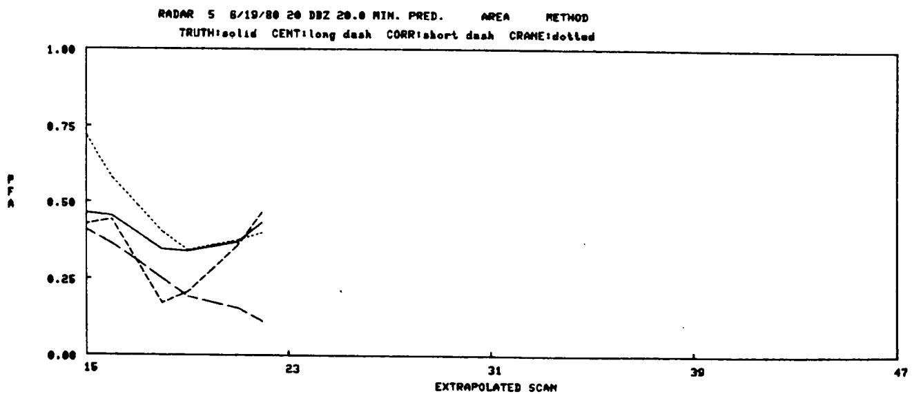
Figure IV-61. 6/19/80 20 min. pred., Area method.
