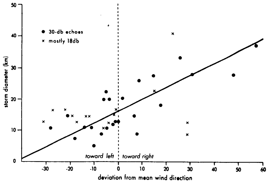
Deviation of storm motion from direction of mean wind as a function of echo diameter. Regression line based on radar echo observations as shown. (After Newton and Fankhauser 1964 a,b .)
