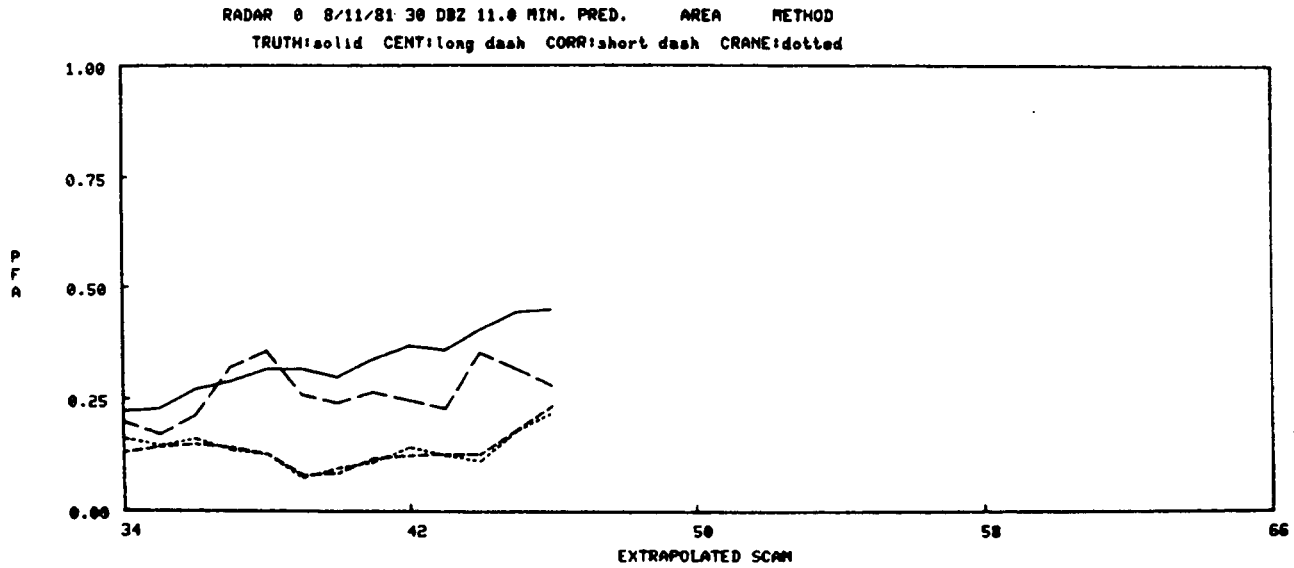
Figure IV-47. 8/11/81 11 min. pred., Area method.
