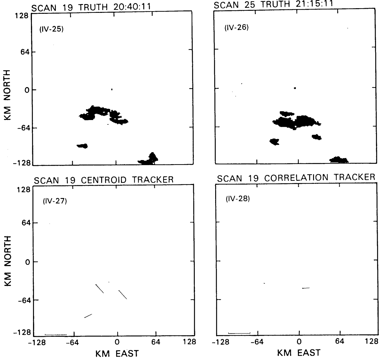
Figure IV-25. to IV-28. NSSL/C 6/19/80 20 dBz.
