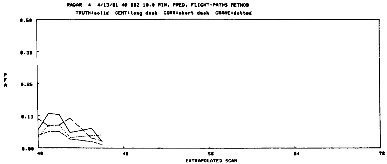
Figure IV-66. 4/13/81 10 min. pred., Flight-paths method.
