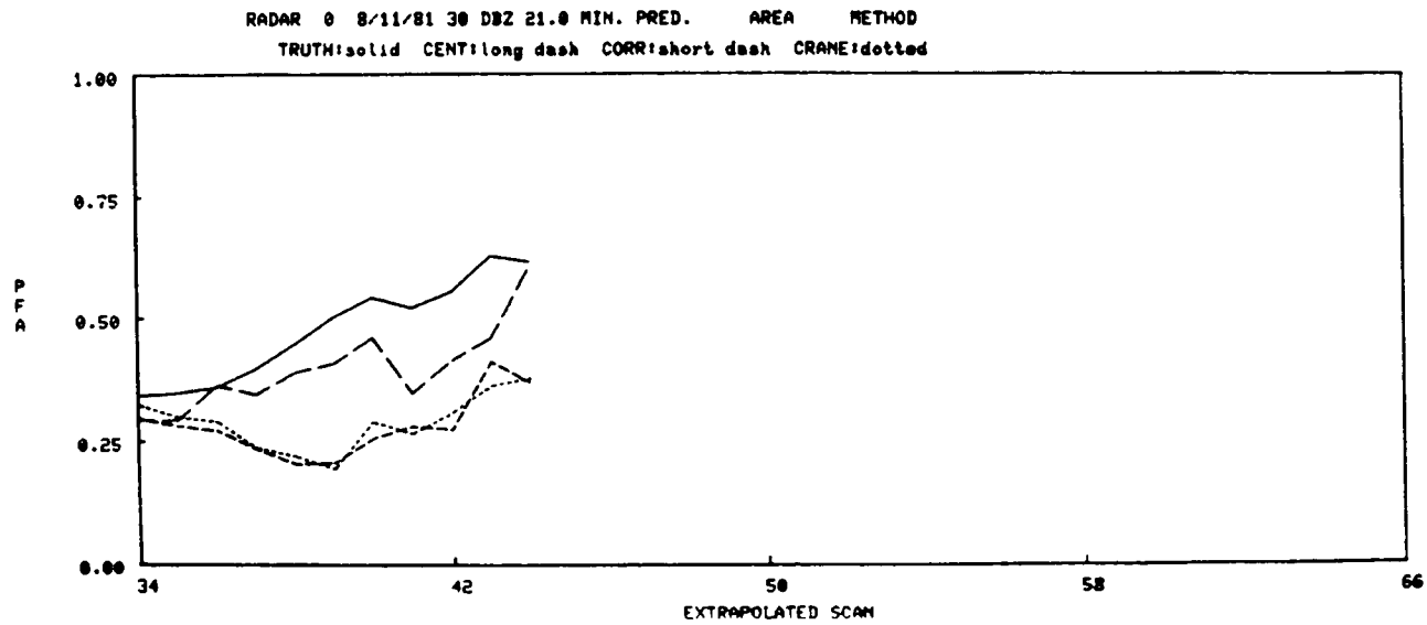
Figure IV-49. 8/11/81 21 min. pred., Area method.
