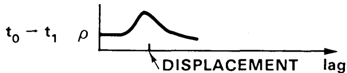
Figure II-1. Tracking/prediction methods we have evaluated.
