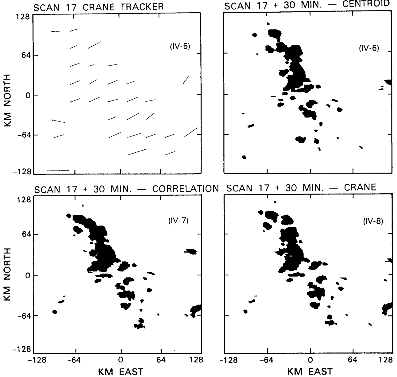
Figure IV-5. to IV-8. M.I.T. 8/5/81 30 dBz.
