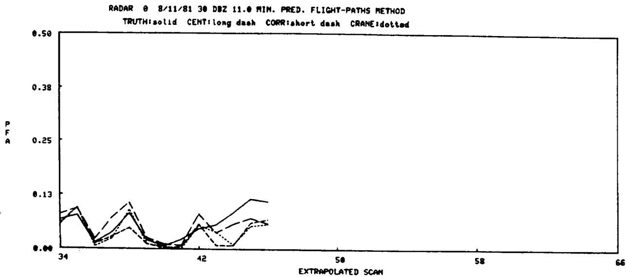
Figure IV-48. 8/11/81 11 min. pred., Flight-paths method.
