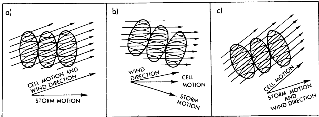
Schematic diagrams of storm movement by propagation (see text). (After Marwitz, 1972b.)
