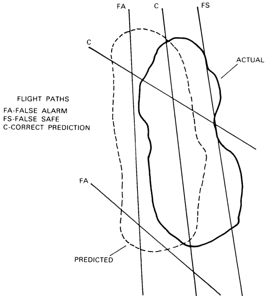
Figure III-1. Objective evaluation of forecasts.
