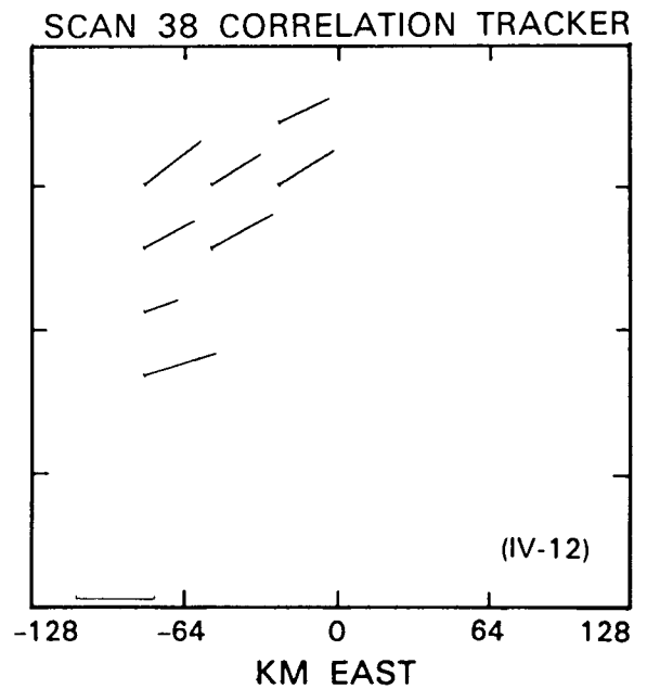
Figure IV-9. to IV-12. M.I.T. 8/11/81 30 dBz.
