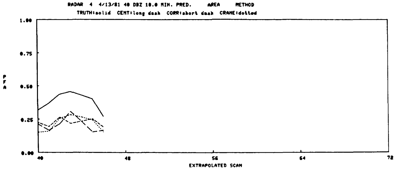
Figure IV-65. 4/13/81 10 min. pred., Area method.
