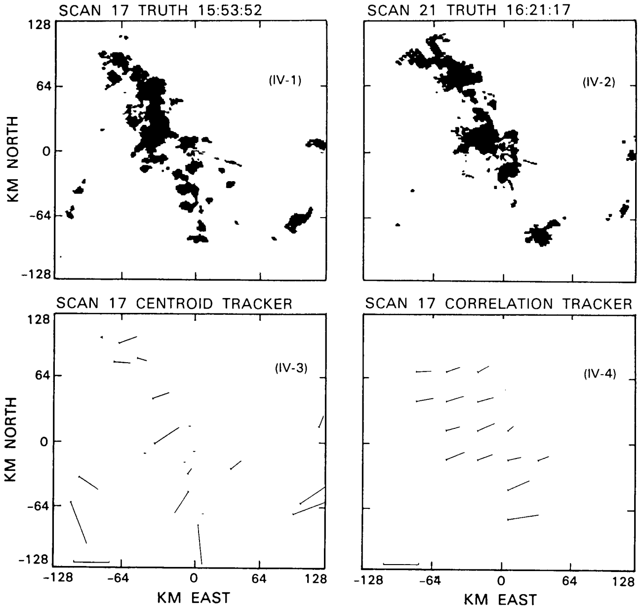
Figure IV-1. to IV-4. M.I.T. 8/5/81 30 dBz.
