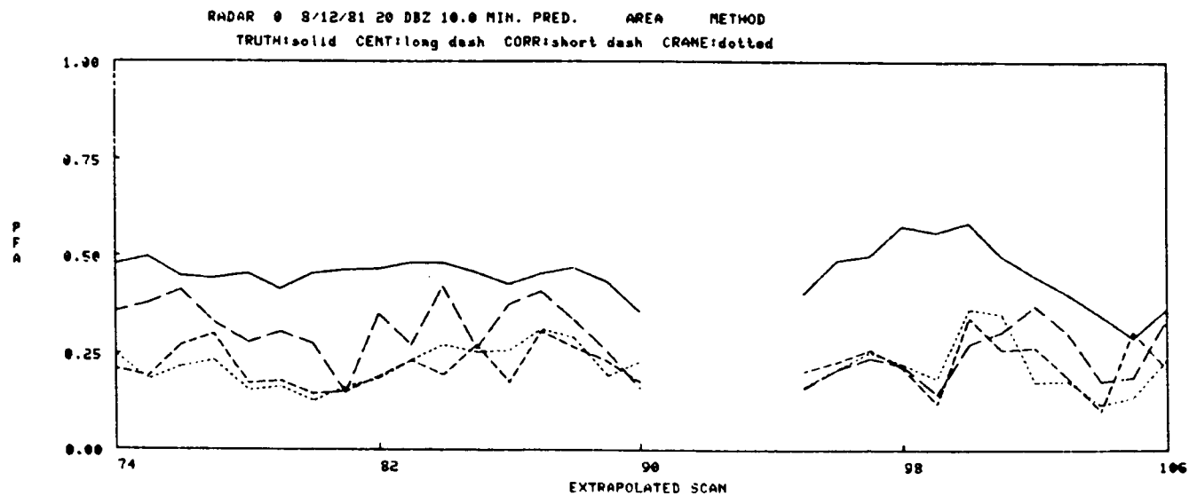
Figure IV-53. 8/12/81 10 min. pred., Area method.
