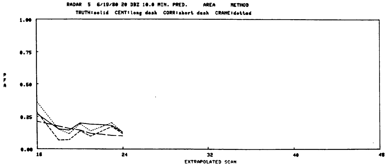
Figure IV-59. 6/19/80 10 min. pred., Area method.
