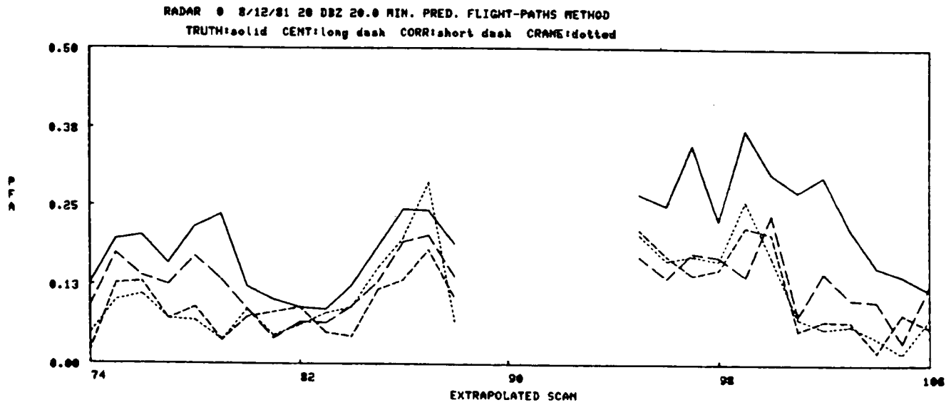
Figure IV-56. 8/12/81 20 min. pred., Flight-paths method.
