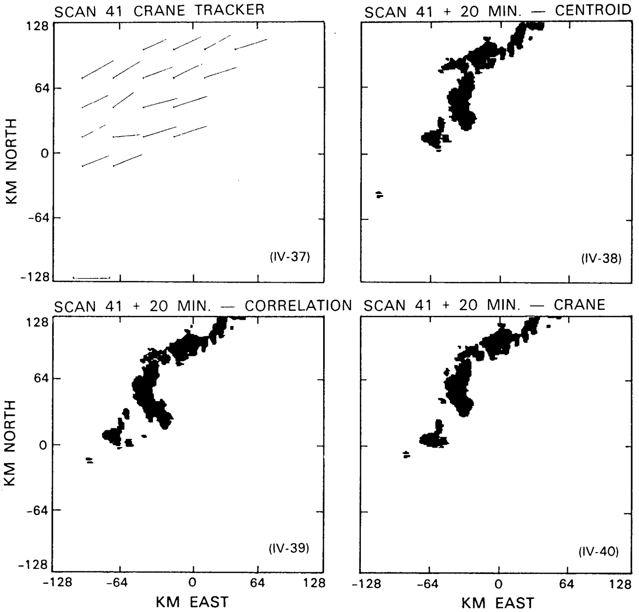
Figure IV-37. to IV-40. NSSL/N 4/13/81 40 dBz.
