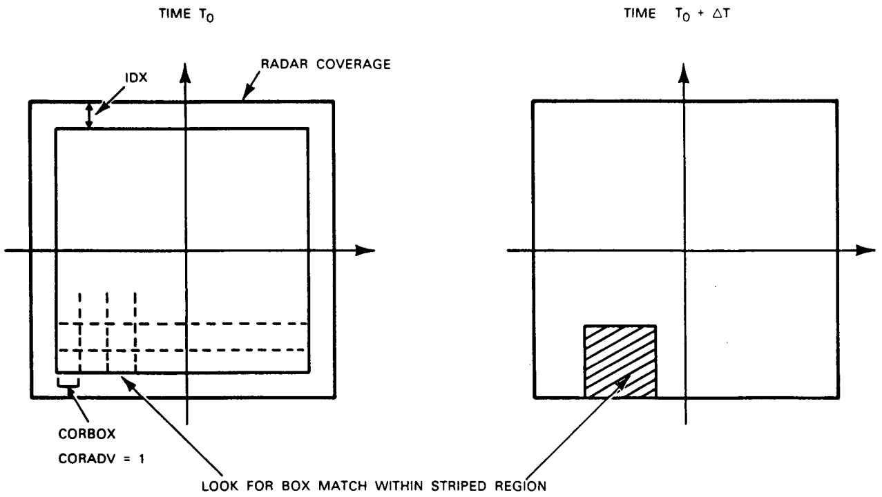
Figure A-2. Cross-correlation, box by box.
