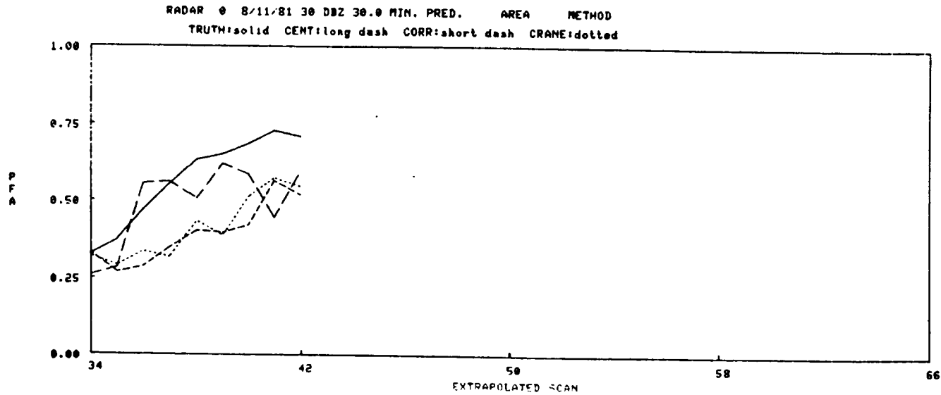
Figure IV-51. 8/11/81 30 min. pred., Area method.
