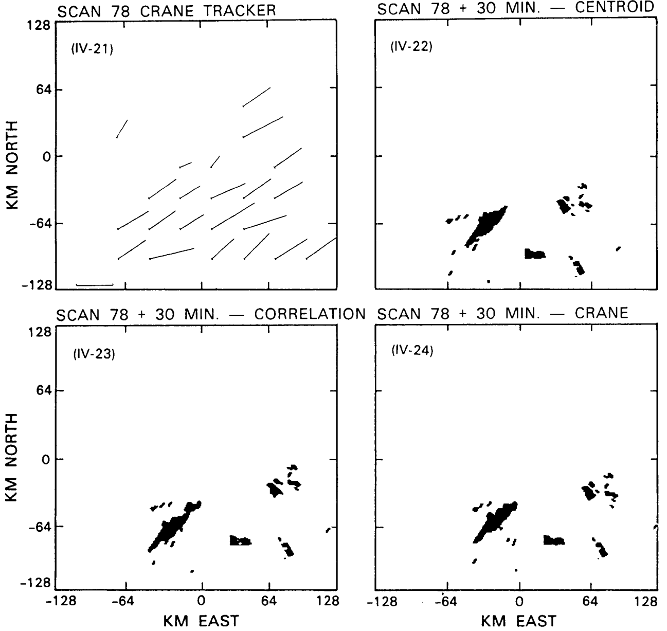
Figure IV-21 to IV-24. M.I.T. 8/12/81 20 dBz.
