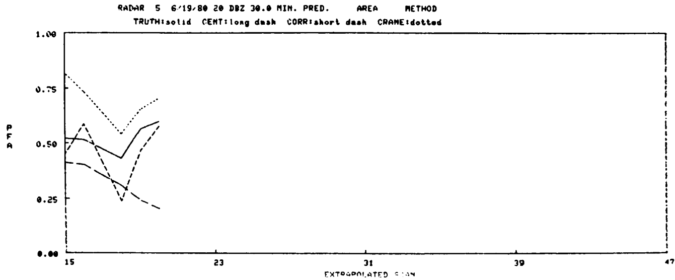
Figure IV-63. 6/19/80 30 min. pred., Area method.
