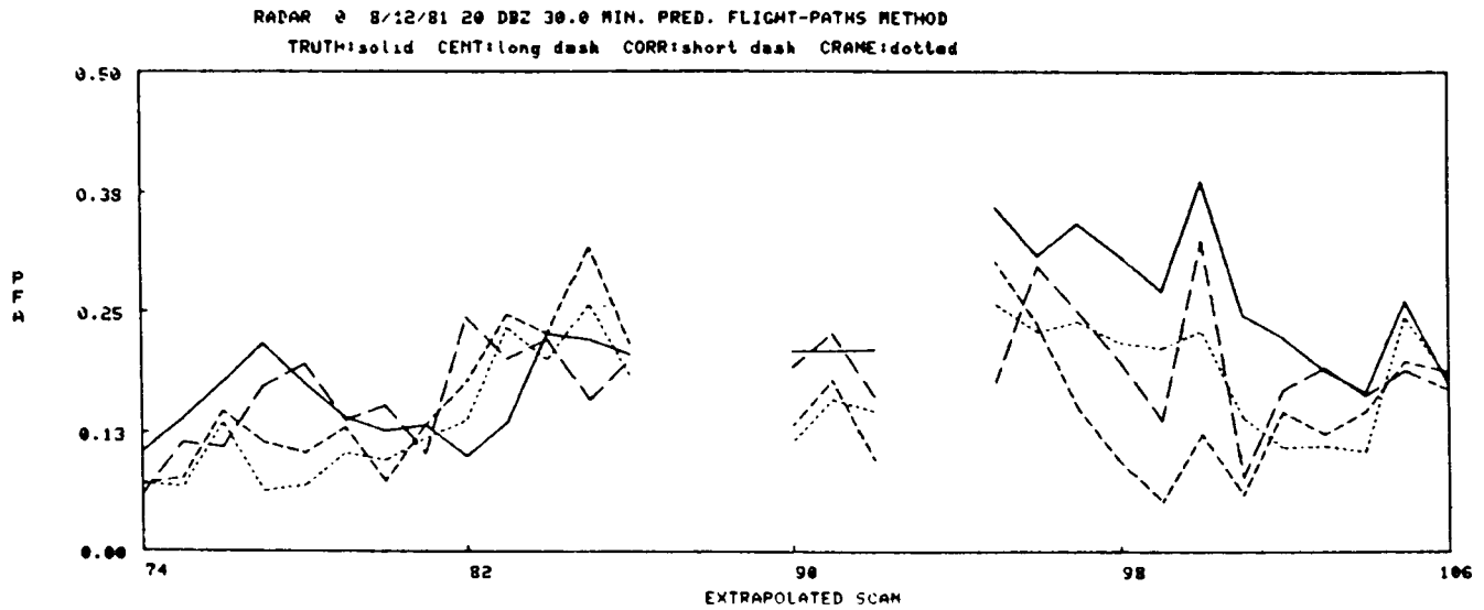
Figure IV-58. 8/12/81 30 min. pred., Flight-paths method.
