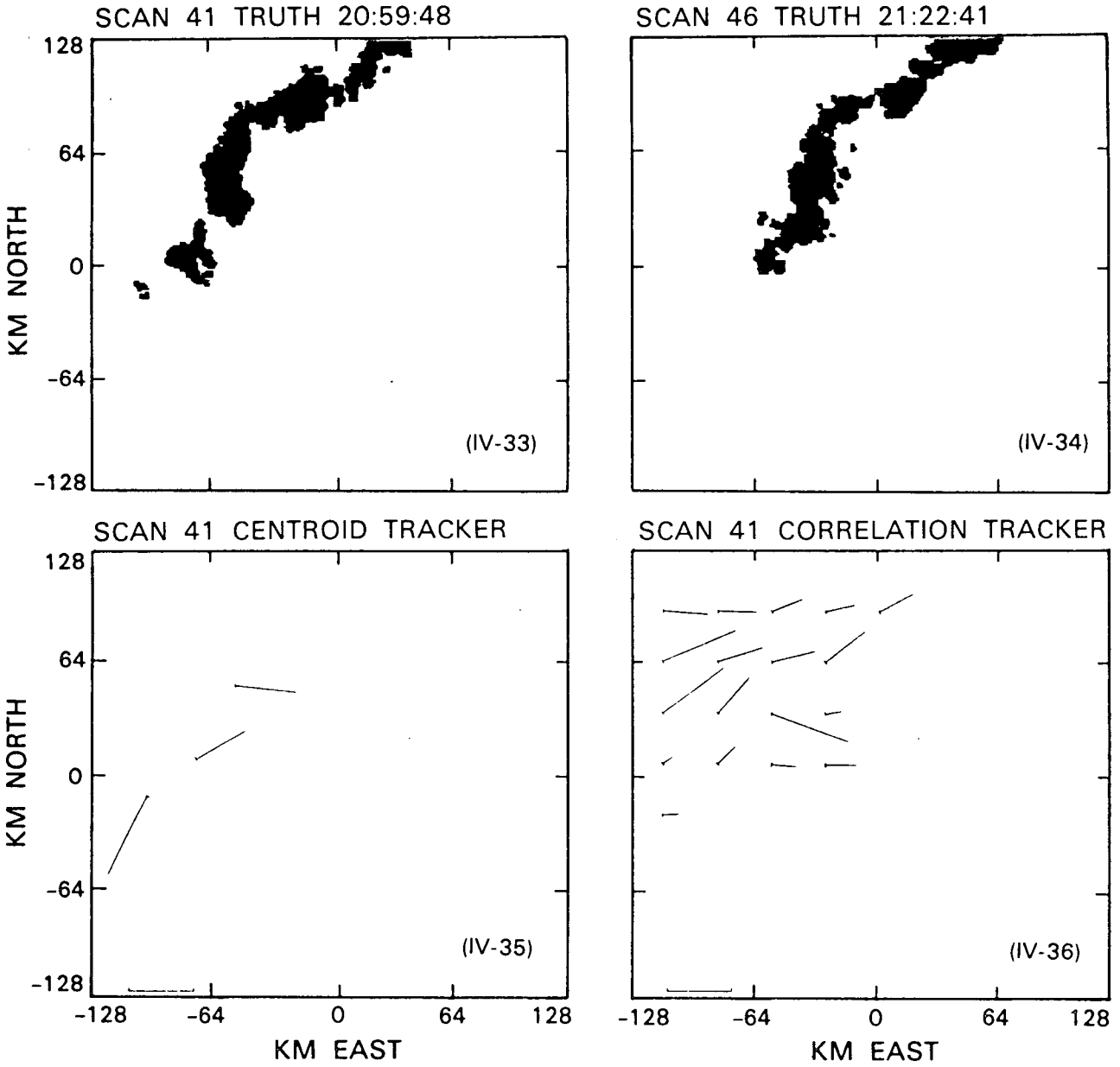
Figure IV-33. to IV-36. NSSL/N 4/13/81 40 dBz.
