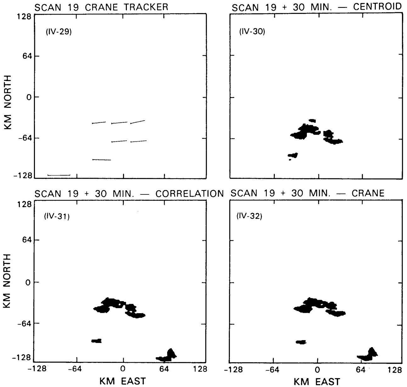
Figure IV-29. to IV-32. NSSL/C 6/19/80 20 dBz.
