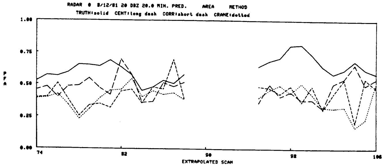
Figure IV-55. 8/12/81 20 min. pred., Area method.
