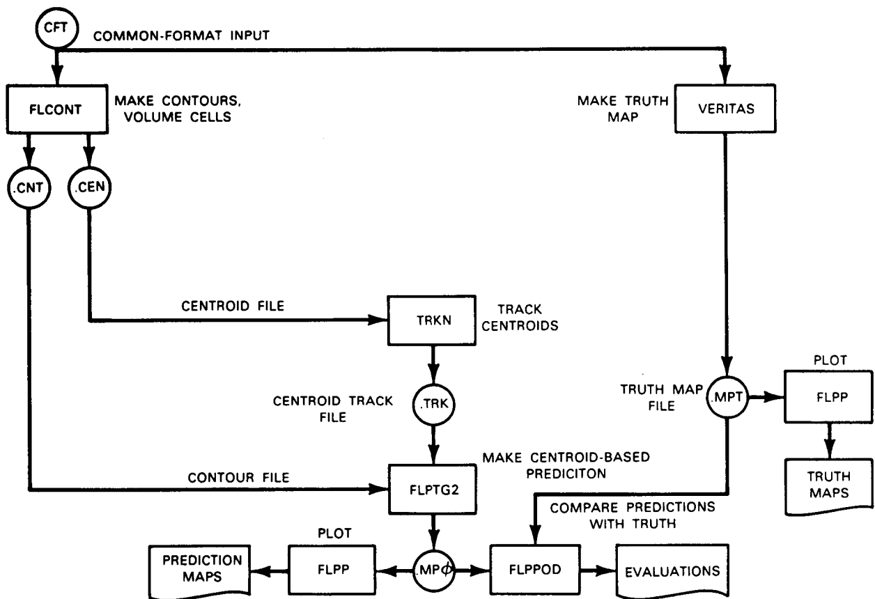
Figure B-1. Centroid tracker flowchart.
