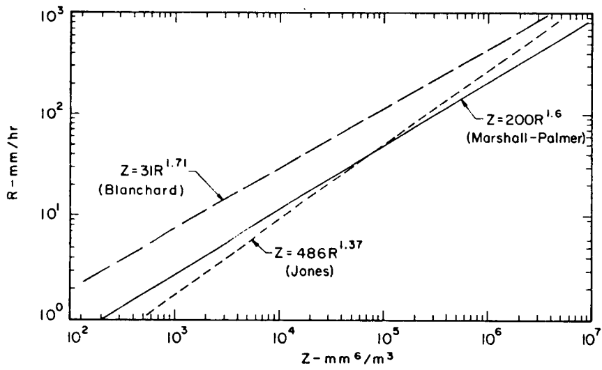
Figure I-1. Plots of various Z-R relationships. (Battan)
