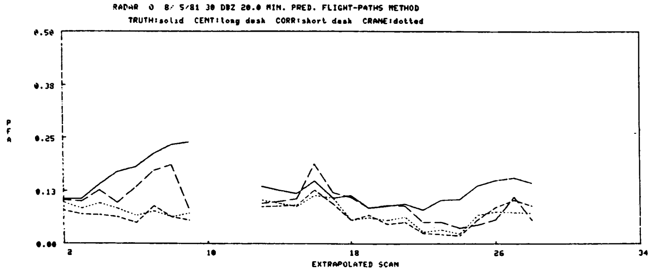
Figure IV-44. 8/5/81 20 min. pred., Flight-paths method.
