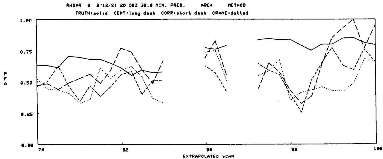
Figure IV-57. 8/12/81 30 min. pred., Area method.
