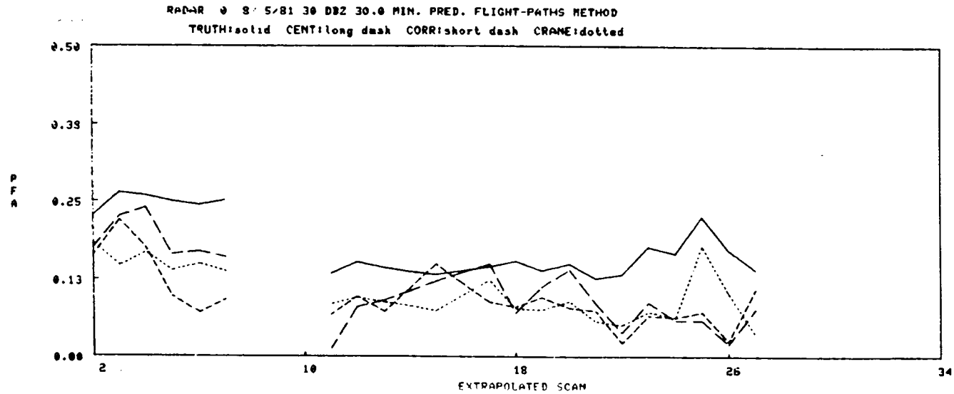
Figure IV-46. 8/5/81 30 min. pred., Flight-paths method.
