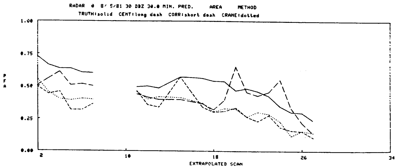
Figure IV-45. 8/5/81 30 min. pred., Area method.
