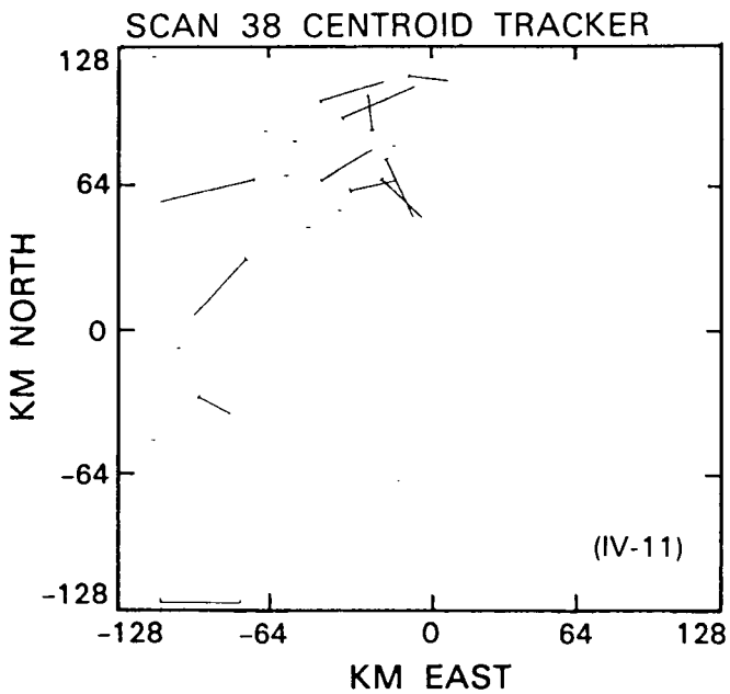
Figure IV-9. to IV-12. M.I.T. 8/11/81 30 dBz.
