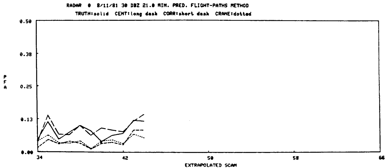
Figure IV.50. 8/11/81 21 min. pred., Flight-paths method.
