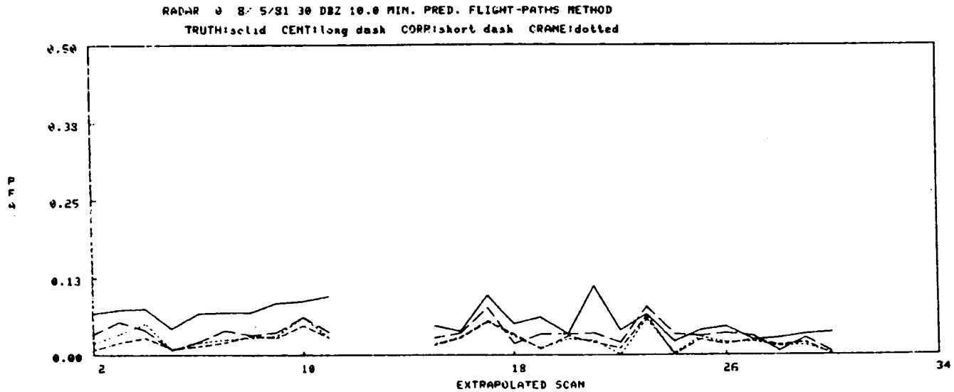
Figure IV-42. 8/5/81 10 min. pred., Flight-paths method.
