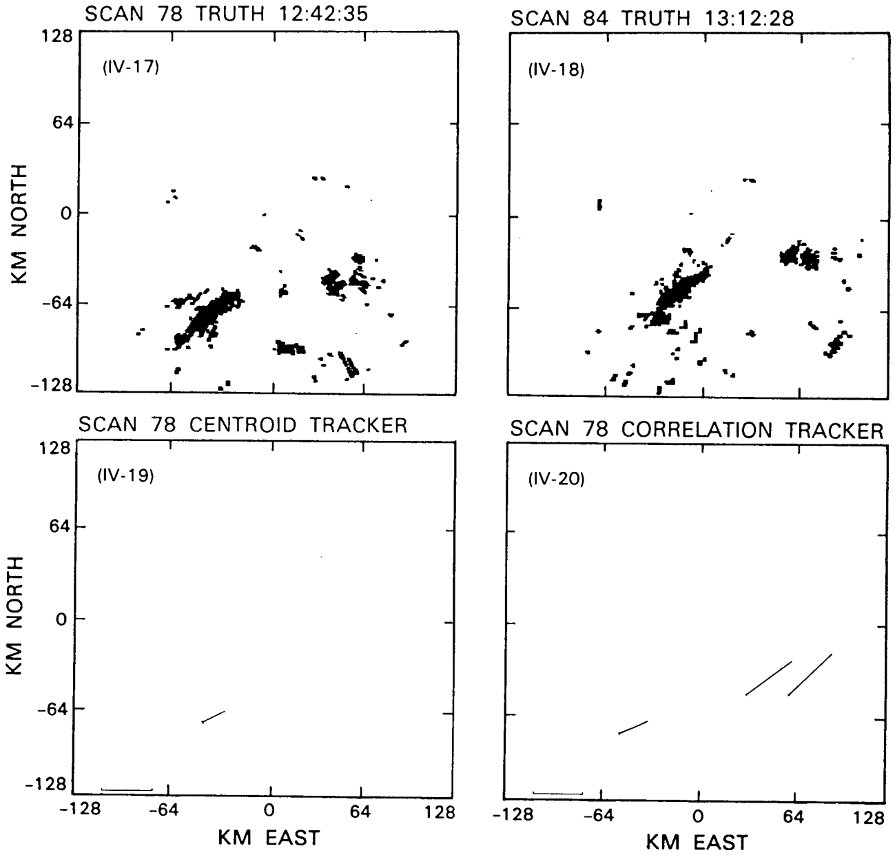
Figure IV-17. to IV-20. M.I.T. 8/12/81 20 dBz.
