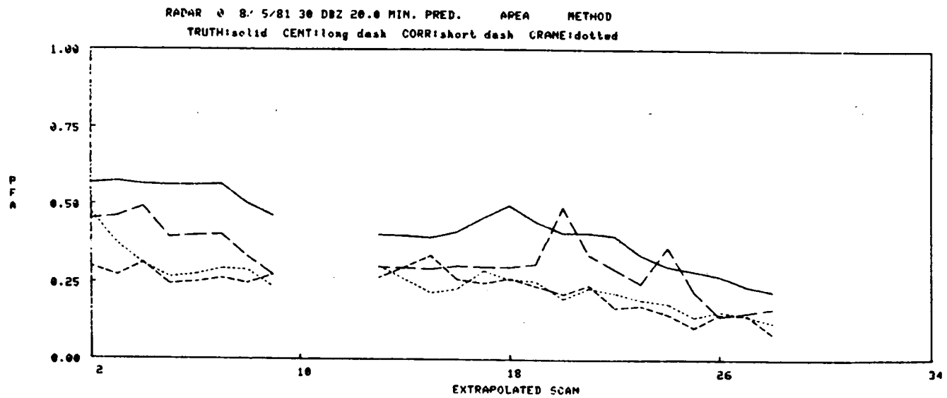
Figure IV-43. 8/5/81 20 min. pred., Area method.
