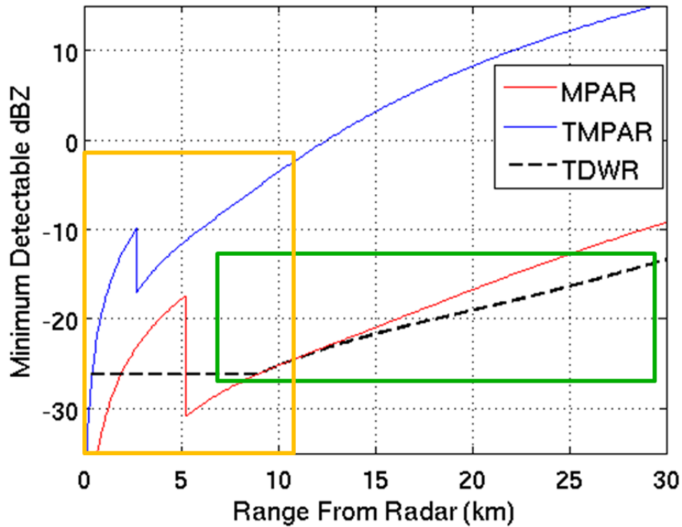
Figure 2-6. Minimum detectable reflectivity for microburst outflows plotted against range for TDWR and notional MPAR and TMAPAR. Volume filling loss is included for a fixed outflow depth of 300 m. The discontinuities in the MPAR and TMAPAR curves reflect the transition from short pulse to long pulse mode. The flattening of the TDWR curve at close range is due to the built-in sensitivity time control (STC) function.
