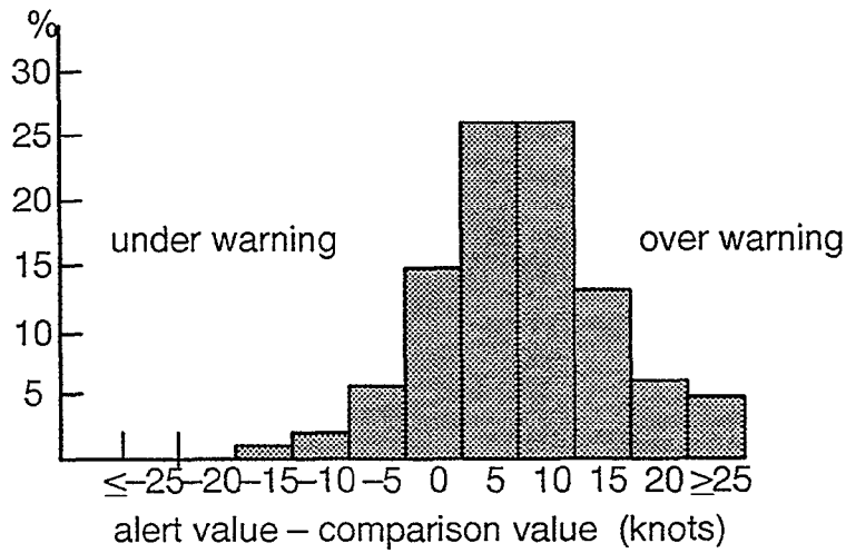
Figure 10. 1991 Union TDWR loss accuracy histogram with flight path shear integration.
