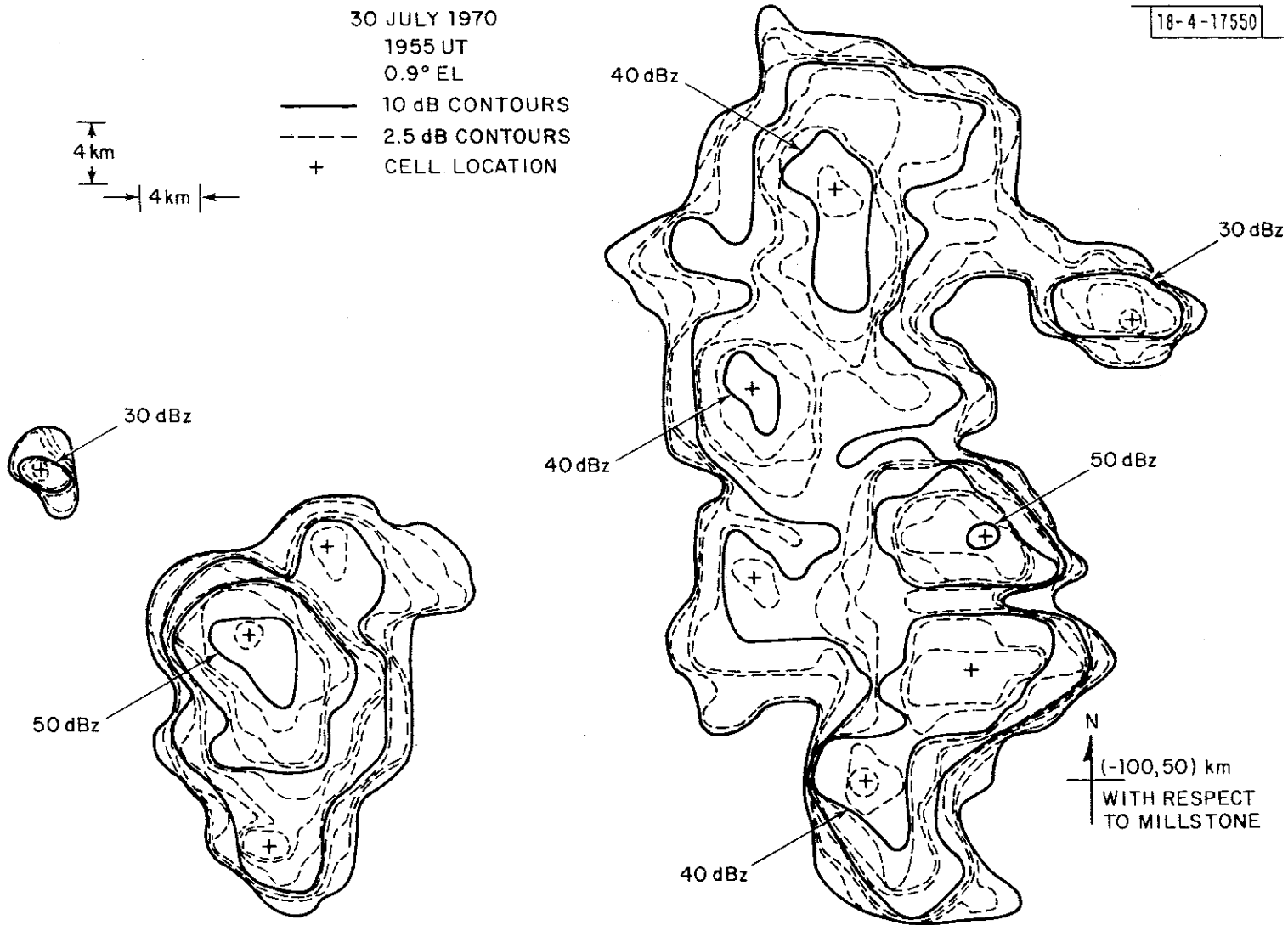
Fig. 3. Radar reflectivity contours and cells detected using a 2.5 dB threshold.
