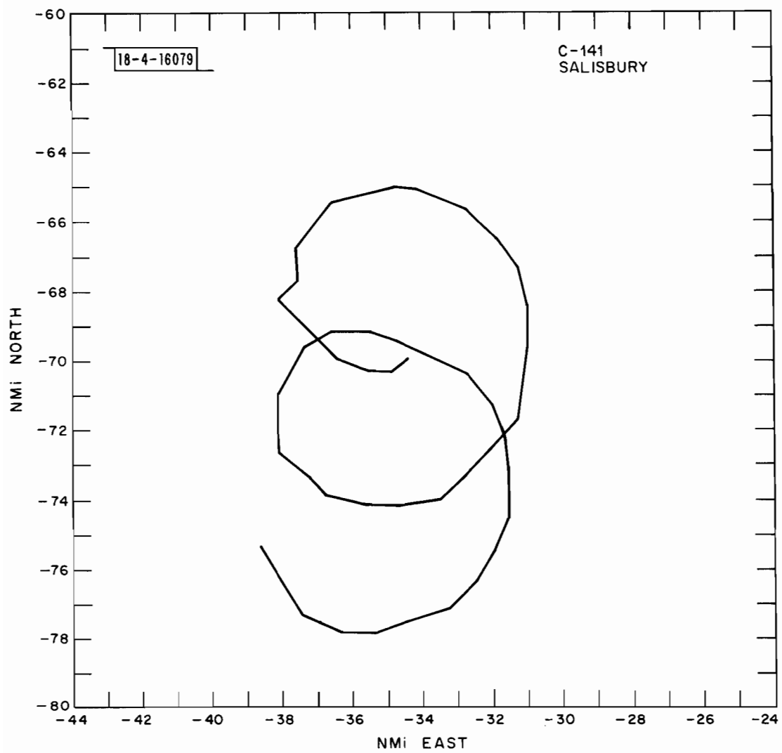
Fig. 39. C-141 in turns at Salisbury with bottom antenna.
