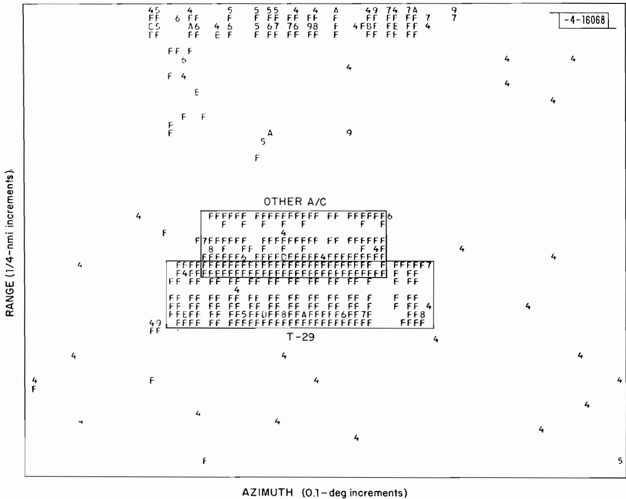
Fig. 18. Potential garbling of replies from the T-29 with those of another aircraft.
