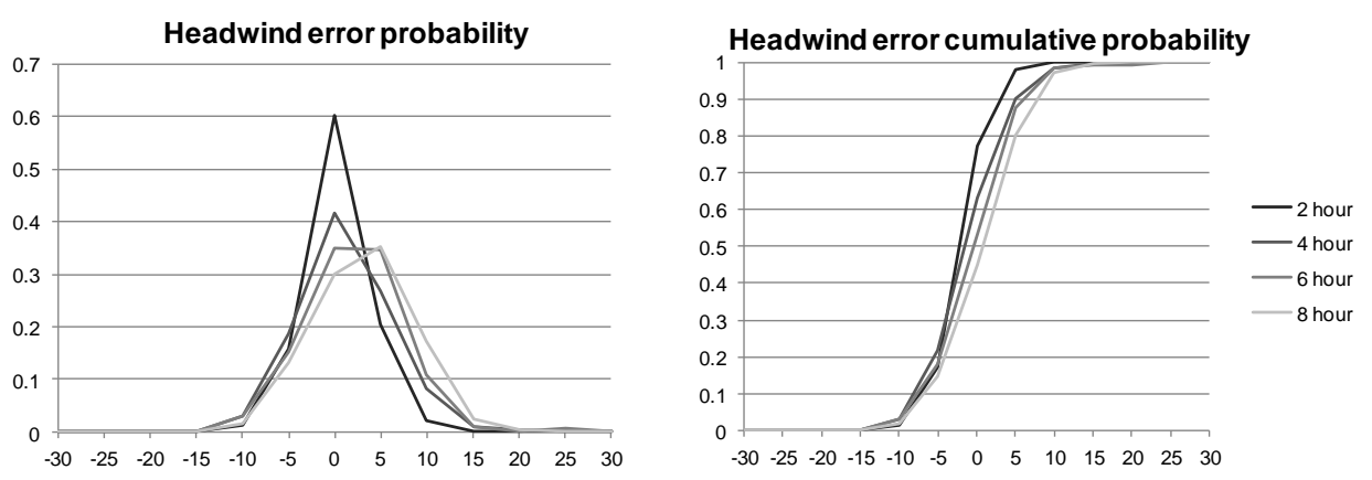
Figure 14. Runway 4 MODEL merge point headwind forecast errors.
