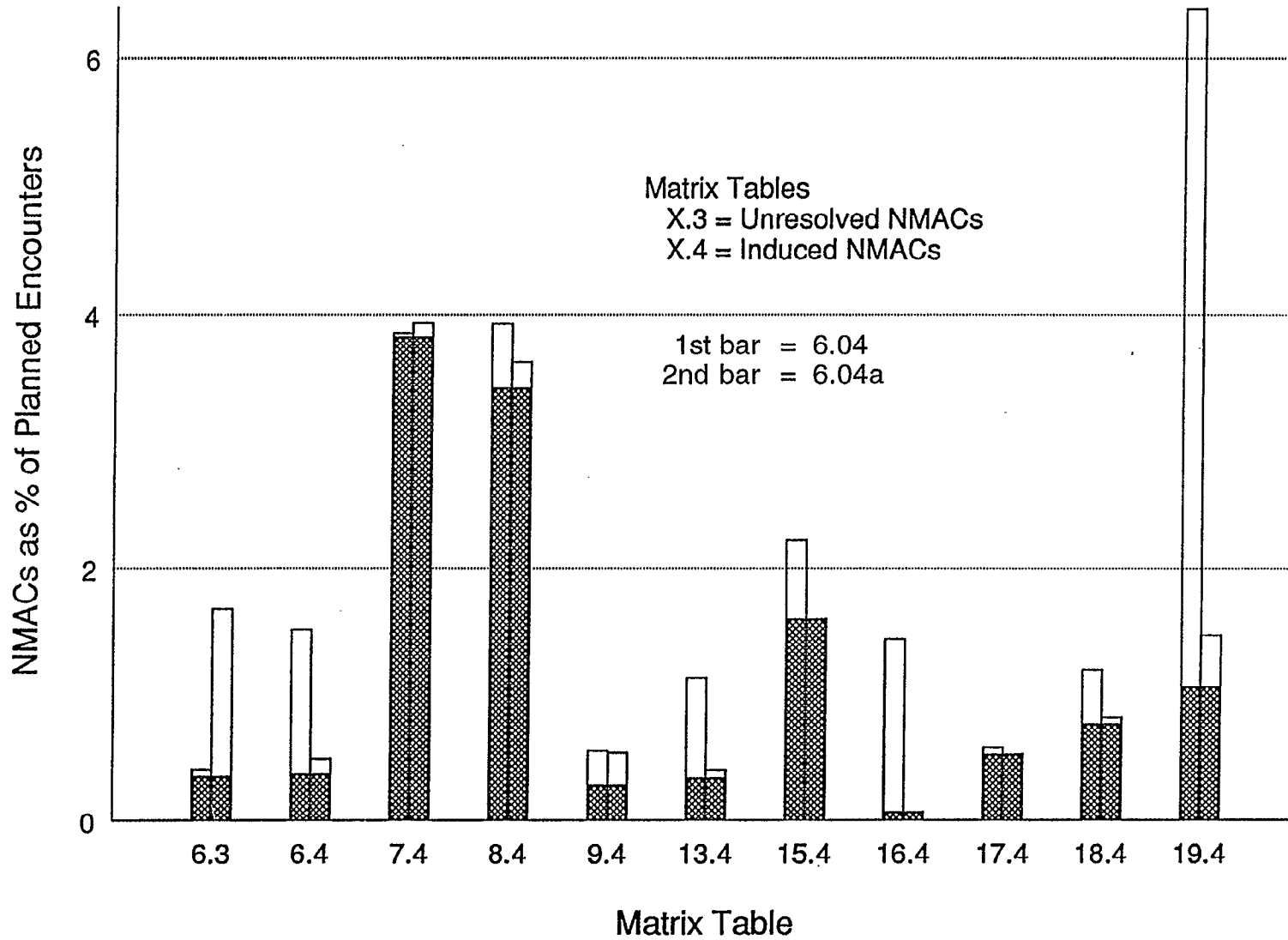
Figure 4-4. Effect of Version 6.04a. Compares number of NMACs (200-ft Separation) - Versions 6.04 and 6.04a, by Matrix Table. Shaded Areas are Common Encounters.
