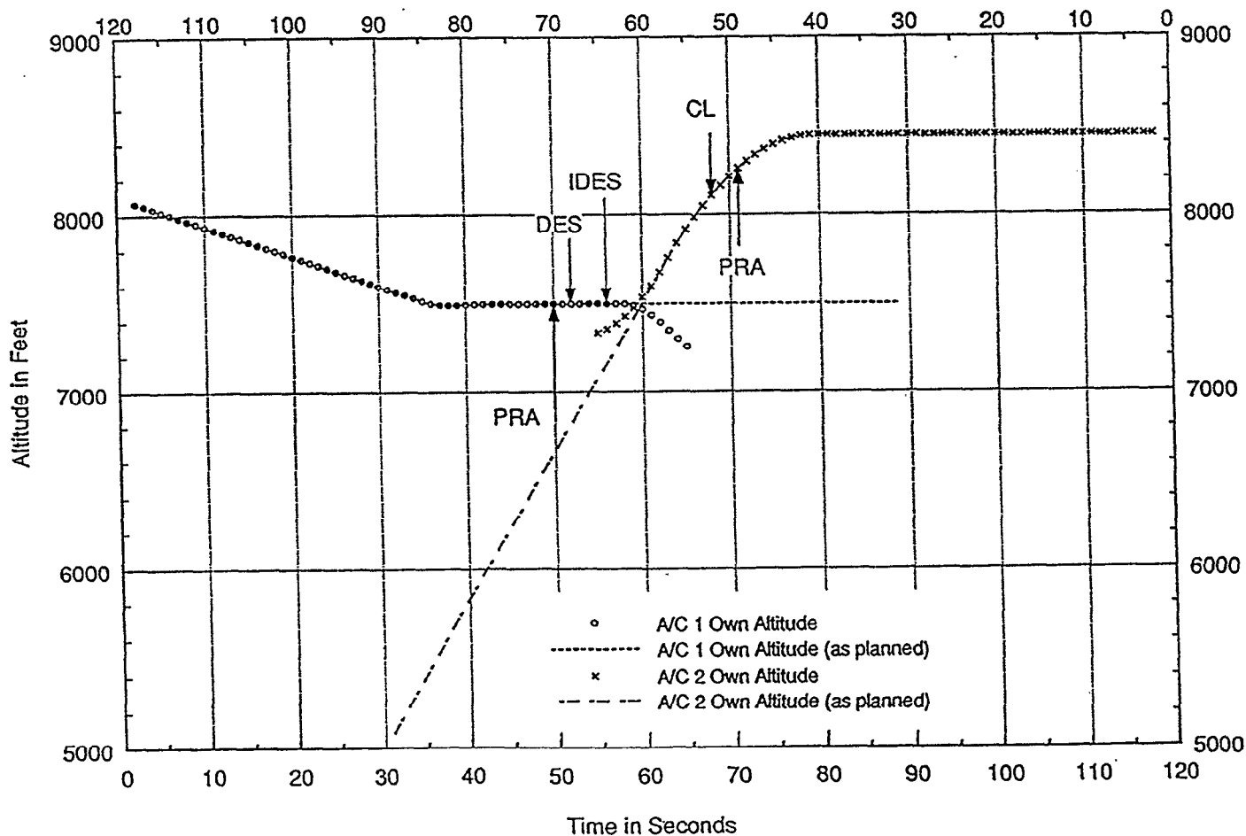
Figure 5-9. Hot-Spot 8.3. Class 8 Unresolved NMACs.
