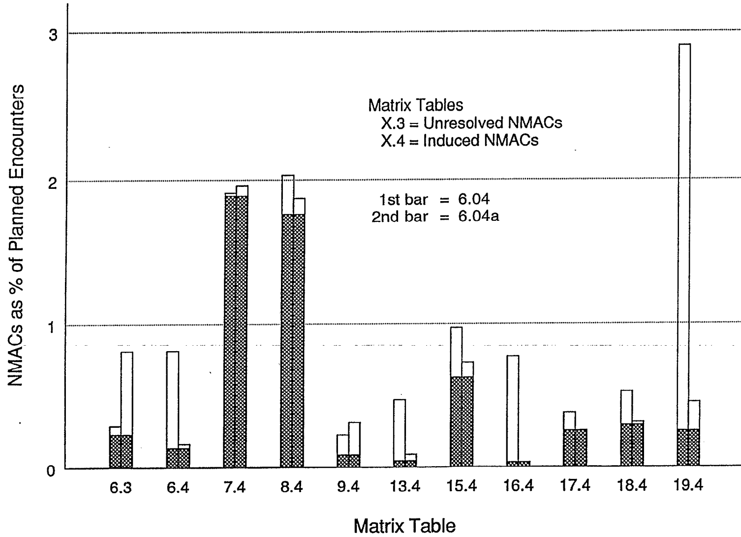
Figure 4-3. Effect of Version 6.04a. Compares number of NMACs - Versions 6.04 and 6.04a, by Matrix Table. Shaded Areas are Common Encounters.
