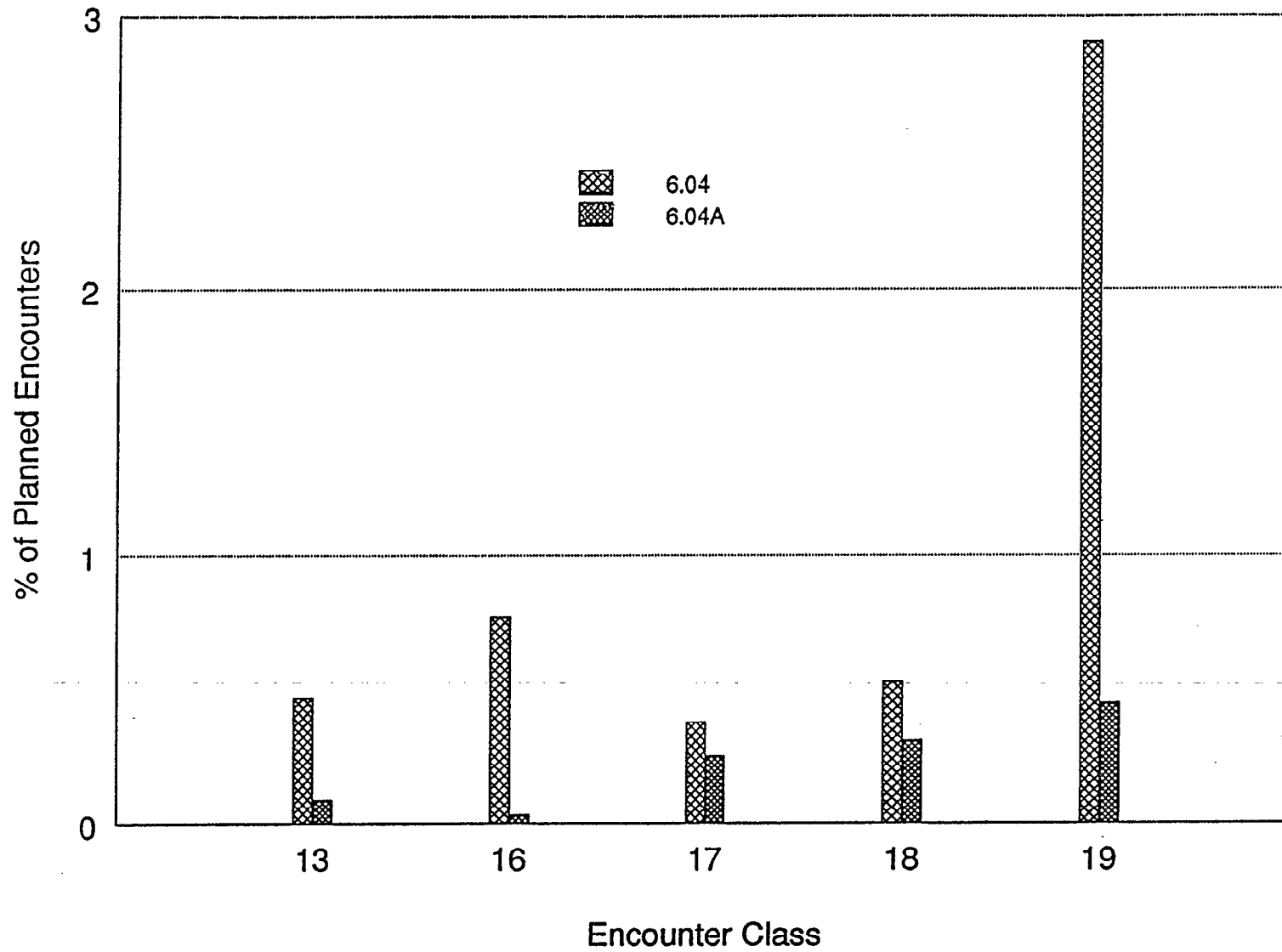
Figure 4-2. Induced NMACs.
