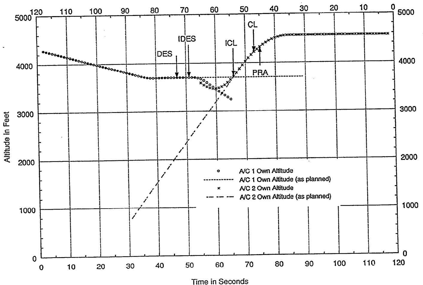
Figure 5-11. Hot-Spot 8.4. Class 8 Induced NMACs.
