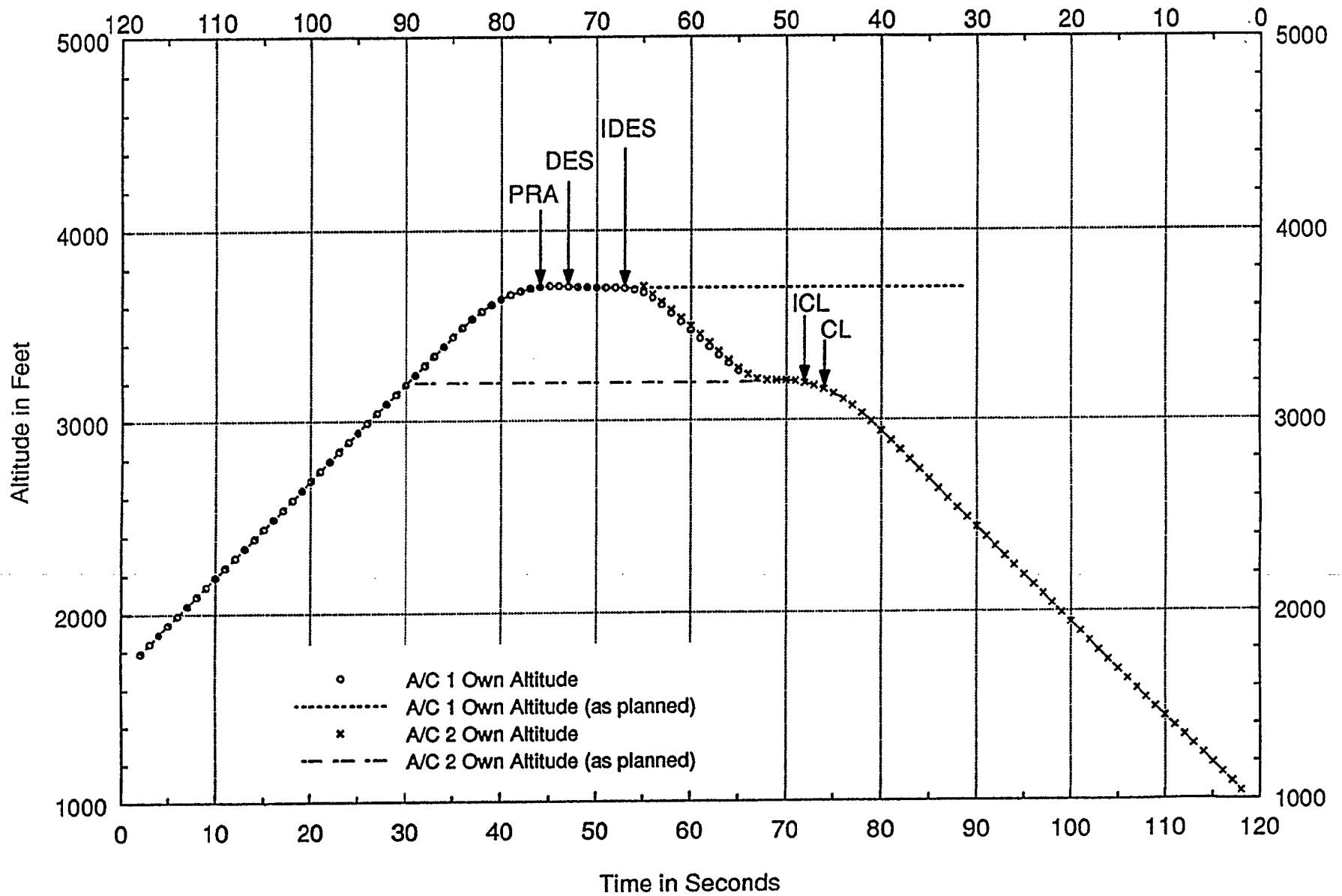
Figure 3-9. Encounter Summary - Aircraft Altitudes. Data file name=LL919YZH.605; REIT Number=2883, SIM Mode: 2165144 (Source: LL Composite FTEG Run, Dated 07/29/94)
