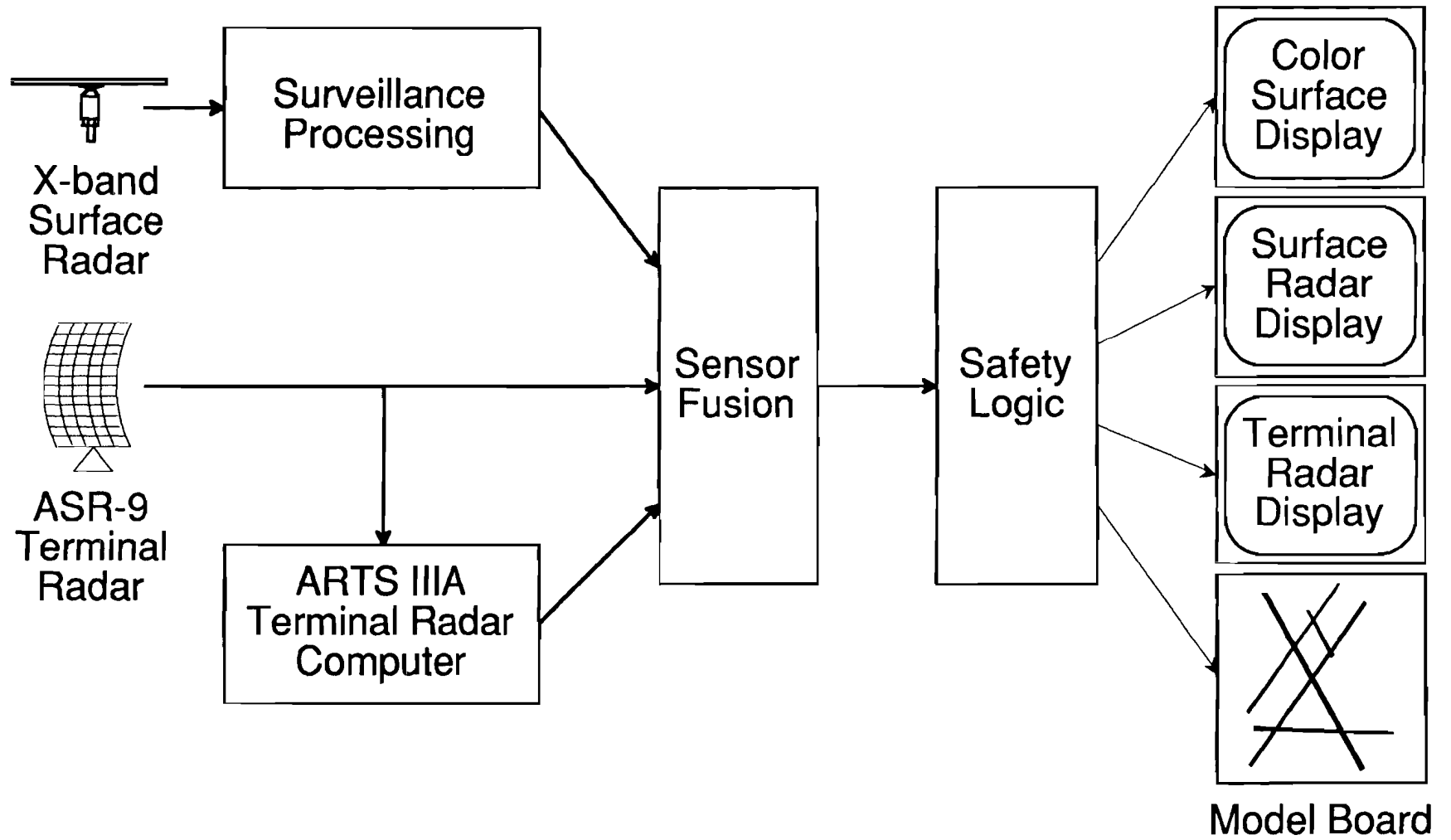
Figure 1-8. RSLs Demonstration System architecture overview.
