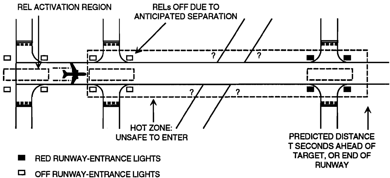
Figure 6-8. Hot zone and REL activation regions for runway-entrance lights.
