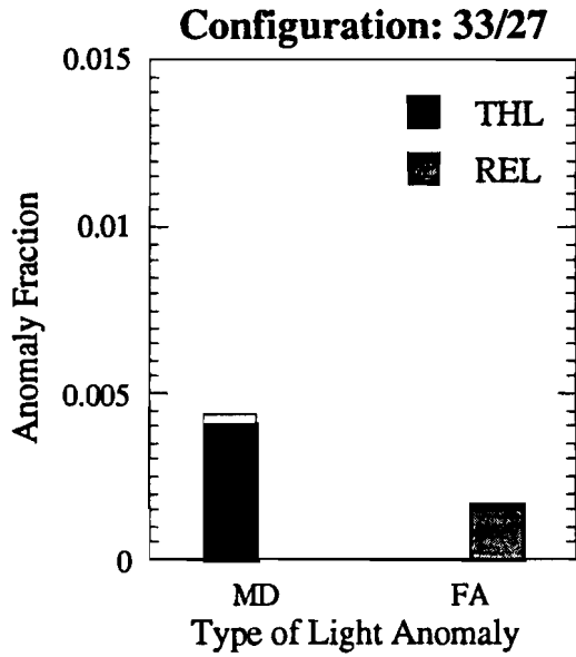
Figure 9-3. Anomaly fraction for false alarms and missed detections in the four configurations.
