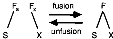
Figure 5-4. Fusion and unfusion processes.
