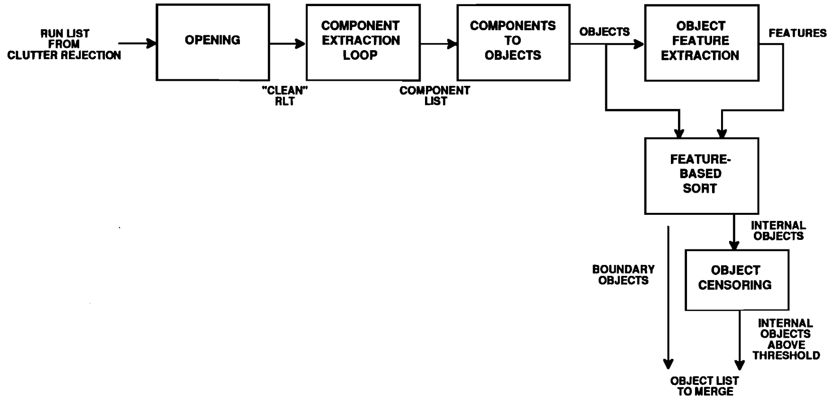
Figure 7-3-6. Architecture of connected component process.
