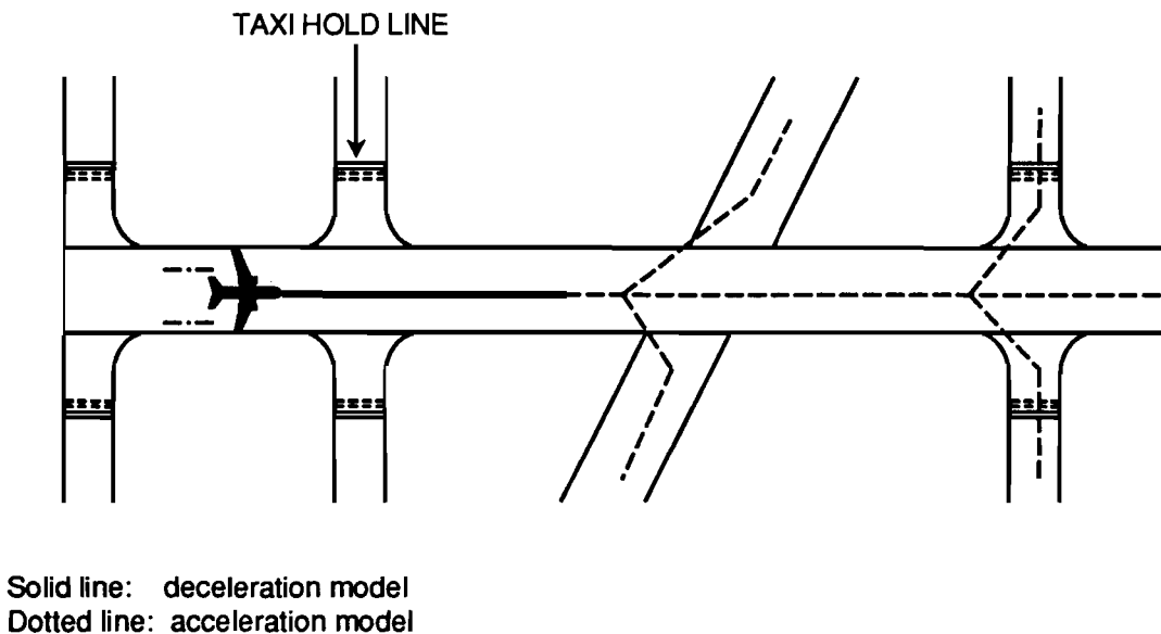
Figure 6-5. Path-prediction trees.
