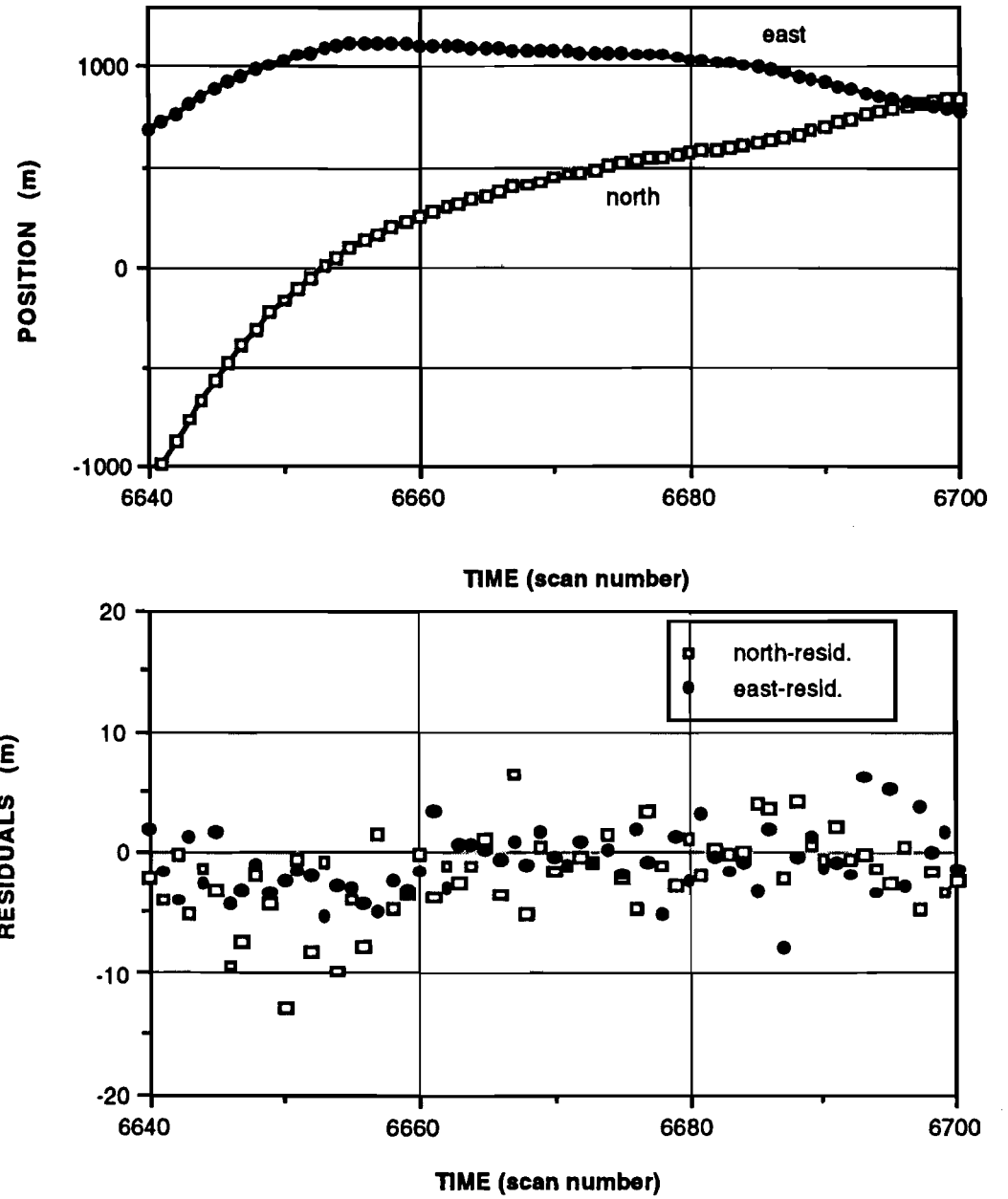
Figure 8-3. Analysis of jitter in track 113142.
