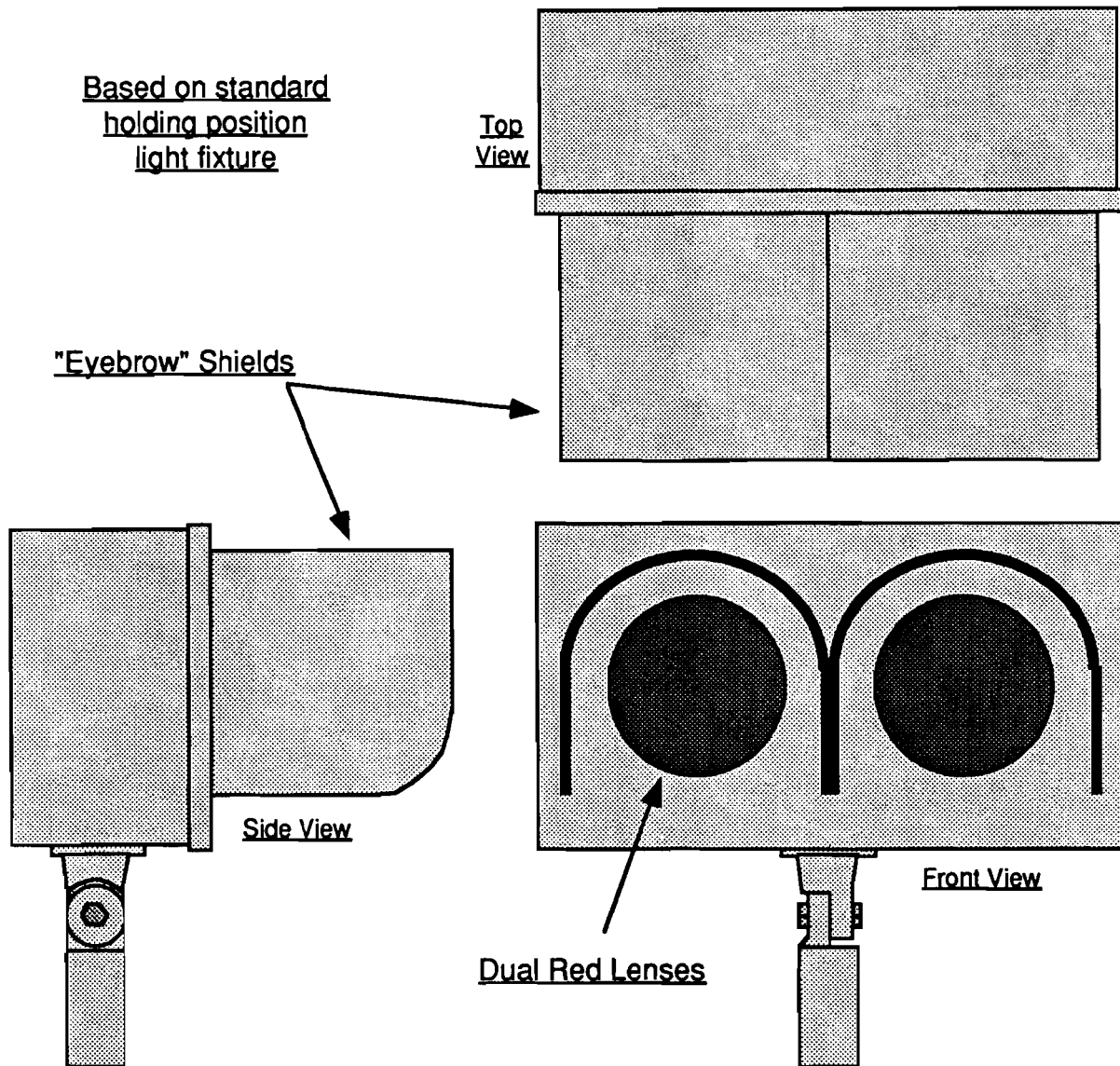
Figure 1-4. RSL status light fixture.
