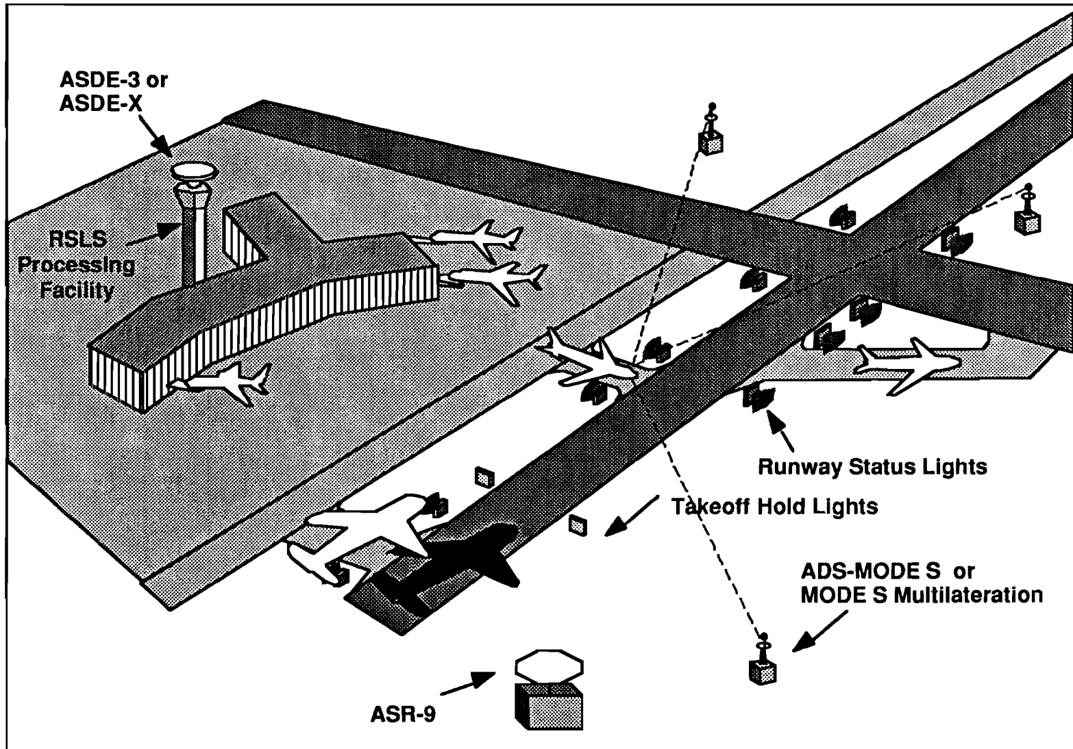
Figure 1-1. RLS system concept.
