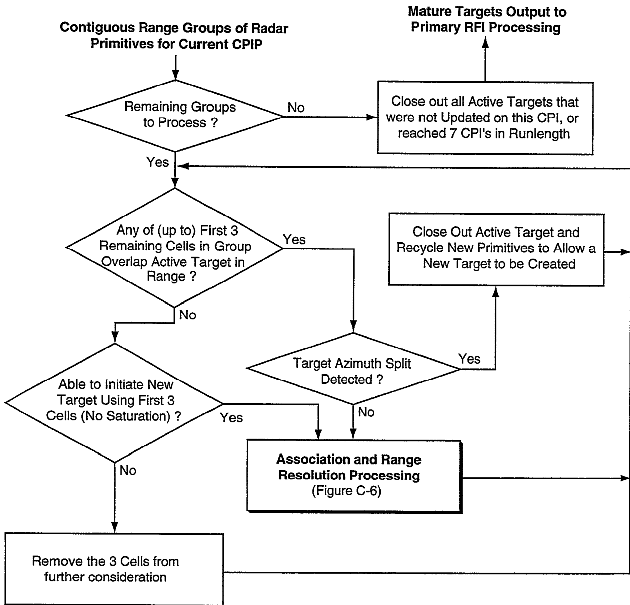
Figure C-5. Target correlation.
