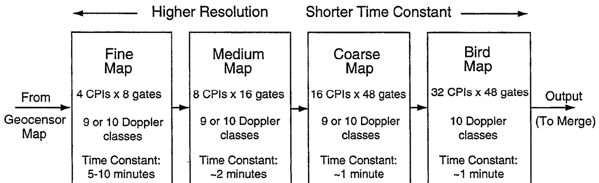
Figure 5-5. 9PAC adaptive map thresholding stages.
