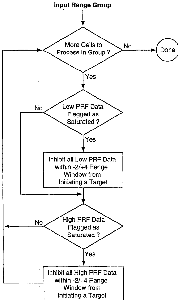
Figure C-4. Saturation preprocessing.
