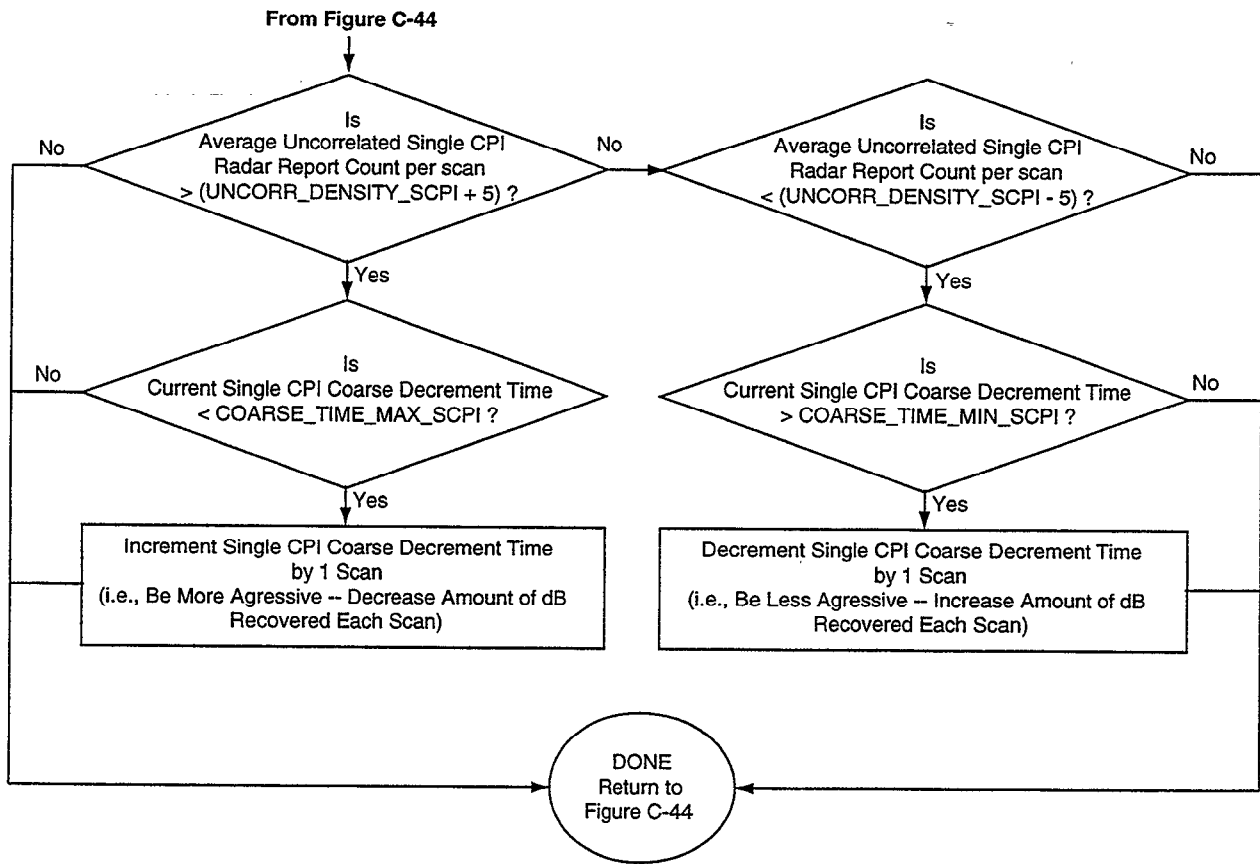
Figure C-51. Single CPI coarse map single scan decrement determination.
