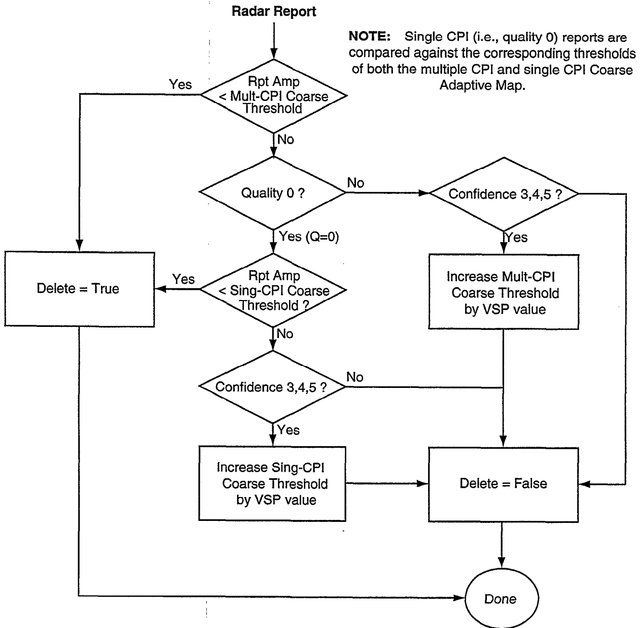
Figure C-18. Coarse adaptive map thresholding.
