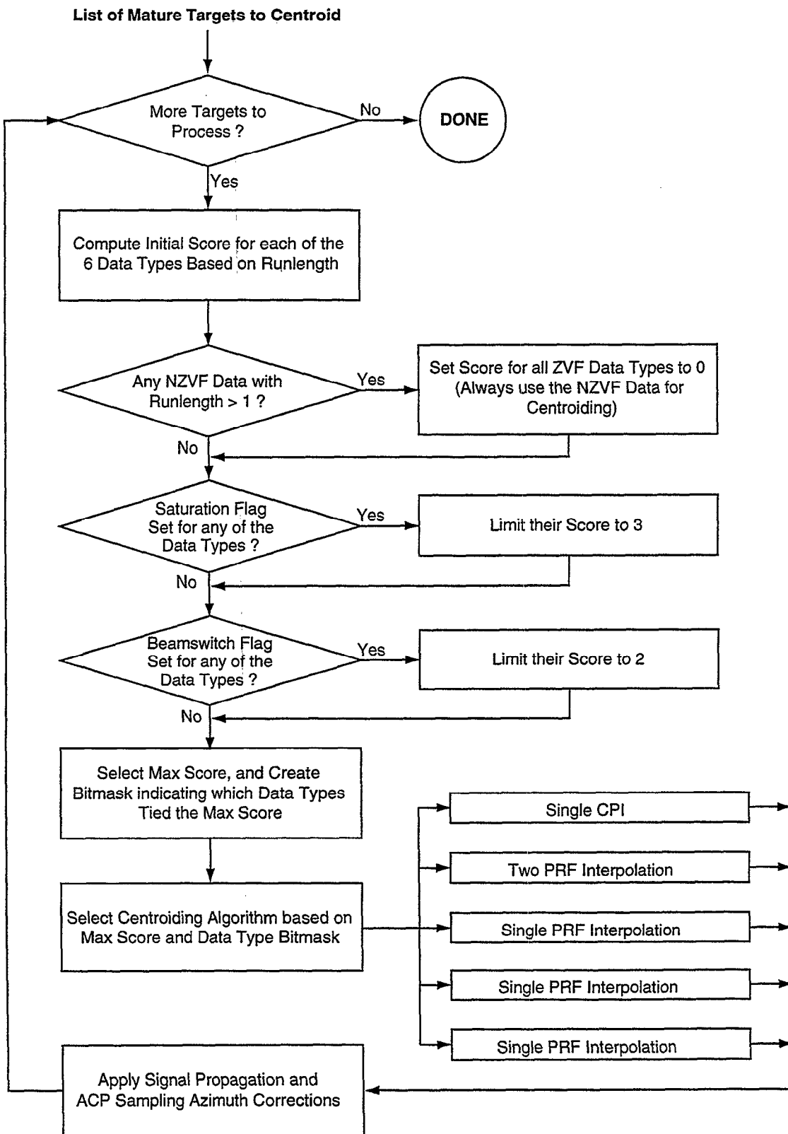
Figure C-8. Azimuth centroiding.
