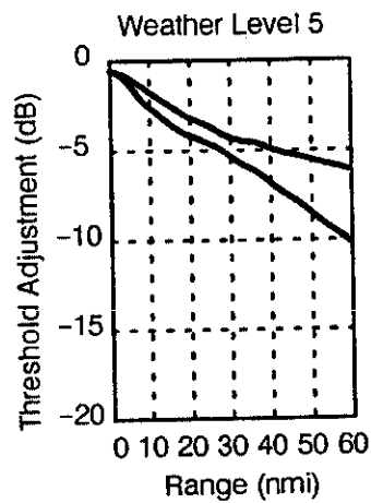
Figure 16. Threshold adjustments necessary to minimize the report error of the ensemble of profiles comprising each weather level in the Boston data set. Upper curve is for the low beam, lower curve for the high beam.
