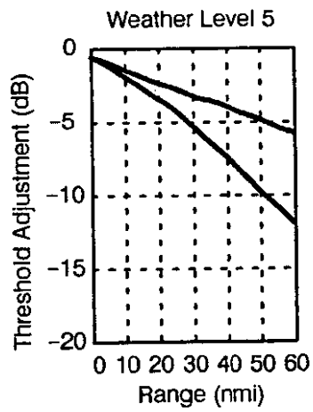
Figure 17. Threshold adjustments as in Figure 16, but for the Huntsville data set.
