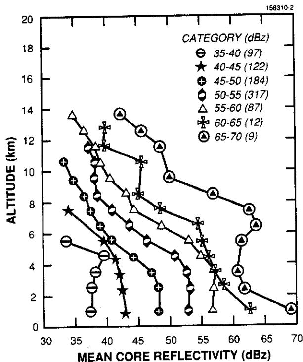
Figure 5. Profiles of mean core reflectivity for various categories of rainshowers. Number of cells in each category is shown in parentheses. (From Konrad, 1978.)
