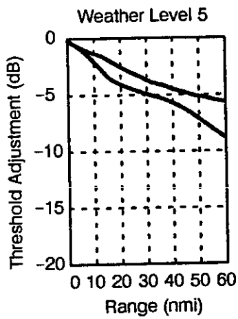
Figure 19. Threshold adjustments as in Figure 16, but for the Denver data set.
