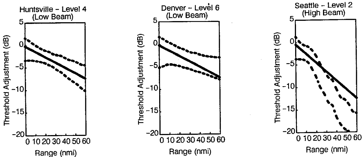
Figure 21. Relative placement of U.S. threshold adjustment curve (solid) with respect to upper and lower rms error bounds of sitellevel specific adjustment curves (dashed).
