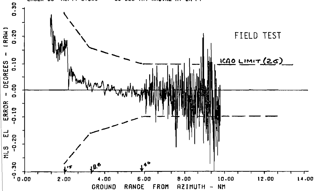
Fig. 4-8 Comparison of DMLS simulation and flight test on -38^\circ radial at 2000 feet at JFK airport.
