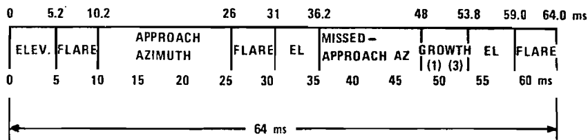
(b) Subsequence #1
