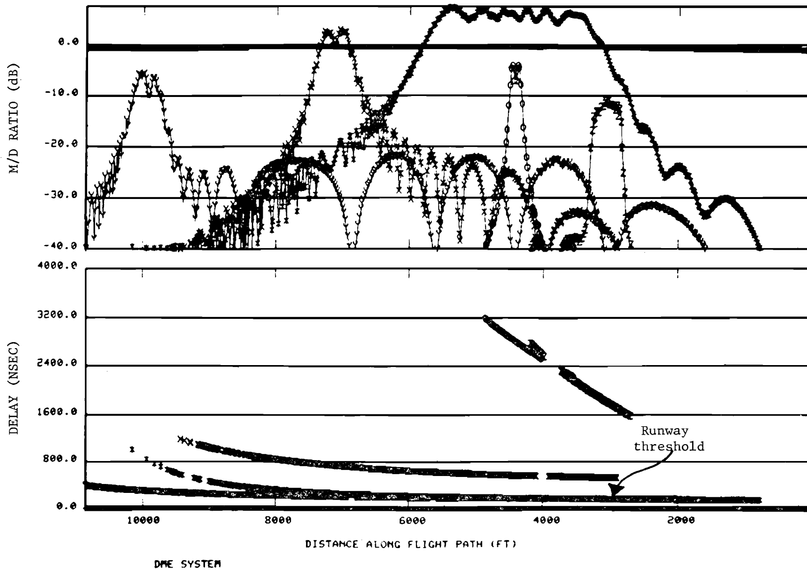
Fig. 4-16. Computed multipath characteristics for Lambert - St. Louis scenario.
