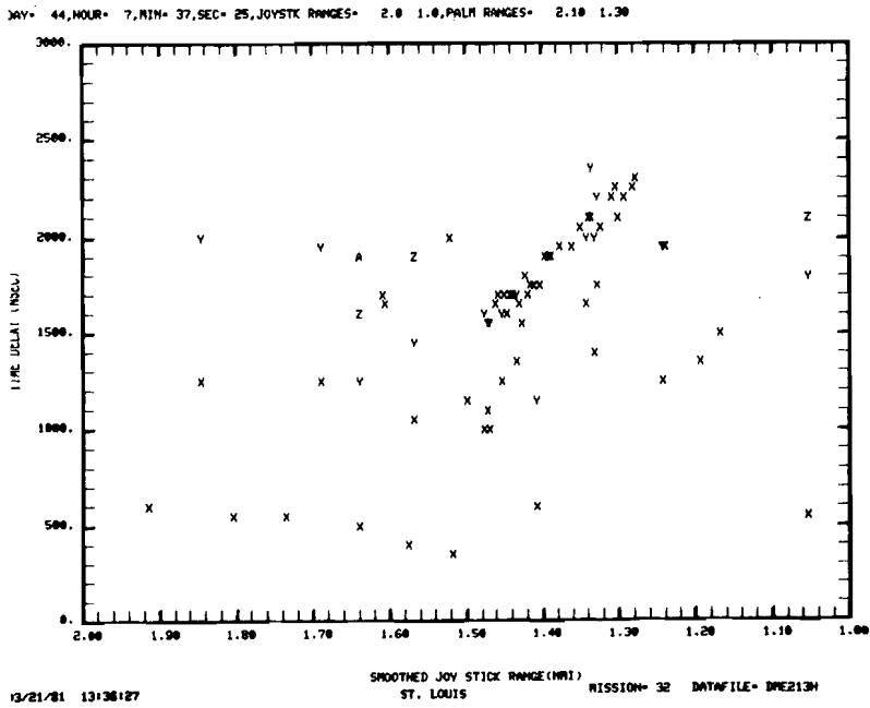
Fig. 4-10b. Data summary for St. Louis's approach with 25 ft. threshold height.
