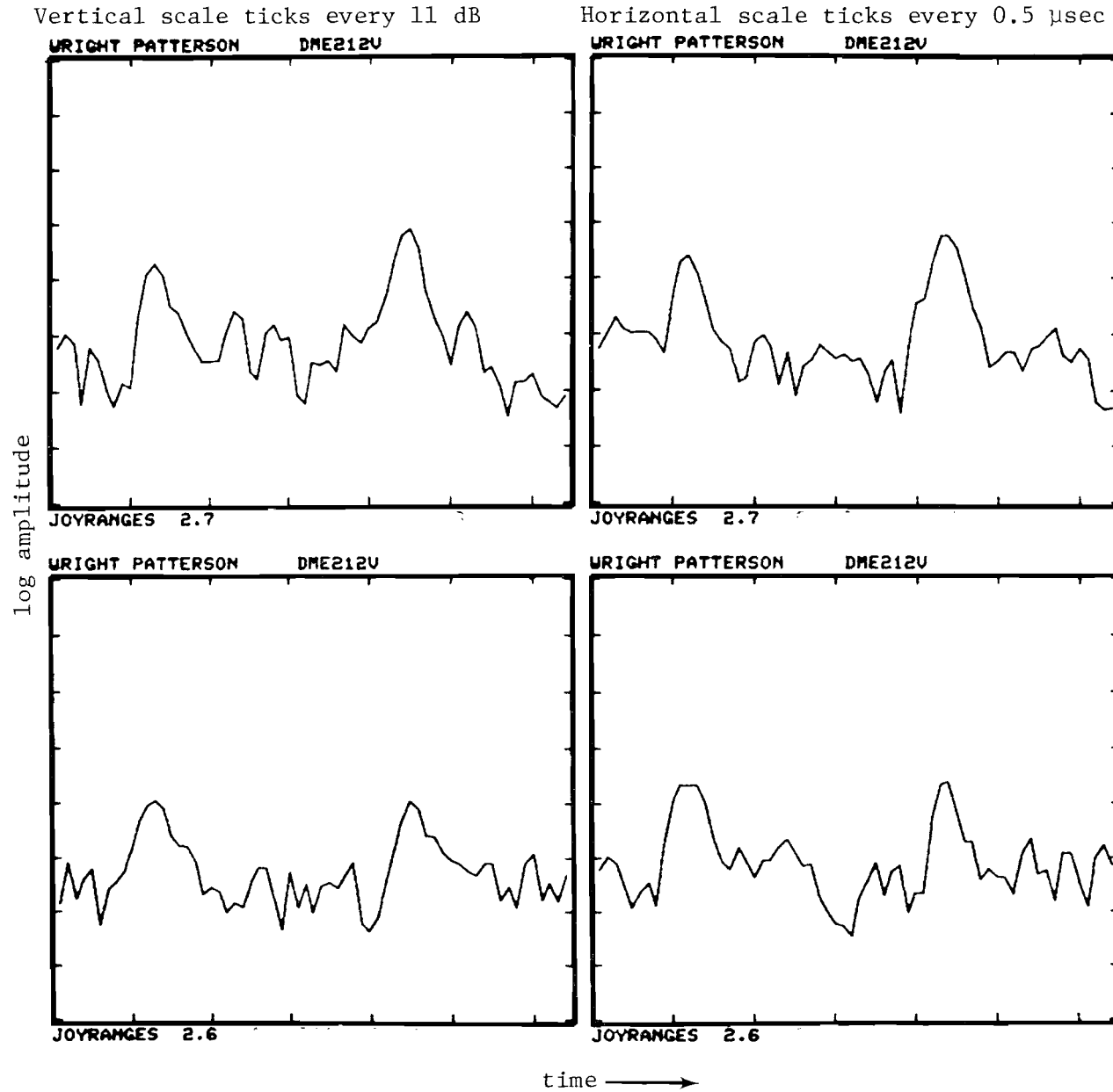
Fig. 6-10. WPAFB waveforms near threshold on flight profile 2.
