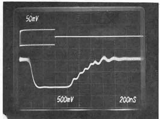
Fig. 2-5d. Gated IF burst response of IF filter and log AMP stage. Upper trace is gated 60 MHz input. Lower trace is filter/log AMP detected video output.
