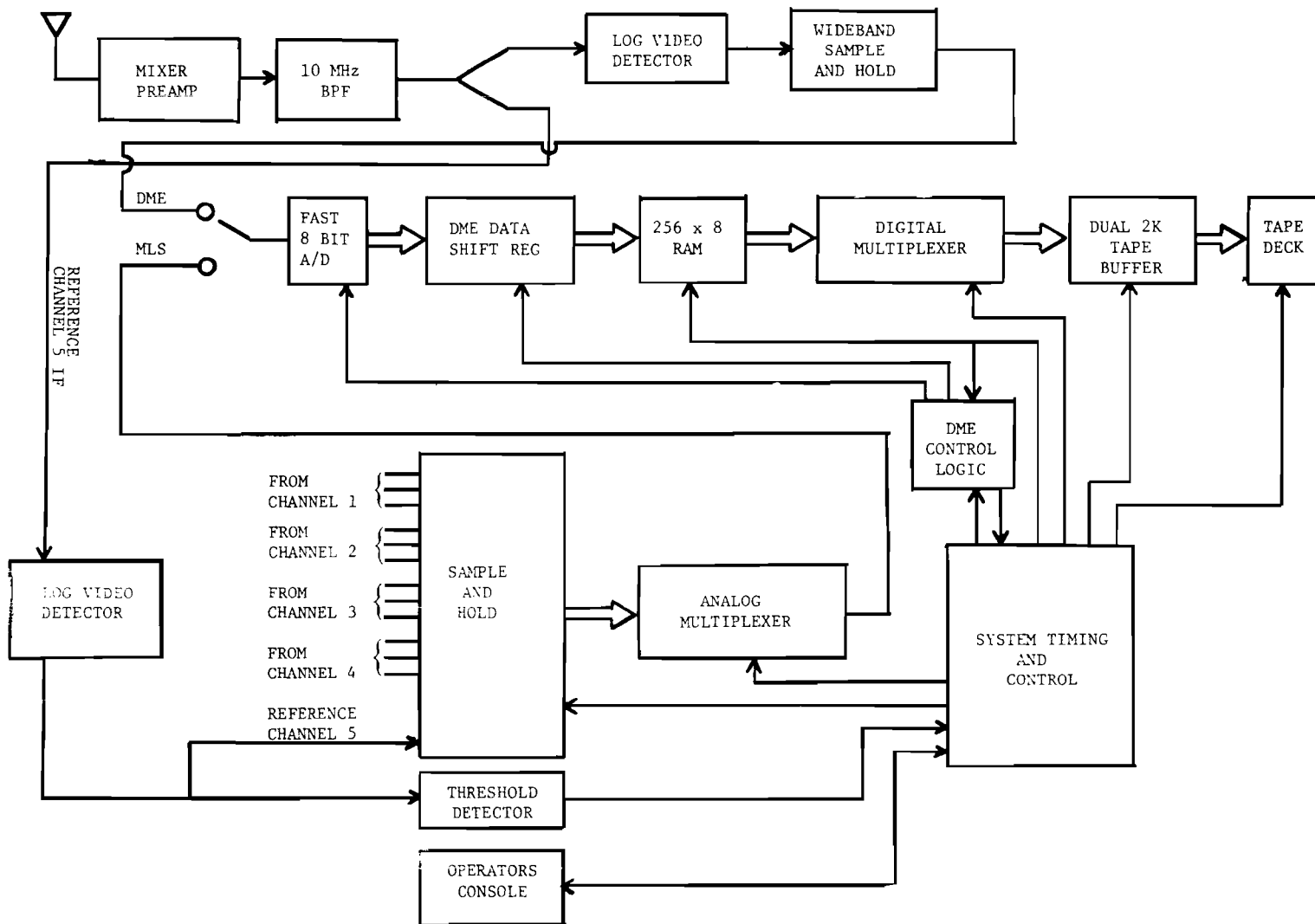
Fig. 2-4. Receiver/processor block diagram.
