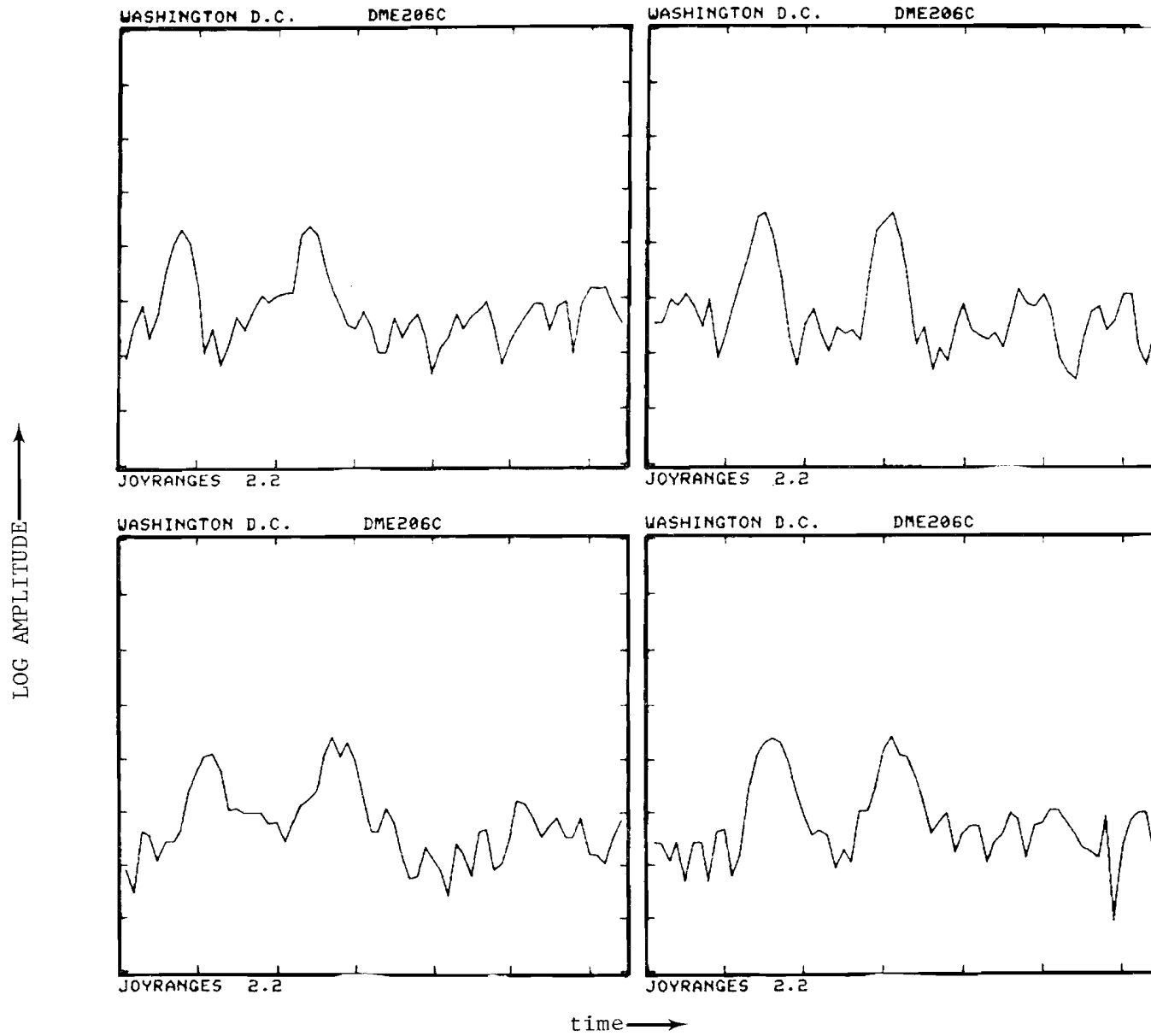
Fig. 8-8. DCA waveforms on 6^\circ approach at 1.4 nmi from threshold.
