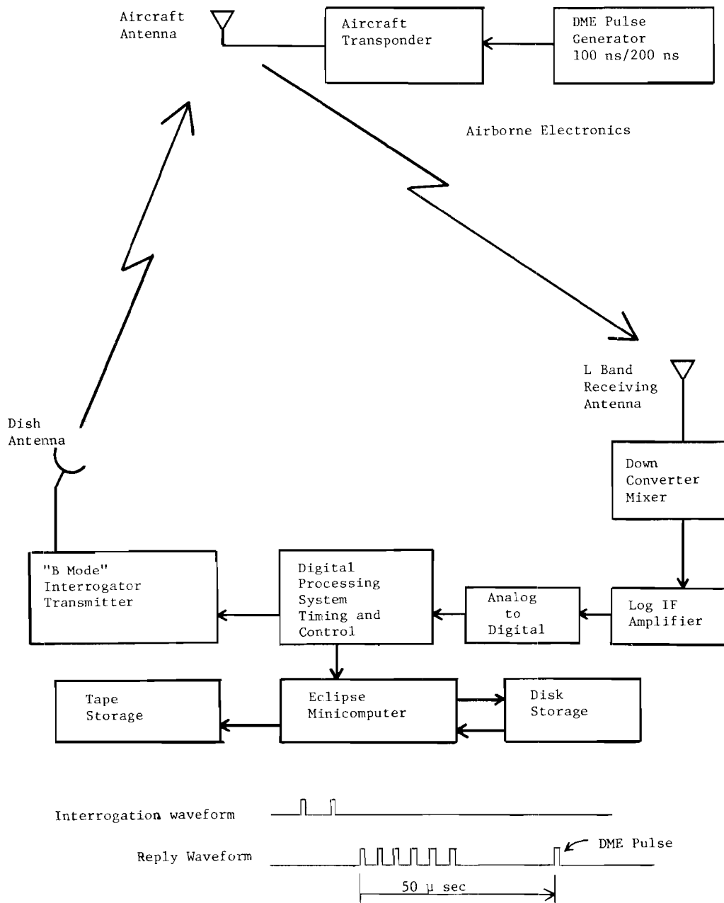
Fig. 2-1. DME hardware block diagram.
