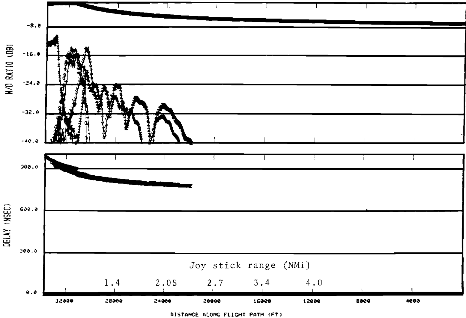
Fig. 8-17. Computed M/D level for 6° glideslope with tilted plate building model.
