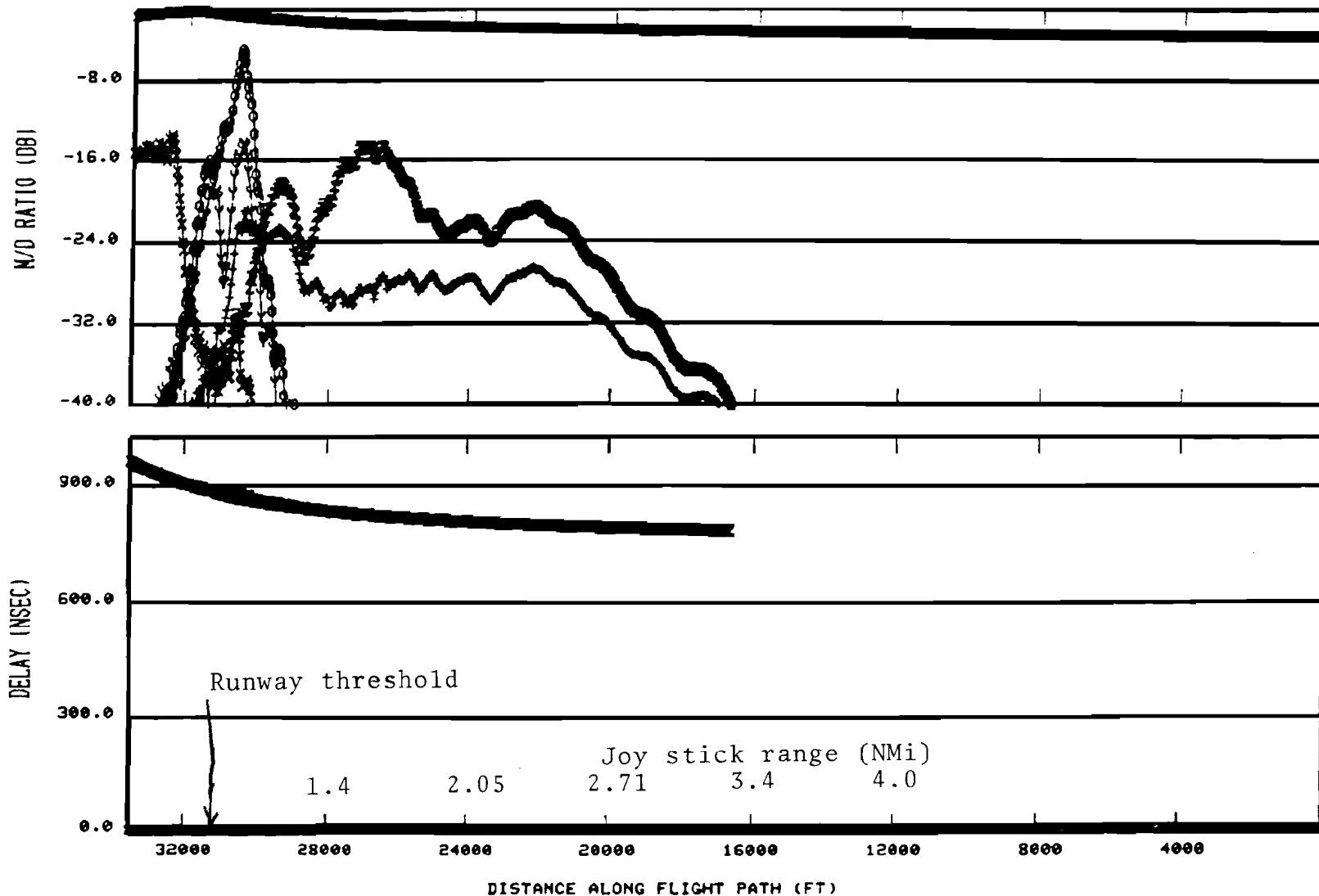
Fig. 8-15. Computed multipath characteristics for DCA 3 rd Approach scenario.
