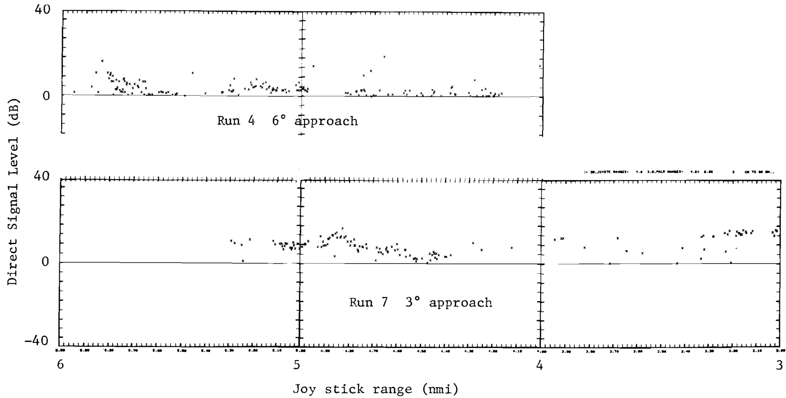
Fig. 8-21. Direct signal strength levels at Washington National Airport.
