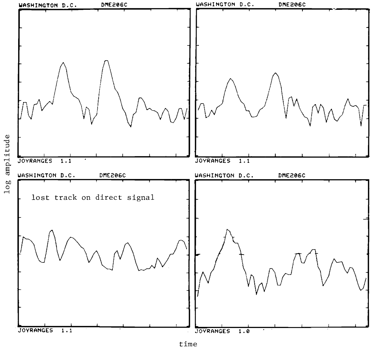
Fig. 8-9. DCA waveforms near threshold on 6° approach.
