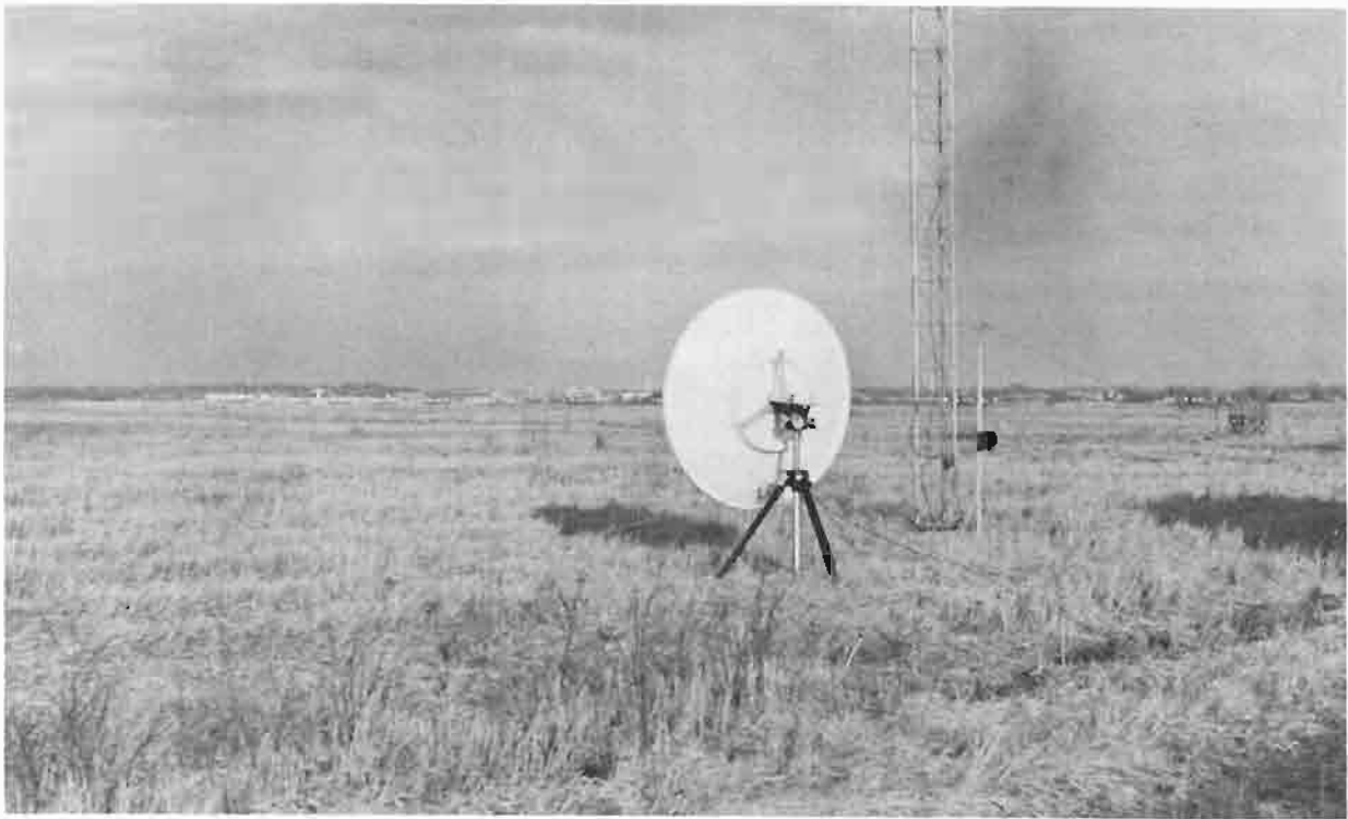
Fig. 6-3a. DME multipath measurement equipment at Wright Patterson AFB, Ohio.
