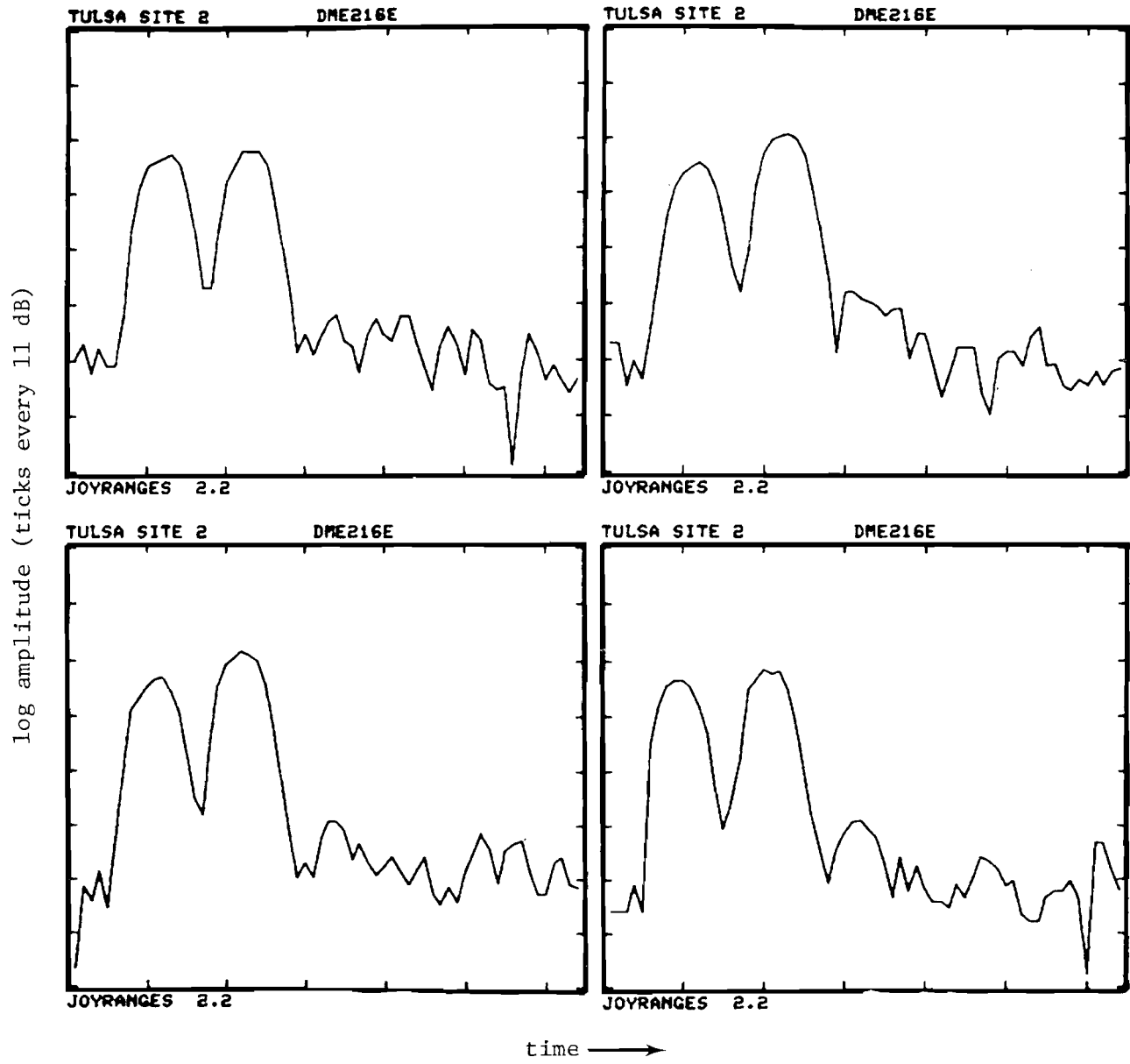
Fig. 5-17. Tulsa site 2 waveforms near threshold.
