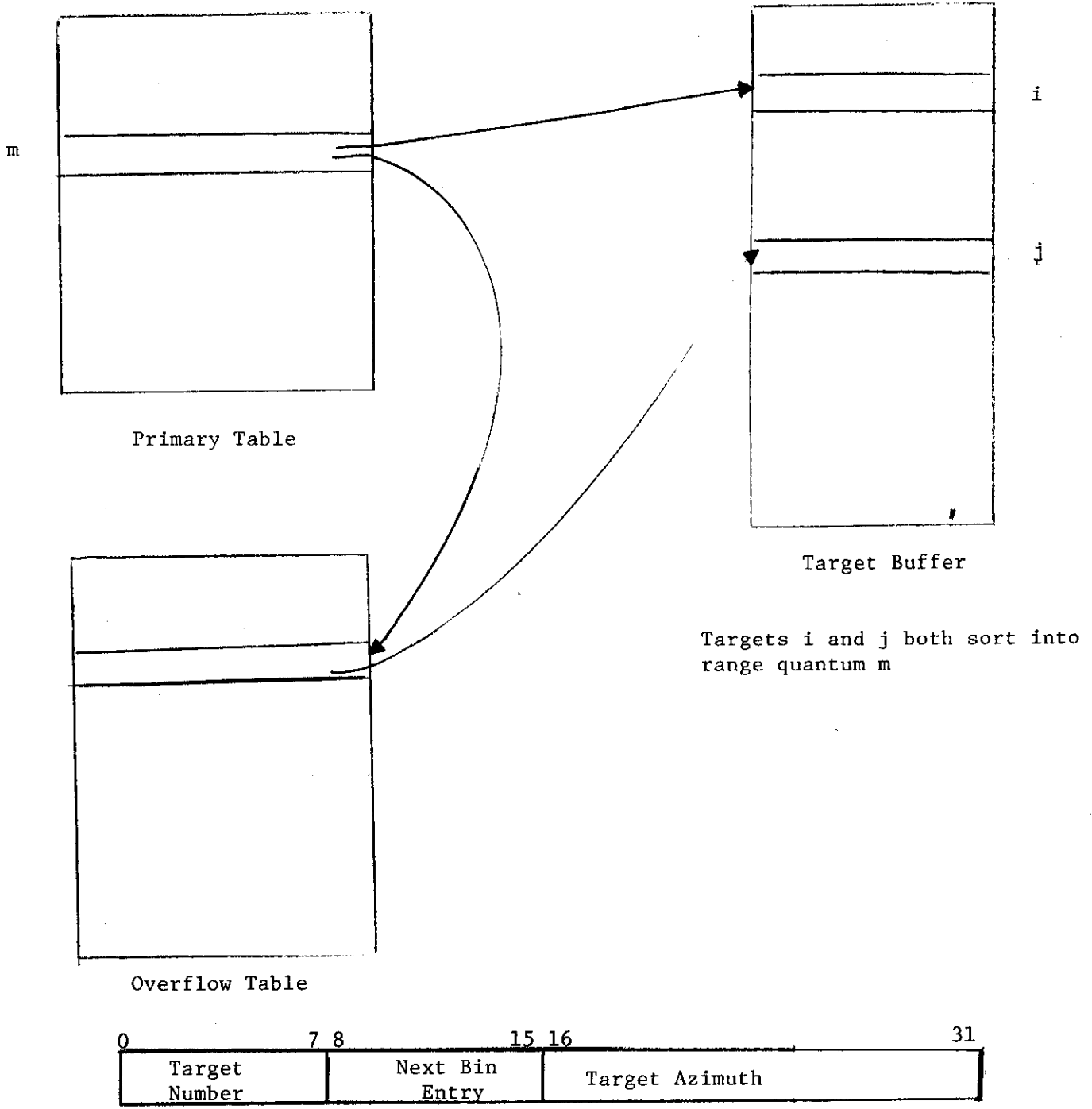
Sort Table Entry
