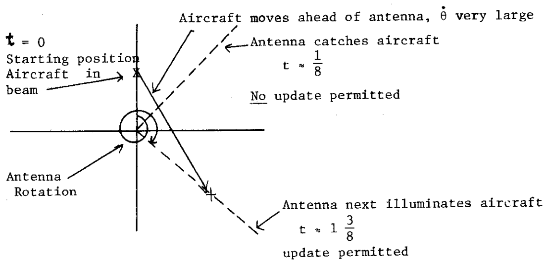
(a) Special case, time between reports < \frac{1}{2} scan
