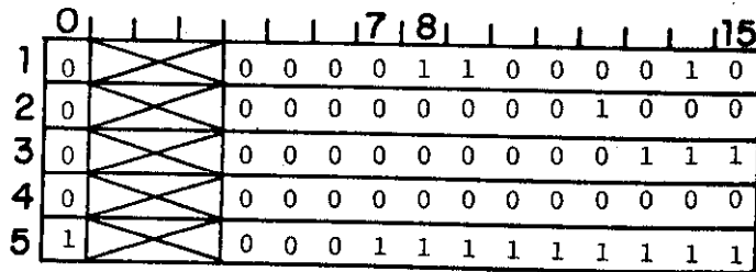
Status Report
