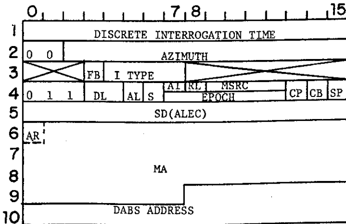
COMM-A INTERROGATION (112 BITS)
