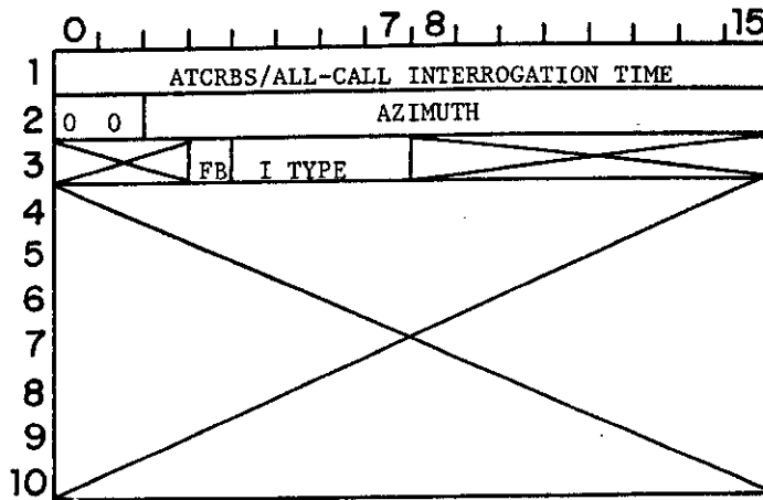
ATCRBS/ALL-CALL INTERROGATION
