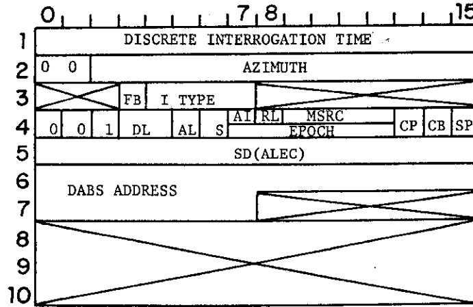
SURVEILLANCE INTERROGATION (56 BITS)
