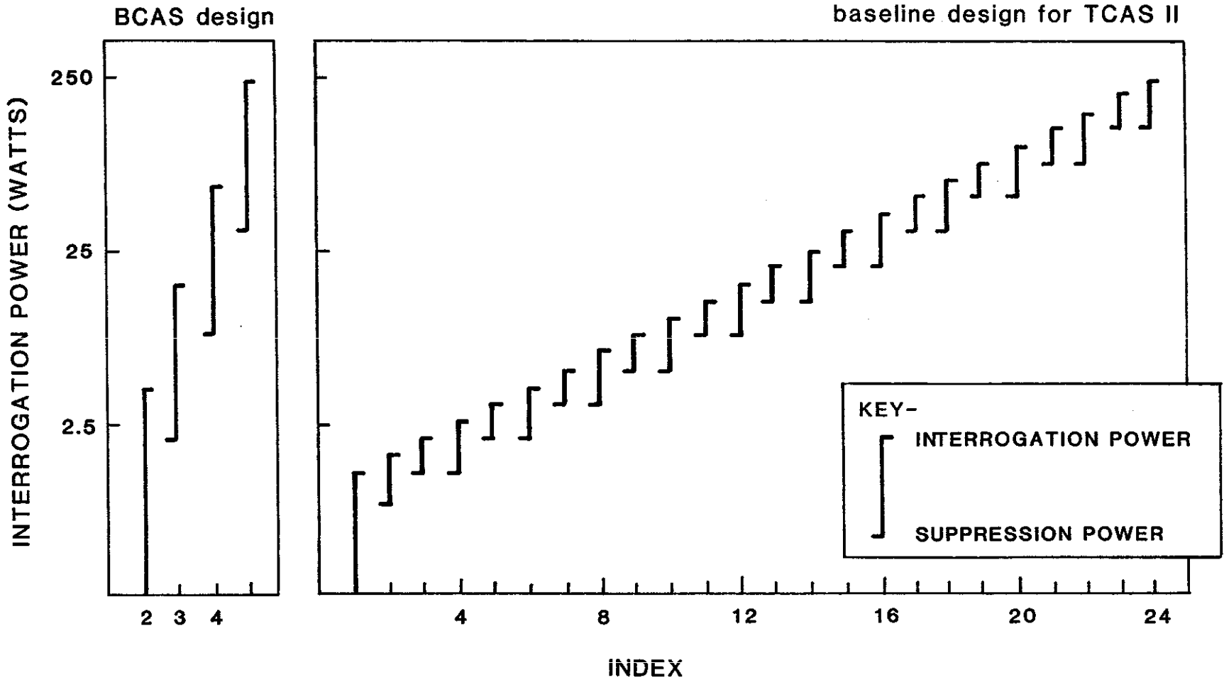
Fig. 3-5. Baseline whisper-shout design.
