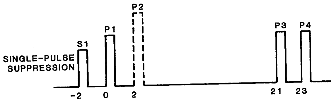
Fig. 3-9. Single-pulse suppression.
