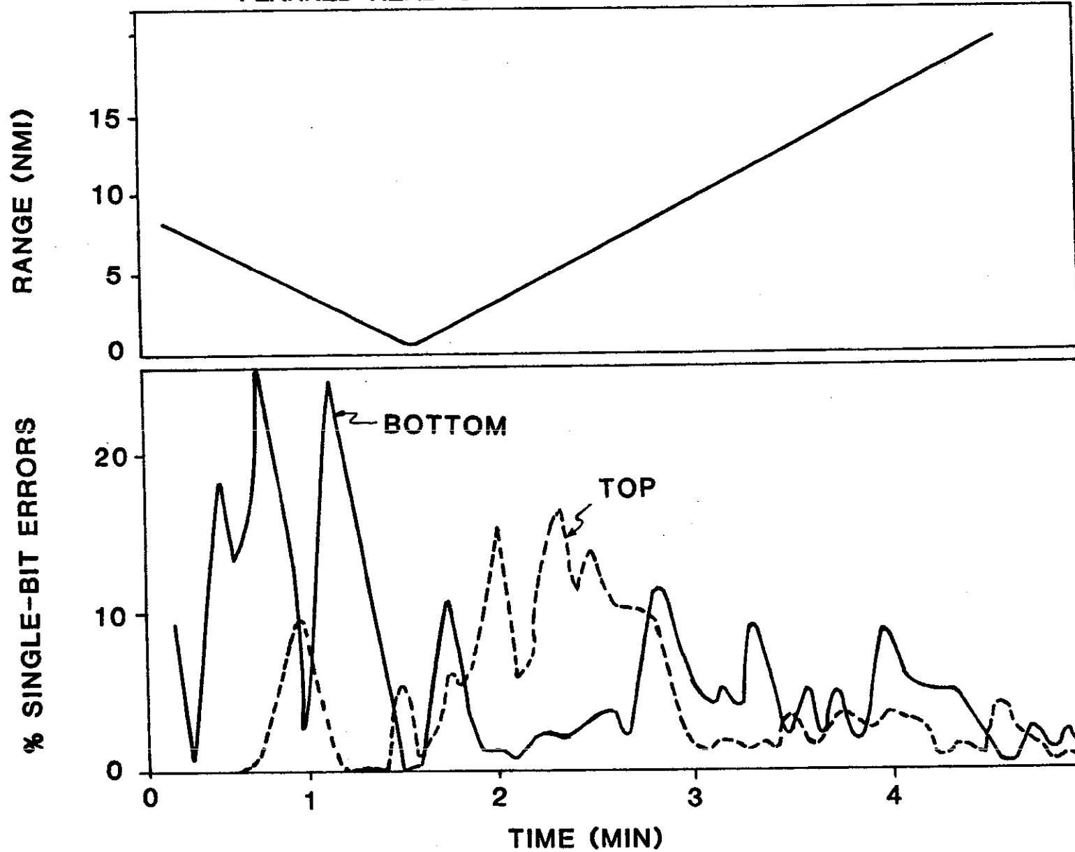
Fig. 4-5. Single-bit error rate observed in high density airspace.
