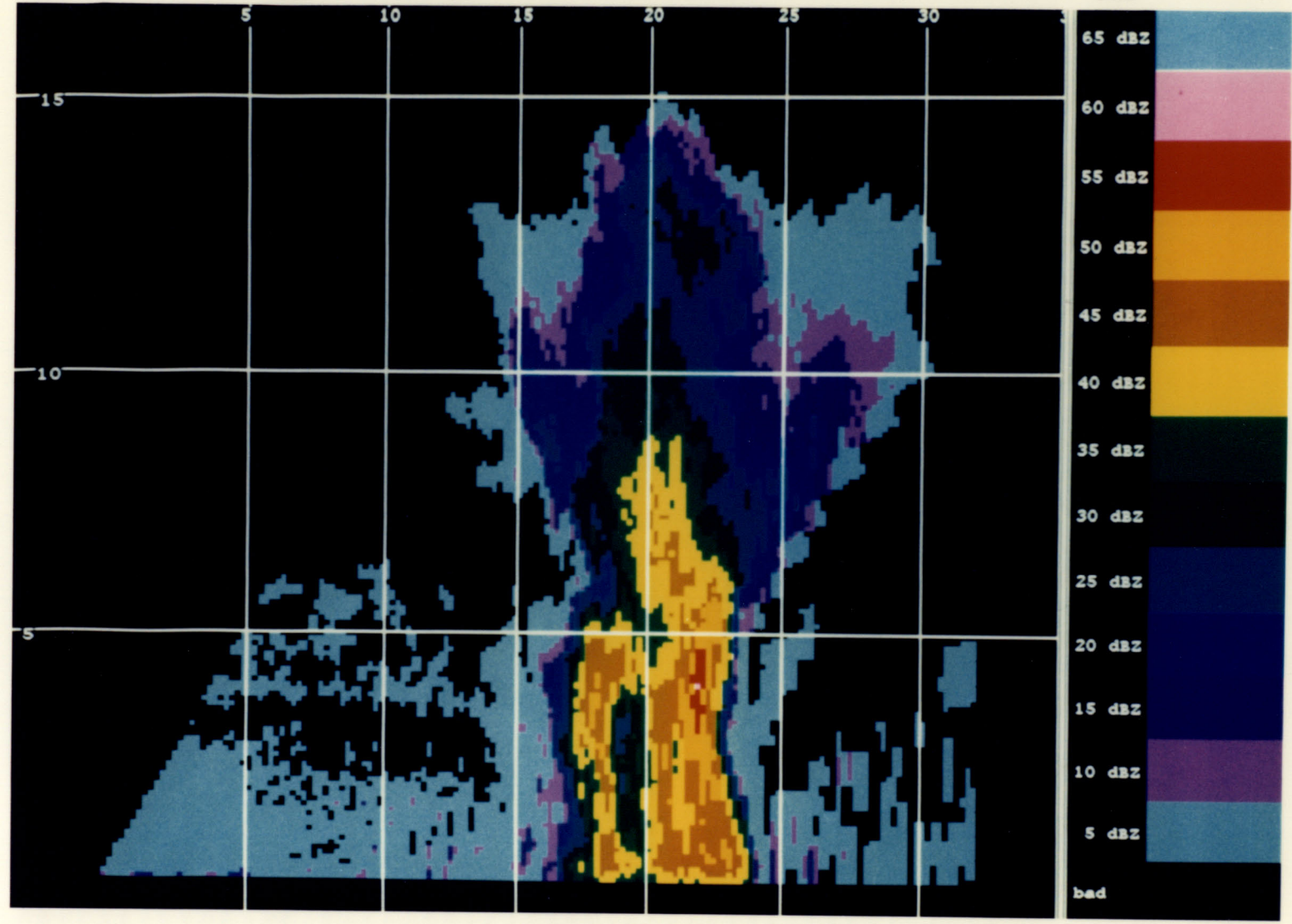
Fig. 1. Hail spike as portrayed in reflectivity field.
