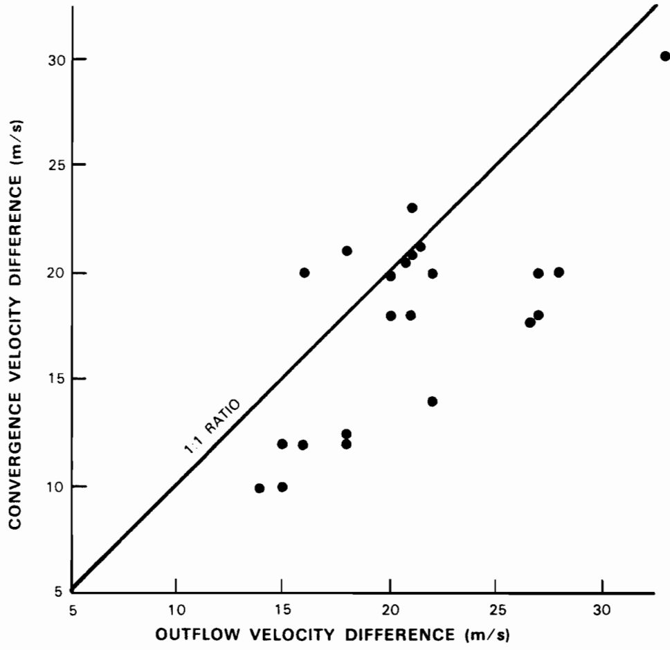
Fig. 2. Scattergram of convergence and surface outflow (m/s).
