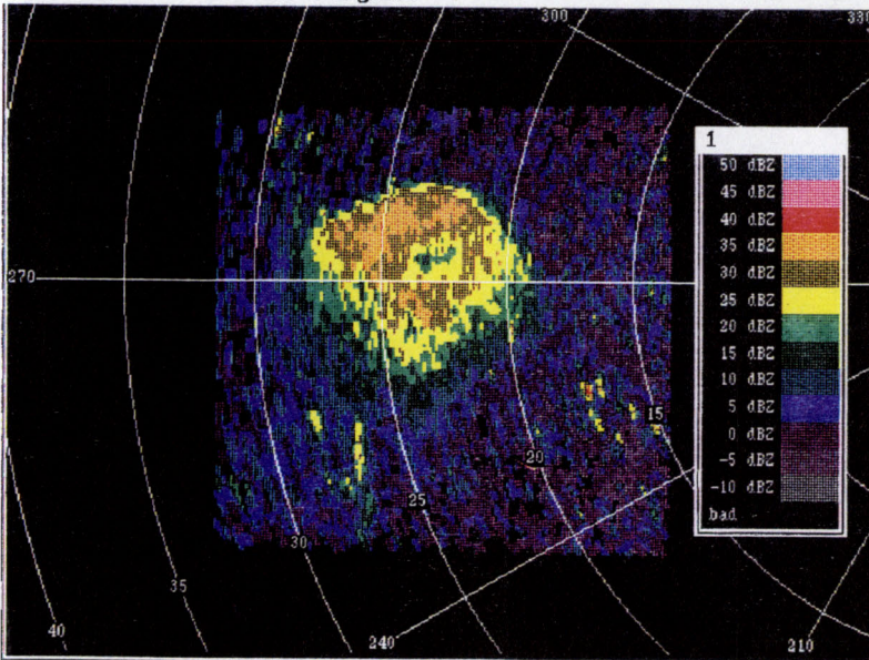
Figure 4. Reflectivity and velocity images of a birdburst on 29 July 1986 in Huntsville, Alabama.
