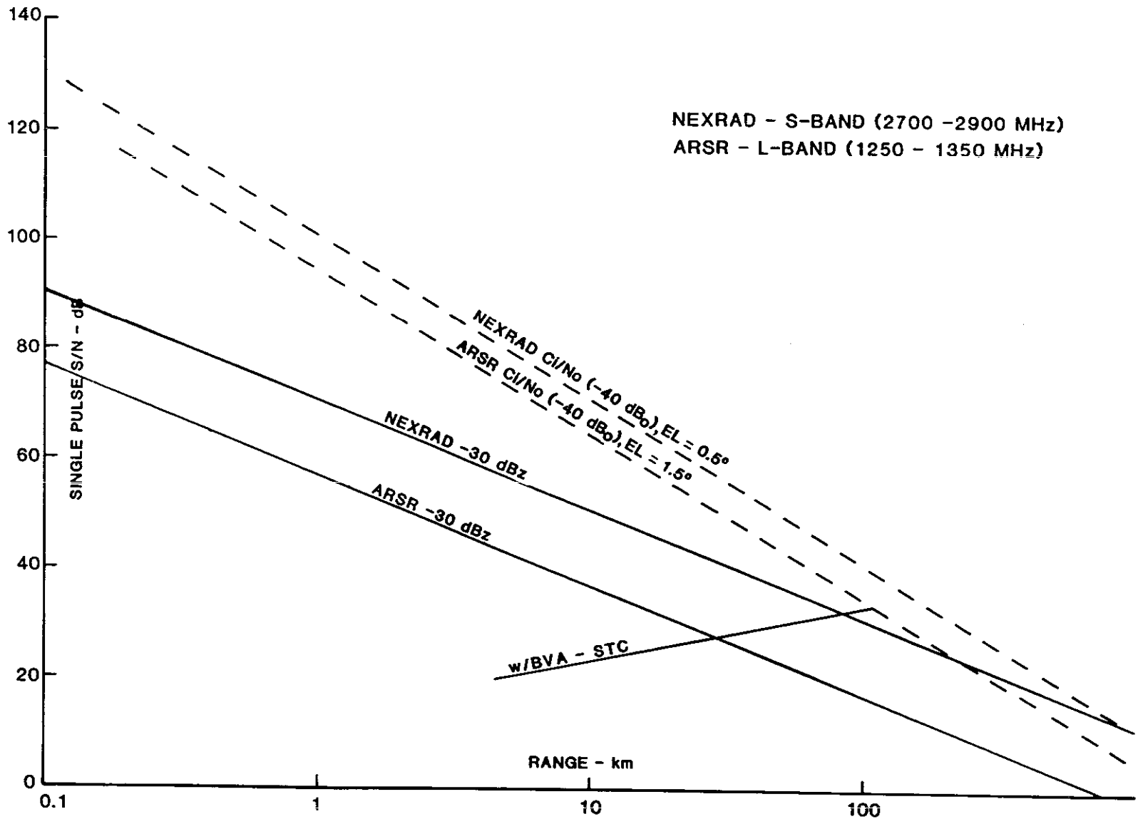
Fig. A-3. Signal-to-noise vs range for weather and ground clutter.
