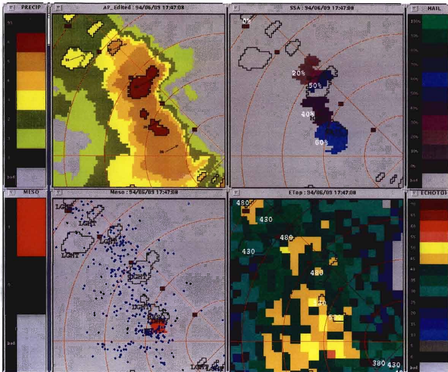
Figure 7. Example of how the SCI product is generated. Storm cell outlines are overlaid on (a) the ITWS 6-level precipitation, (b) probability of severe hail (percent), (c) lightning flashrate (flashes per minute; blue dots) and mesocyclone detections (red squares), and (d) echo tops (x1000 feet). The data for each grid are searched within the outlines to determine the appropriate information to issue in the text box.
