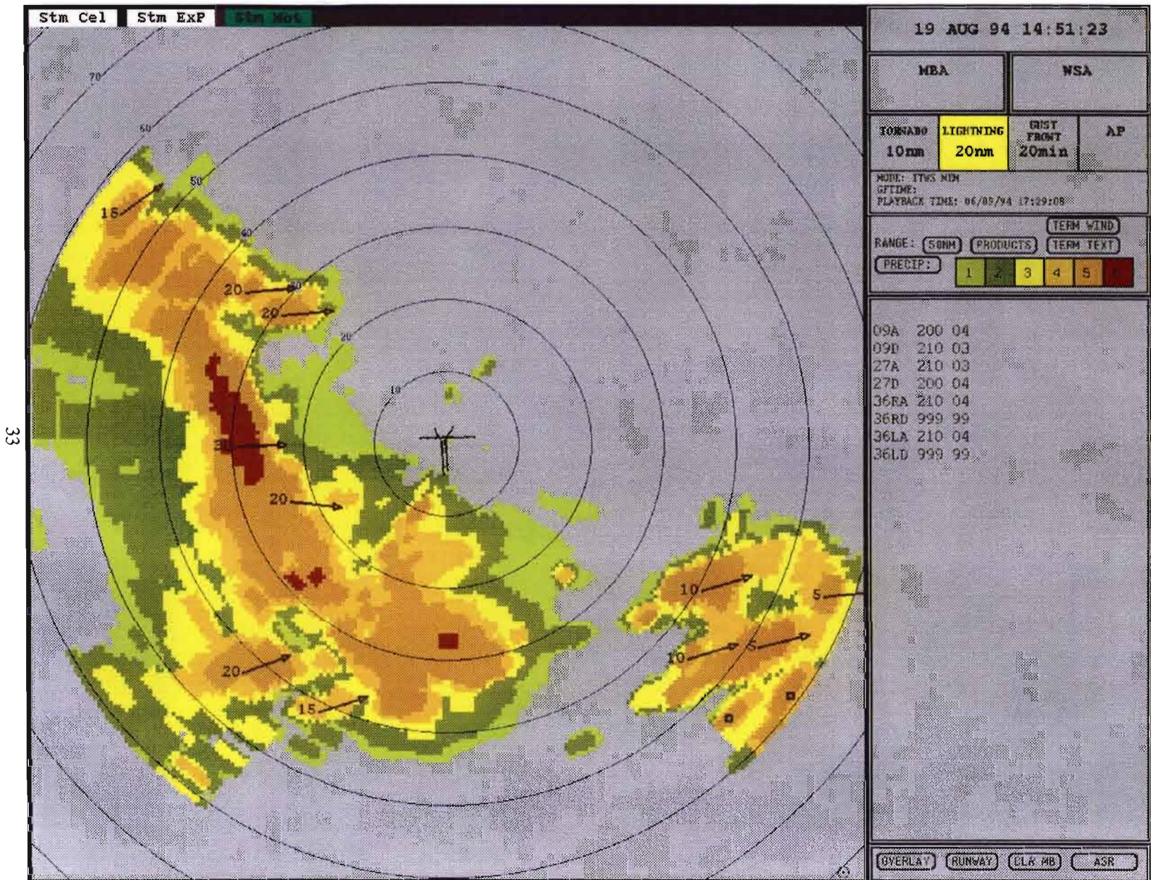
Figure 8. Example of the ITWS Storm Motion product. The arrows overlaying the precipitation product indicate the direction of motion of the storm and the number positioned at the base of the arrow indicates speed of motion in knots
