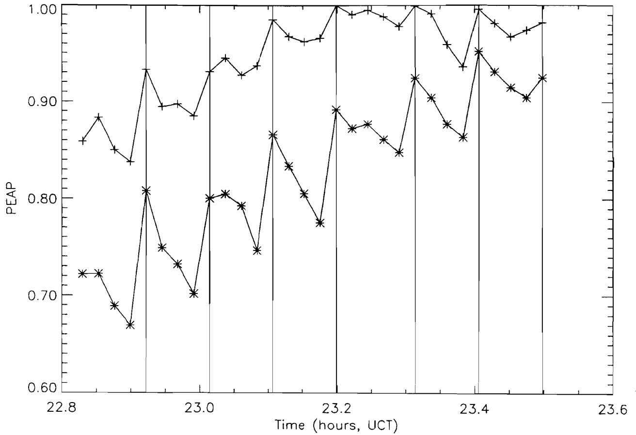
Figure 5. Time series of PEAP for level 2 and greater (*) and level 3 and greater (+) AP.
