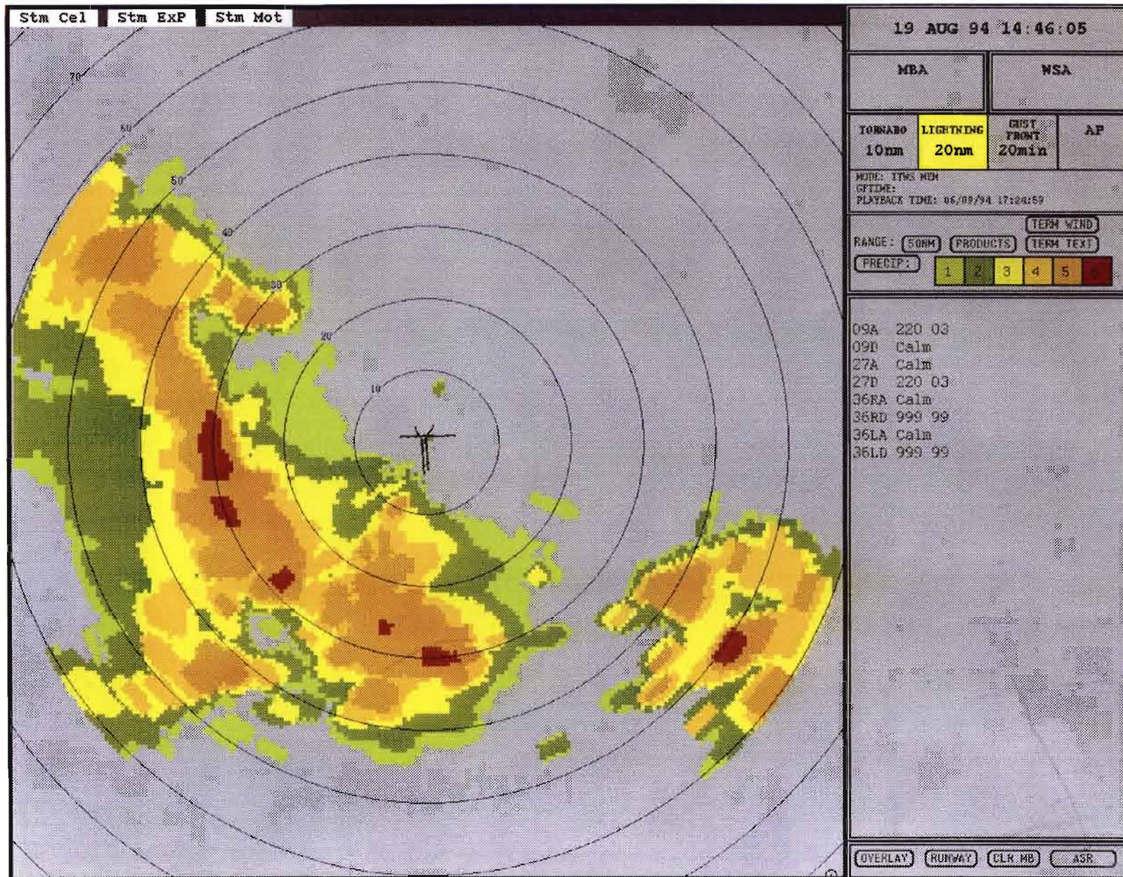
Figure 17. Example of the Lightning Detection product. The yellow box in the upper right corner is illuminated when cloud-to-ground lightning is detected within a user-specified distance (20 nm for ATC users; 5 nm for other users) of the airport reference point.
