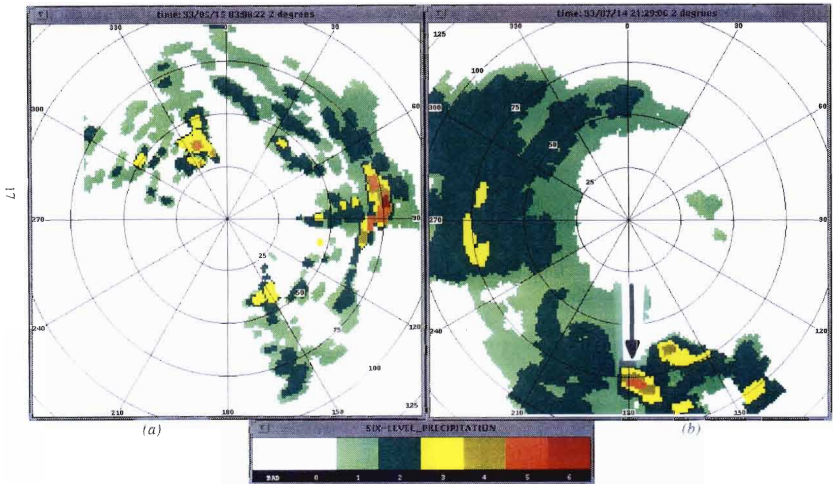
Figure 4. Examples of Anomalous Propagation (AP) in ASR-9 weather channel data. (a) AP created by a nocturnal inversion at Dallas-Ft. Worth International Airport. At the time of this image, the skies were cloud-free. (b) AP created by a cold thunderstorm outflow passing over the ASR-9 radar at Orlando International Airport. The level 5 weather indicated by the arrow is in reality level 3. Contamination of weather returns by AP causes weather levels to appear higher than they really are.
