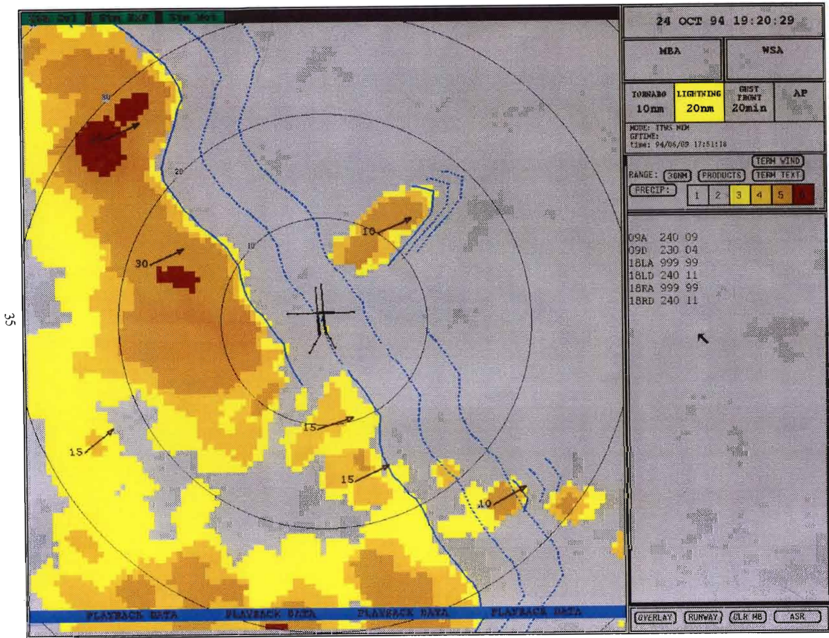
Figure 9. Example of the ITWS Storm Extrapolated Position product. The solid blue line indicates the current location of the leading edge of the level 3 or greater precipitation; the dashed lines are the 10- and 20-minute extrapolated positions of the leading edge.
