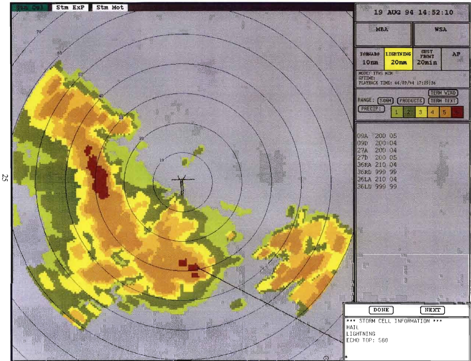
Figure 6. Example of the SCI product. The text box at the lower right corner of the figure provides information about the storm cell to which the black line is drawn. HAIL indicates a greater than 50 percent probability of the presence of severe hail at the ground; LIGHTNING indicates a cloud-to-ground lightning flashrate of three flashes per minute in the storm; ECHO TOP provides an estimate of the echo top of the storm above ground level in units of (x 100) feet; SEVERE STORM indicates the presence of strongly rotating horizontal winds and strong updrafts in the storm.
