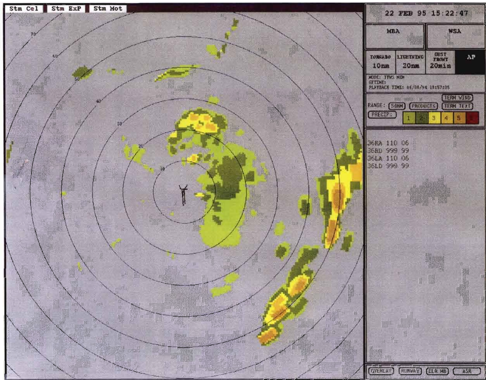
Figure 2. Example of the ITWS Precipitation Product. The six levels are color-coded according to the key at the upper right of the figure. Greens represent lighter precipitation; reds represent heavier precipitation. The AP alert panel in the upper right corner of the Situation Display illuminates (black with white text) when a region of AP is detected that exceeds five square miles.
