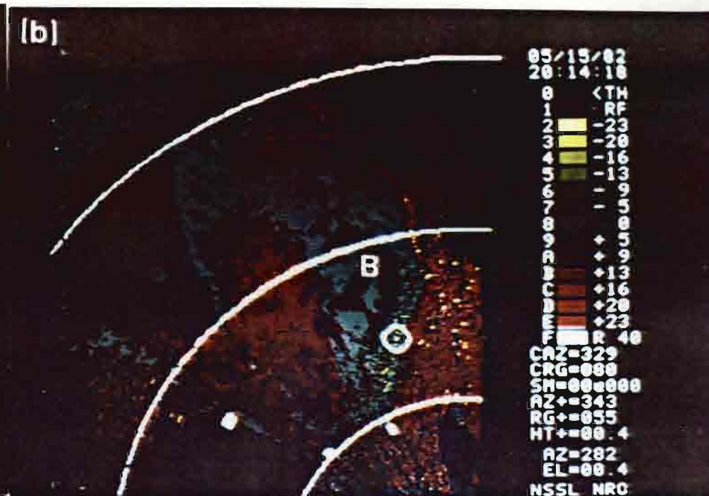
Figure IV-4. Plan Position Indicator displays from Norman, OK Doppler radar for 15 May 1982, 20:14:18 CST, ST=0dB:
