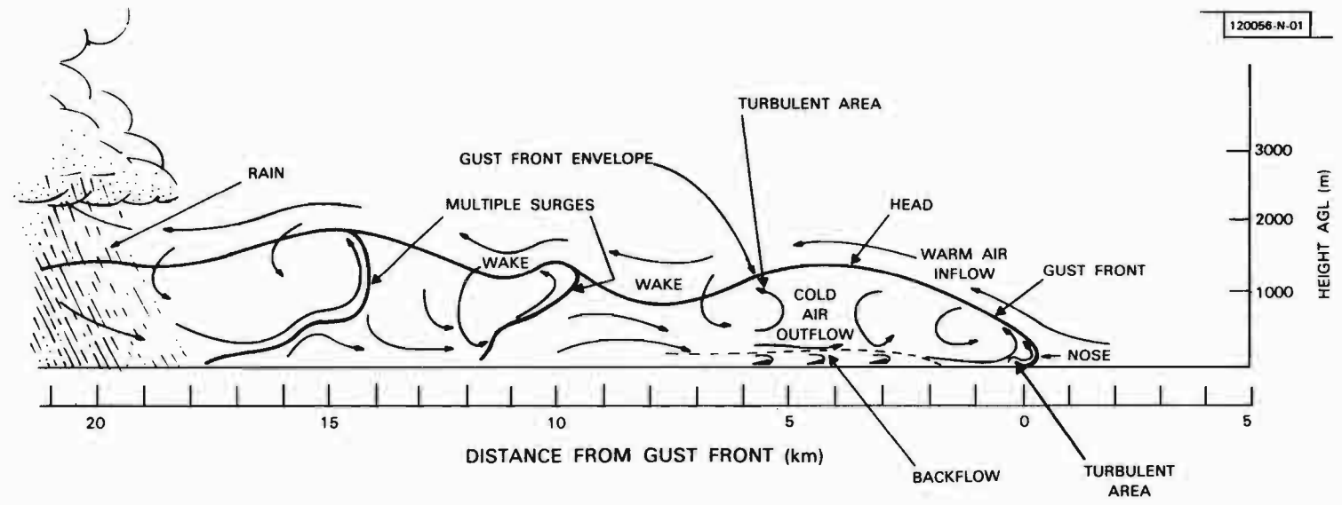
Fig. II-2. Schematic diagram of the vertical structure of a thunderstorm outflow and gust front. Motion is gust front relative. (Adapted from Goff, 1976.)
