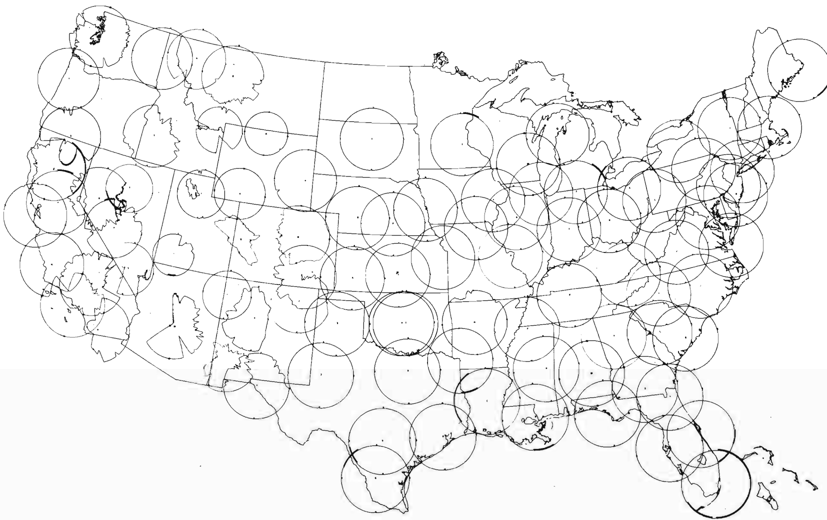
Fig. A.19. ARSR composite coverage map, 15,000 ft. MSL, maximum range R_{\max} = 100 nmi.
