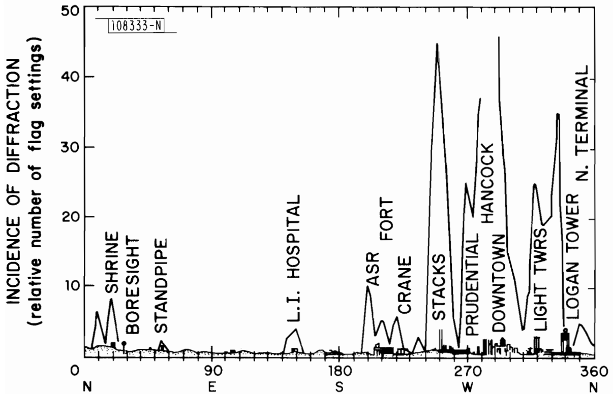
Fig. 2.14. Incidence of monopulse diffraction errors at Logan Airport.
