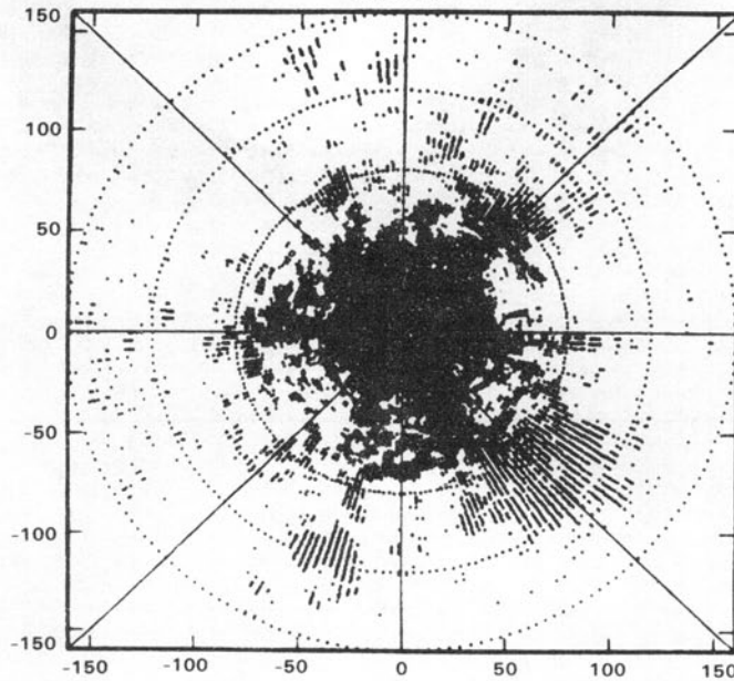
Fig. 3.11d. Comparison of NSSL and M.I.T. clutter data at 0.4° elevation angle.
