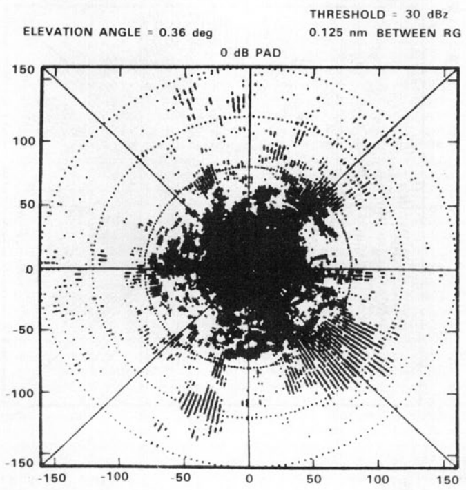
Fig. 3.11b. Comparison of NSSL and M.I.T. clutter levels.
