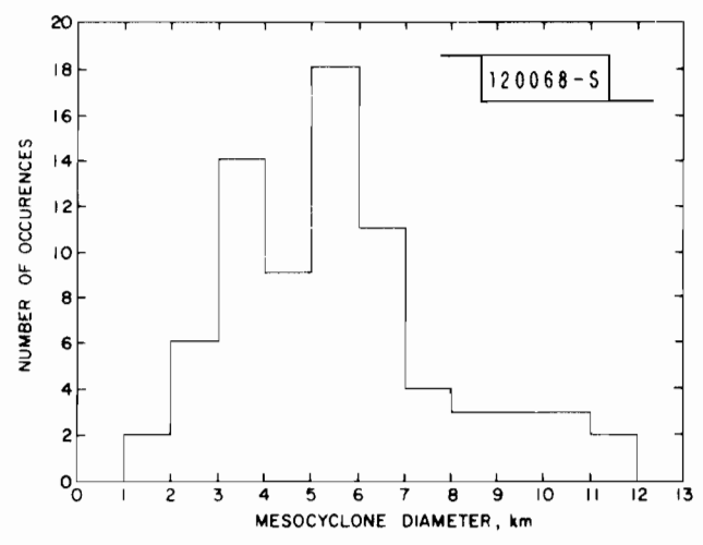
Fig. 3.16. Frequency of occurrence of measured mesocyclone diameters.
