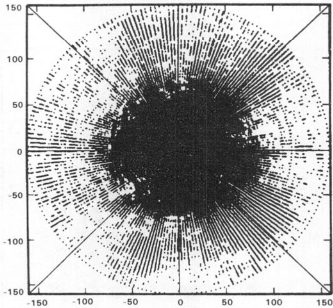
Fig. 3.11c. Comparison of NSSL and M.I.T. clutter data at 0.4° elevation angle.
