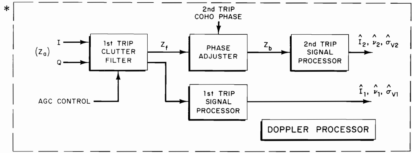
Fig. 3.5. Dual coherent interval system.
