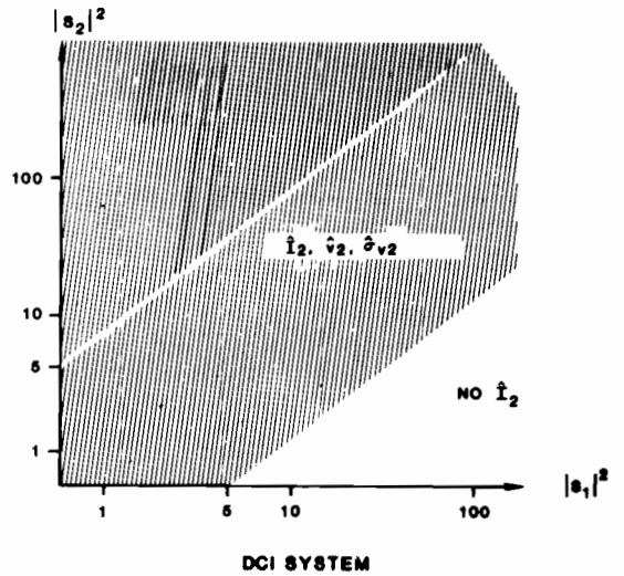
Fig. 3.9. Comparison of system performance in obscuration.
