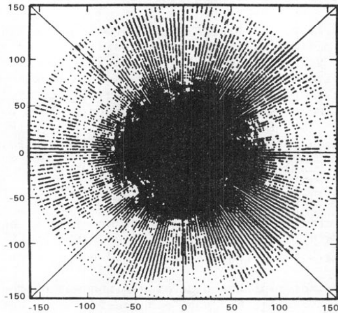
Fig. 3.11a. Comparison of NSSL and M.I.T. clutter levels.
