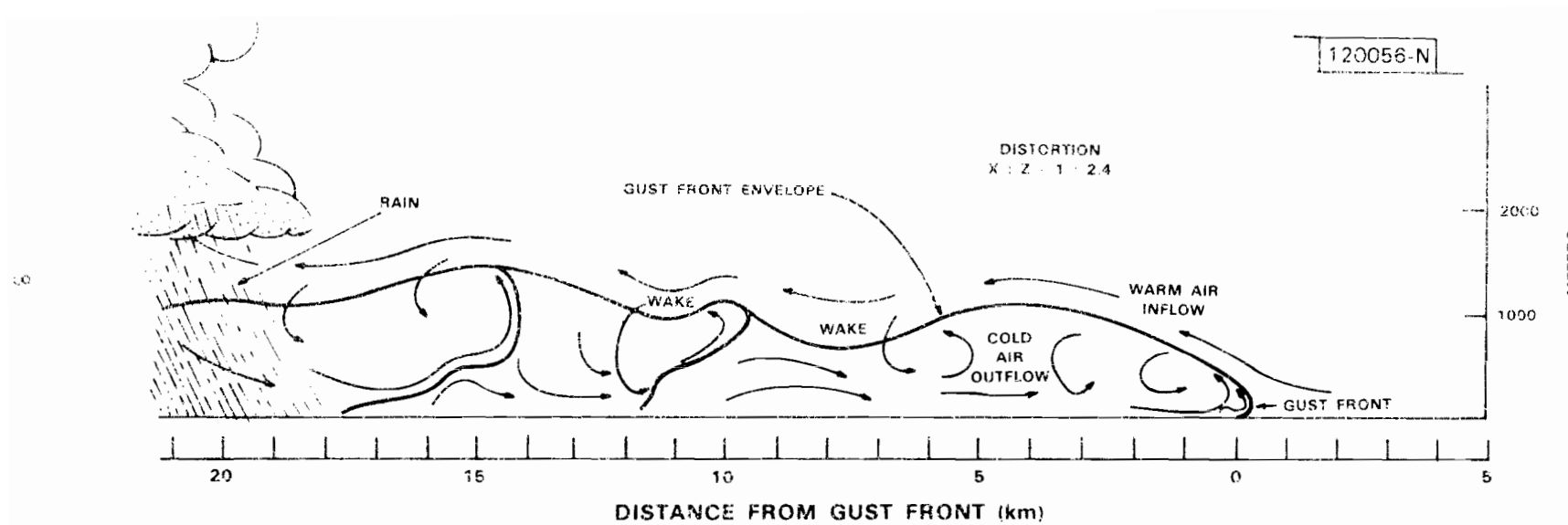
Fig. 1.3 Squall line thunderstorm outflow (schematic).
