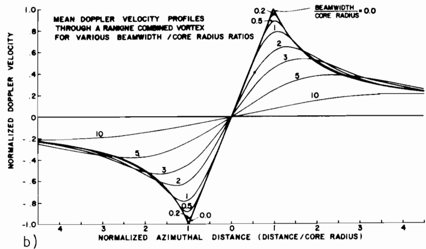
Fig. 3.15. (a) Single doppler horizontal mesocyclone signature of a stationary rankine combined radius. (b) Theoretical mean doppler velocity azimuthal profiles through a rankine combined vortex.
