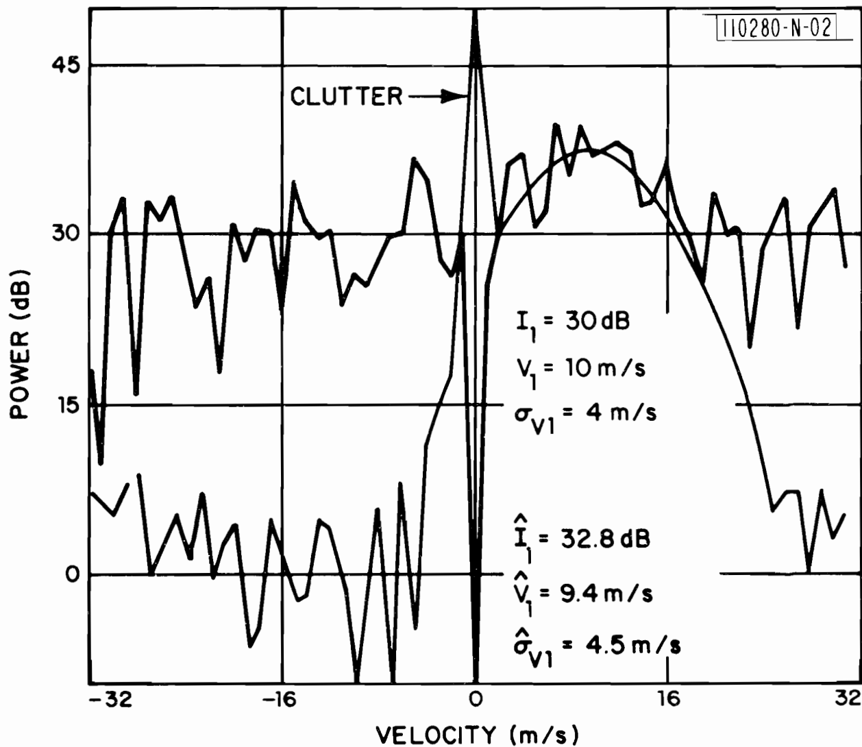
Fig. 3.7. Effects of decohered second trip echo on first trip signal.
