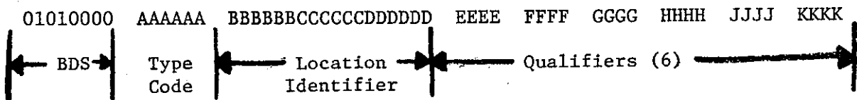
Fig. 4.1. Comm-B Message Field for Pilot Weather Requests.
