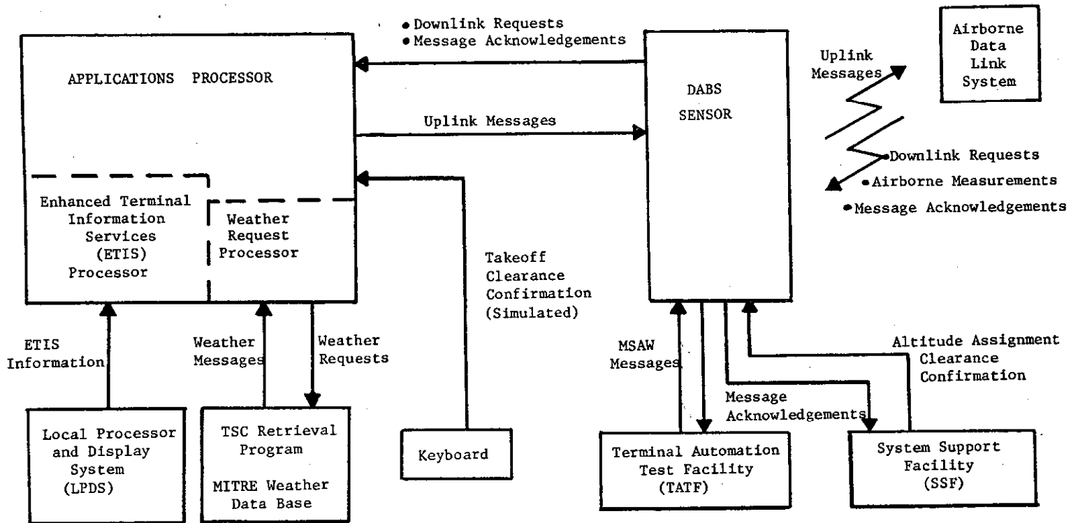
Fig. 1.1. DABS Data Link Communications Flow Diagram for NAPEC Tests and Evaluations.
