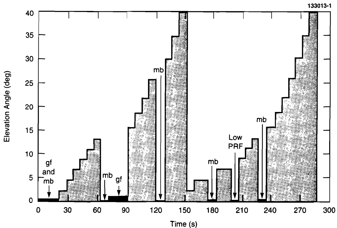
Figure 3: Antenna elevation-angle sequence used for the TDWR operational test and evaluation in 1988. The first scan in the sequence is a full-circle scan at an elevation of 0.6°. This scan is used jointly by the gust front and microburst algorithms. A second full-circle scan at an elevation of 1° is used by the gust front algorithm alone. The microburst algorithm further requires surface scans at one-minute intervals. These scans cover a 120° sector over the airport at an elevation angle of 0.4°. The PRF selection algorithm requires a long-range, low-PRF full-circle scan. The remaining scans are used by the microburst features aloft algorithms.
