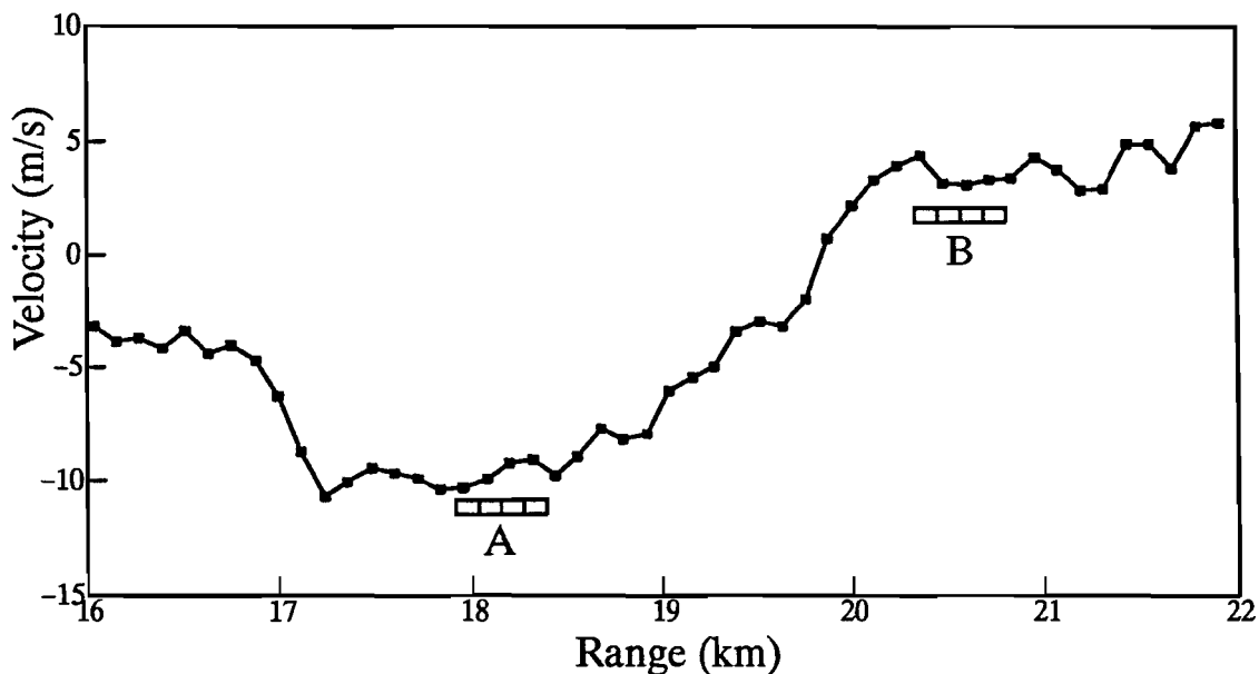
Figure 15: Example of the segment search window. The window consists of NUMBER(Window) range samples, starting at the current sample. The pattern of velocity measurements in the window determines if a segment is to be started or terminated. The window marked “A” is an example of a valid segment starting condition, while window “B” is the corresponding termination point.
