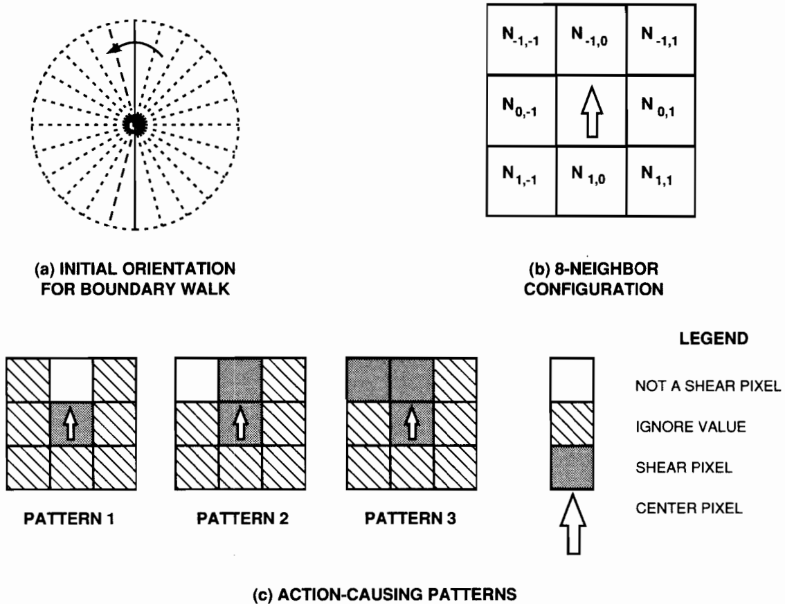
Figure 3.1: Region growing method employed by the DBA.
