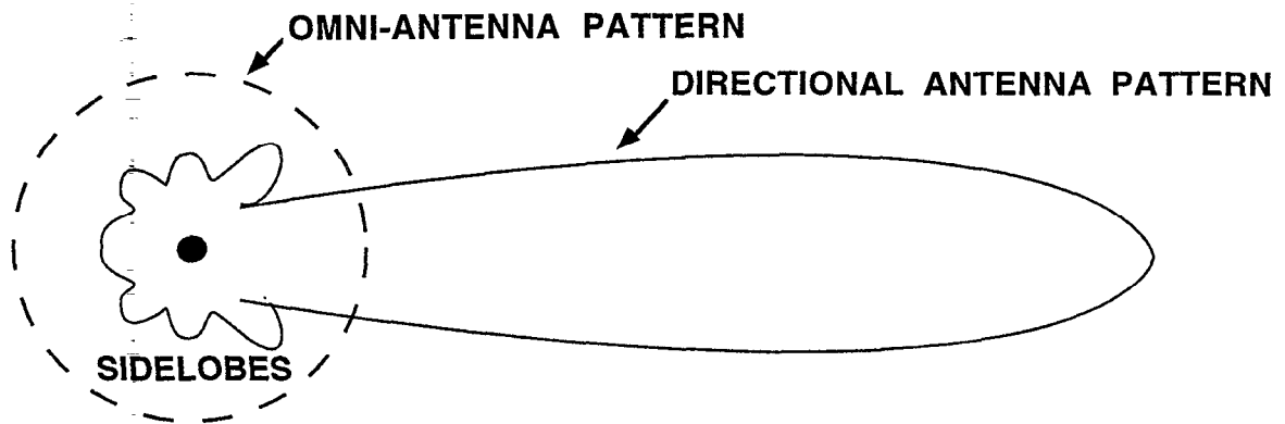
Figure 4. Main beam and omni-antenna patterns.
