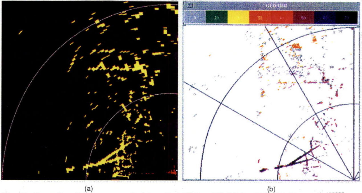
Figure 6. Comparison of geocensor maps for (a) standard ASR-9 and (b) ASR-9 with 9-PAC. The standard ASR-9 map is binary, whereas the 9-PAC map has variable threshold levels (as indicated by the color bar in relative dB). Note 9-PAC's increased detail of the roads just inside the 10-nmi range ring.
