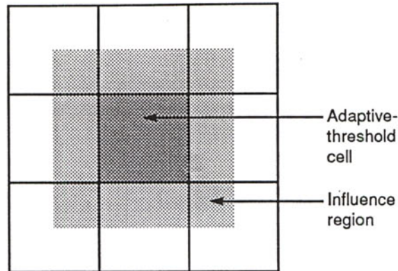
Figure 7. Adaptive-threshold cell ( 1/2 nmi \times 1/2 nmi) and influence region ( 1 mi \times 1 mi) used to update the fine-grain map. All targets falling in a cell's influence region are used to update the cell's histogram.
