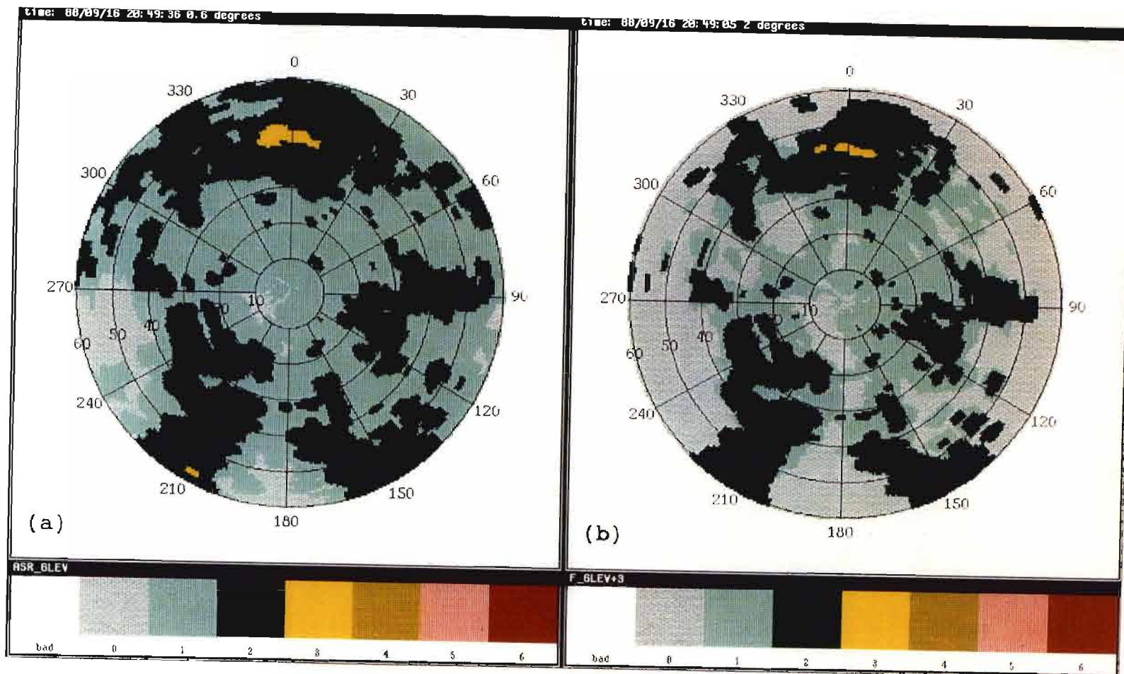
Figure 3-10. Comparison between (a) ASR-9 six-level and (b) emulation data increased by 3 dB, stratiform rain, 16 September 1988. Inspection indicates much better agreement between the two data products as was found without the 3 dB increase. The remaining discrepancy between Level 1 weather produced by both radars is assumed to be due to a difference in sensitivity between the two radars and threshold settings.
