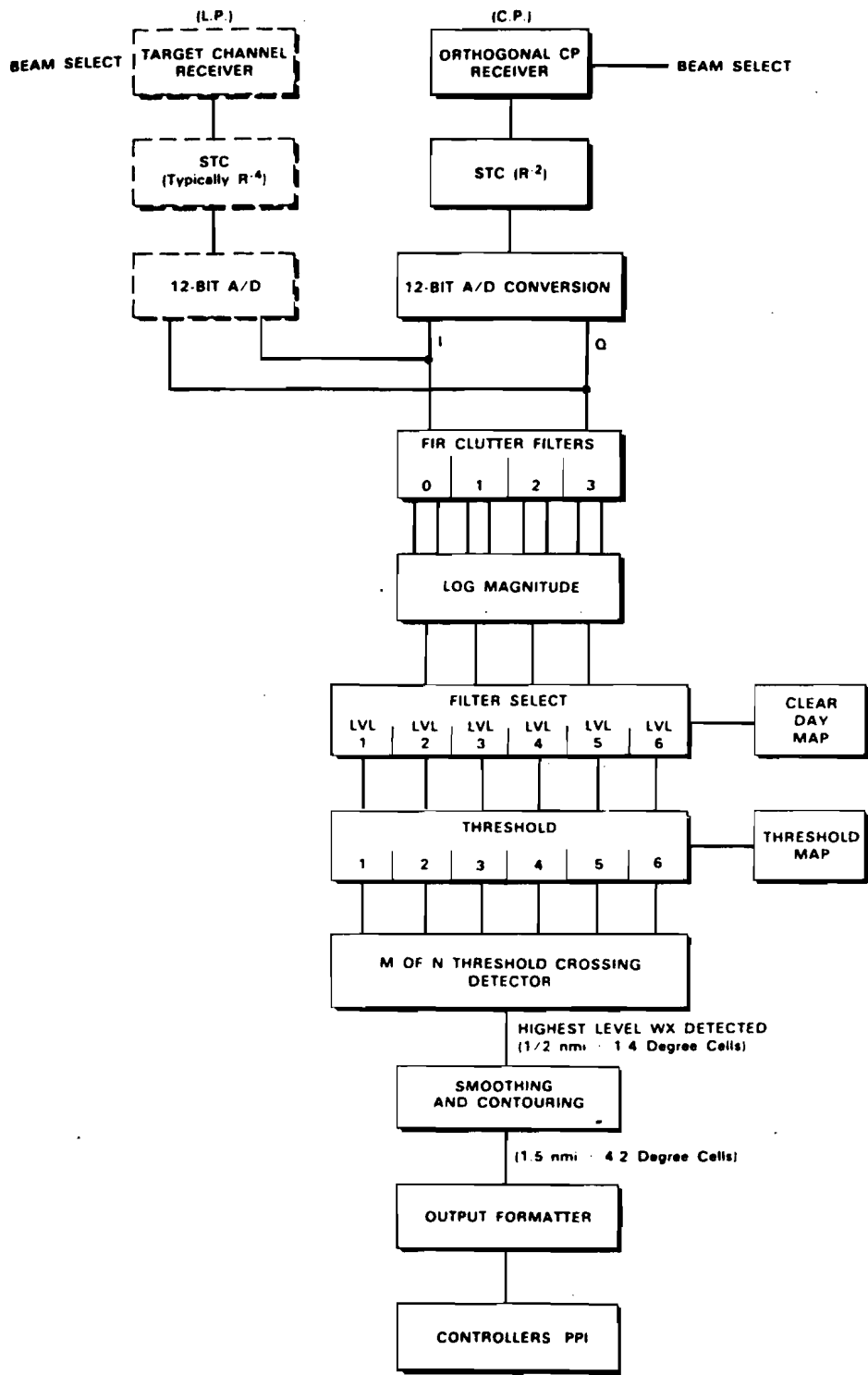
Figure 1-2. ASR-9 Weather Channel Processor Block Diagram.
