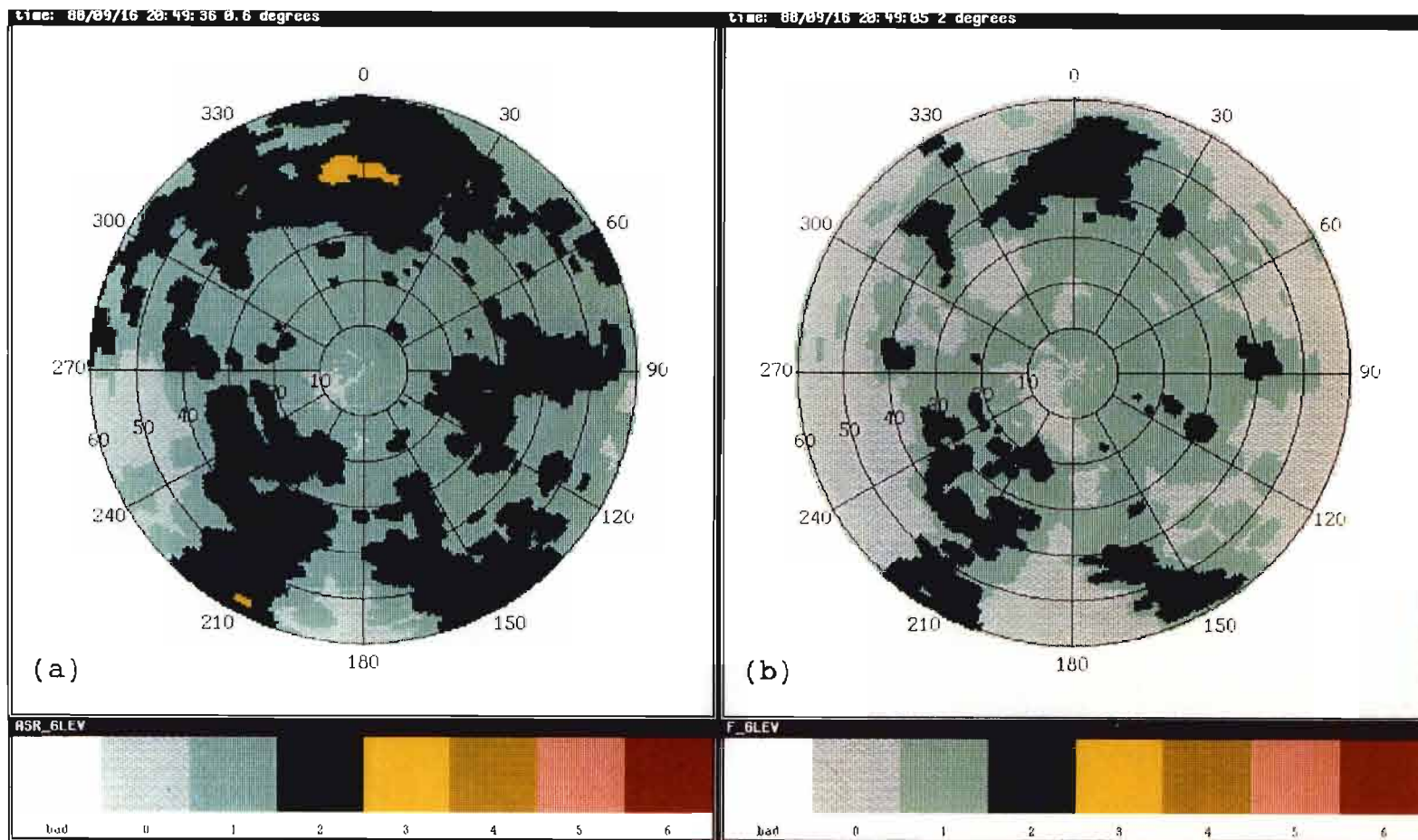
Figure 3-8. Comparison between ASR-9 six-level and emulation data, stratiform rain, 16 September 1988. Inspection indicates that the ASR-9 is reporting significantly more area for each level as well as higher levels than the FL-3 emulation data.
