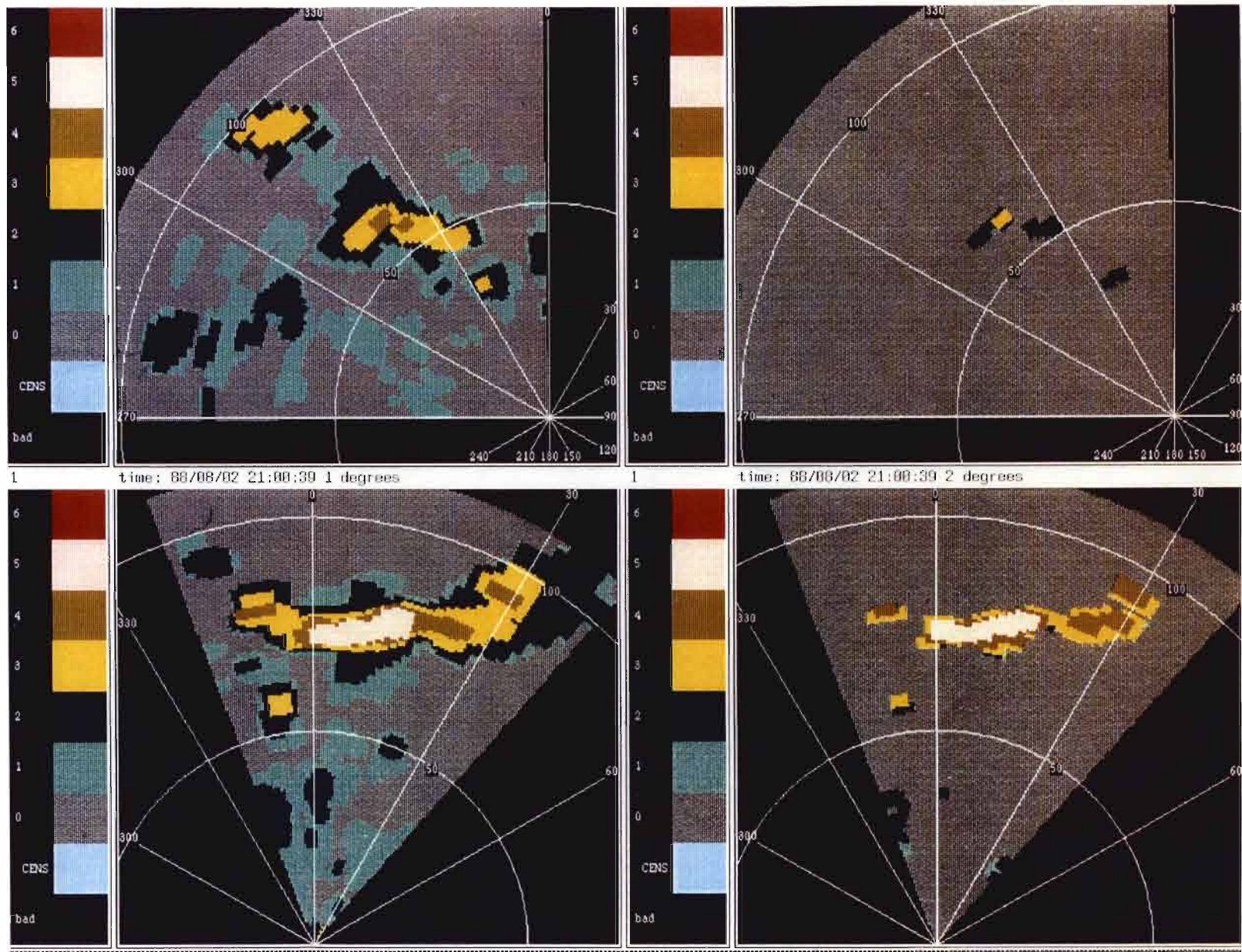
Figure I-3. FL-3 based emulation of ASR-9, showing effect of varying smoothing parameters on both AP and weather. (a) AP, 8 of 16, 5 of 9 spatial filters. (b) AP, 15 of 16, 9 of 9 spatial filters. (c) Weather, 8 of 16, 5 of 9 spatial filters. (d) Weather, 15 of 16, 9 of 9 spatial filters.
