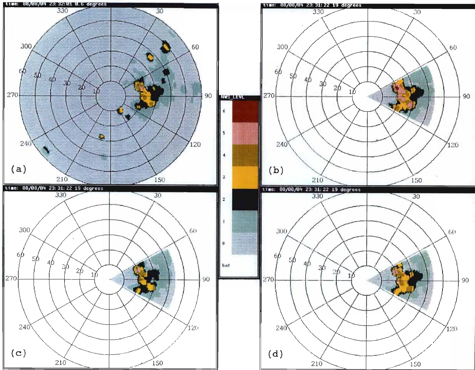
Figure 3-22. Comparison between (a) ASR-9 six-level and (b) MIT based maximum, (c) average, and (d) horizon-scan data, convective storm, 4 August 1988. Inspection indicates that the ASR-9 data agree best with the average and horizon-scan reflectivity data, suggesting that the ASR-9 beamfill correction storm model is not appropriate for this storm event.
