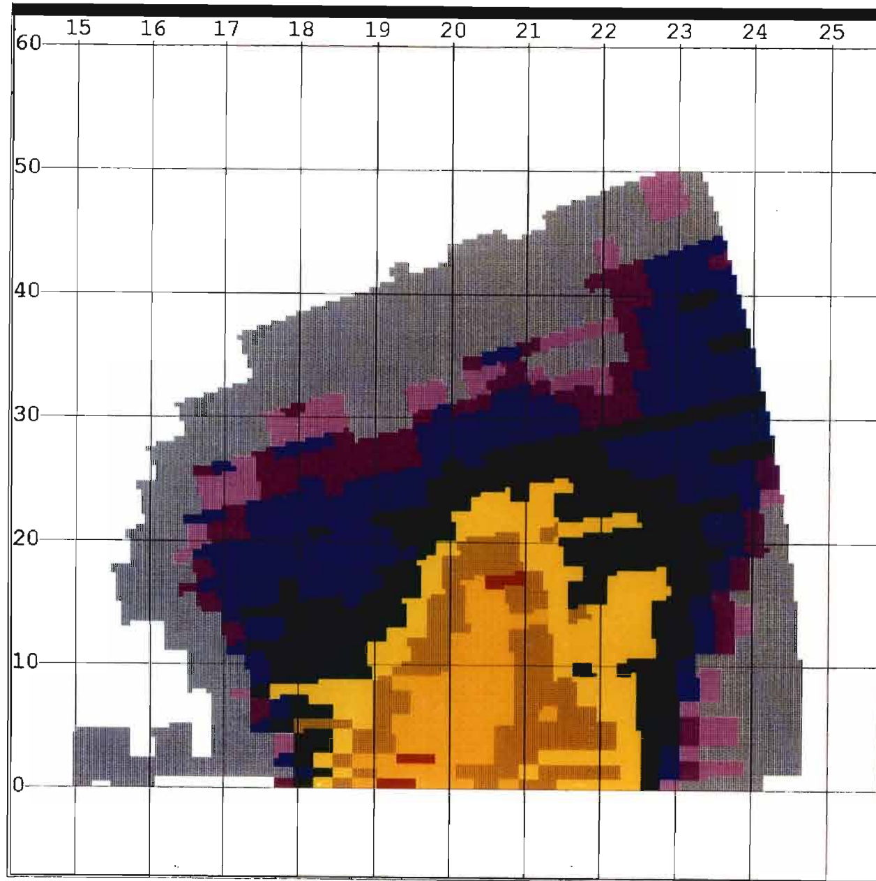
Figure 3-24. RHI at 75 degrees azimuth generated from MIT volume scan data for event shown in Figure 3-22. Range is in nautical miles; altitude is in thousands of feet. This figure shows the vertical reflectivity profile of the storm with its core extending from the ground up to about 5 km (16,400 ft.).
