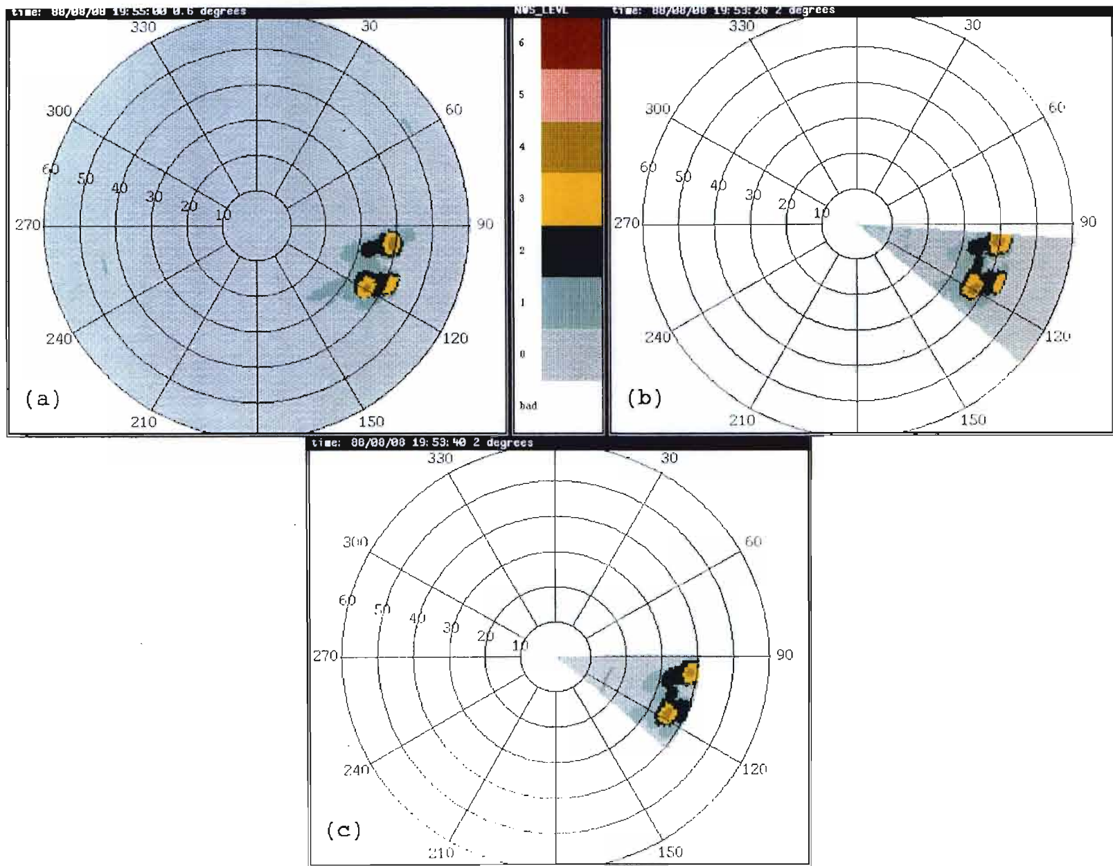
Figure 3-6. Comparison between (a) ASR-9 six-level, (b) simulation, and (c) emulation data, convective storm, 8 August 1988. Inspection indicates excellent agreement among the three data products.
