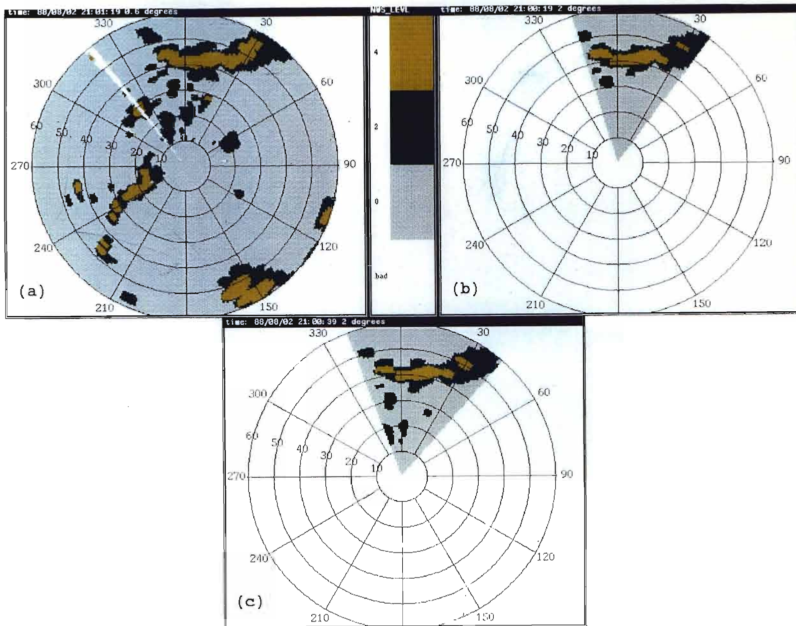
Figure 3-1. Comparison between (a) ASR-9 two-level, (b) simulation, and (c) emulation data, convective storm, 2 August 1988. Inspection indicates good agreement among the three data products.
