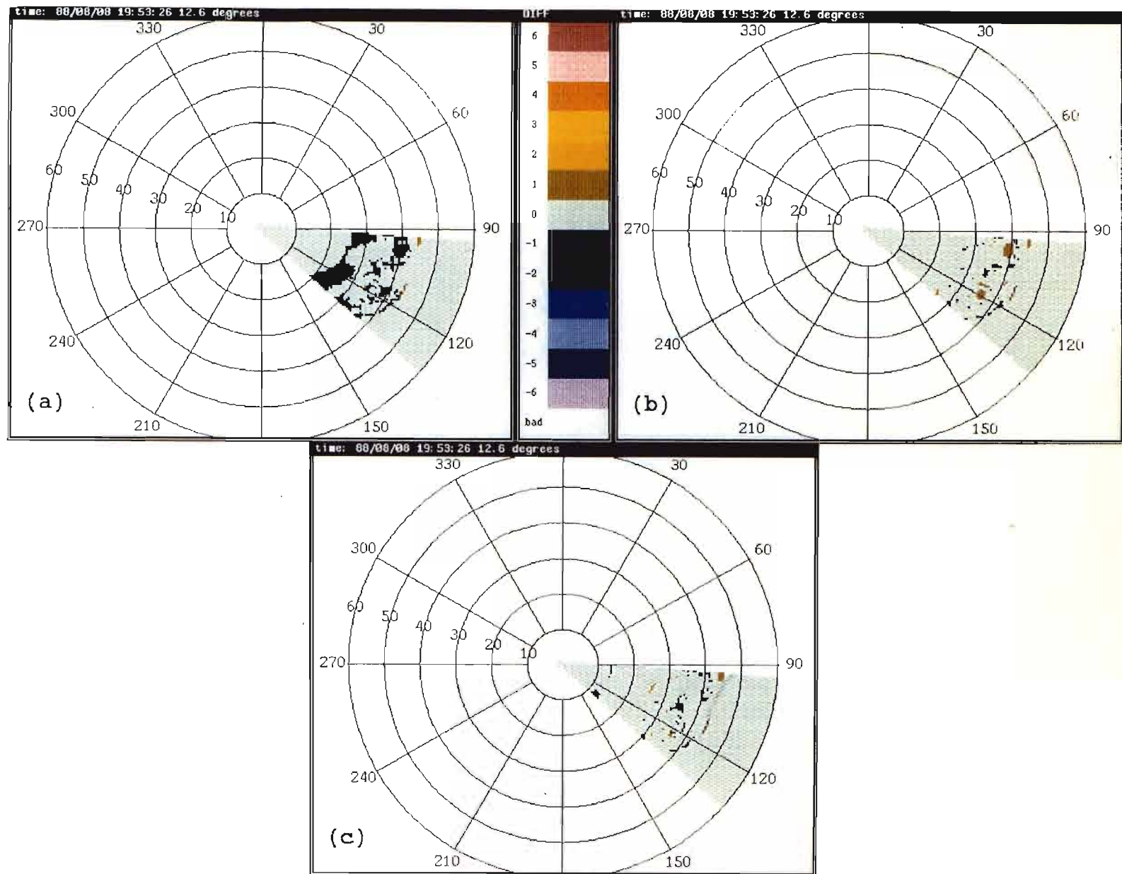
Figure 3-26. Reflectivity difference between ASR-9 six-level and (a) MIT based maximum, (b) average, and (c) horizon-scan data, convective storm, 8 August 1988. Statistics show that the ASR-9 data agree best with the average and horizon-scan reflectivity data, while the maximum data is sometimes two levels higher than the ASR-9 data.
