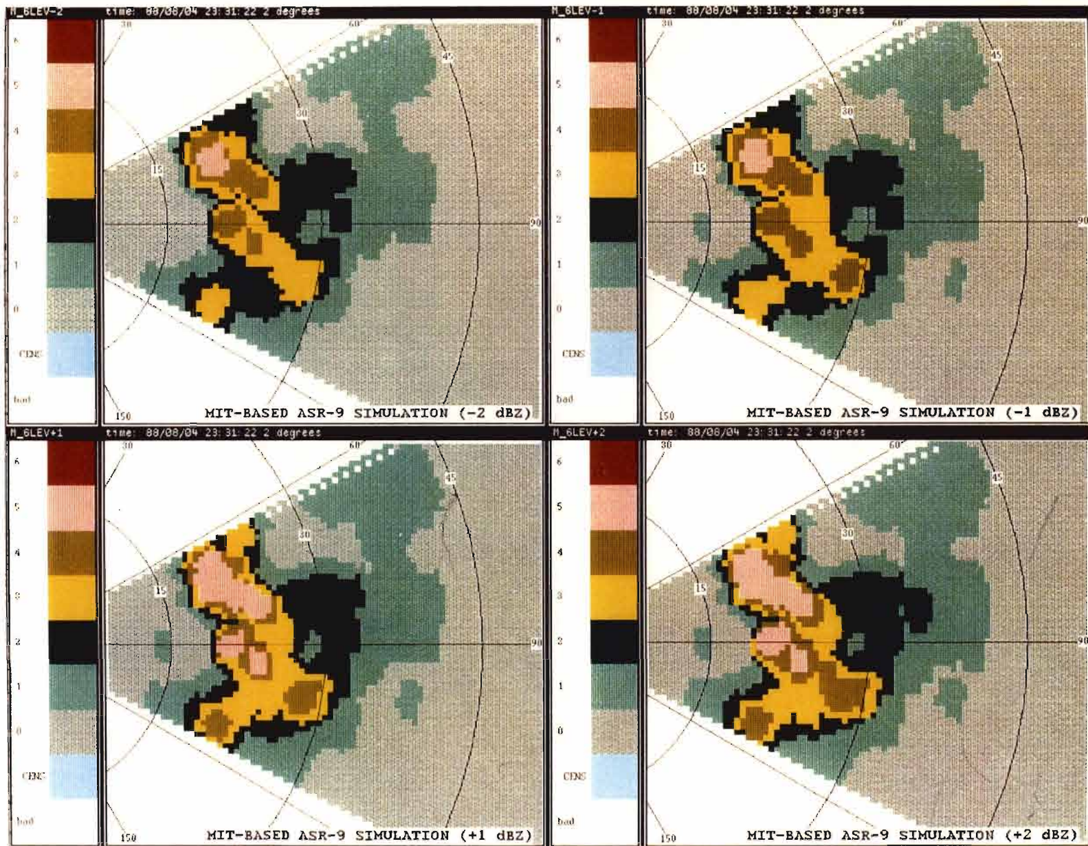
Figure 2-2. Simulation output for convective storm, 4 August 1988 (event 1) for reflectivities offset by (a) -2, (b) -1, (c) +1, and (d) +2 dB. Relatively small reflectivity offsets can have a significant impact on the spatial extent of weather contours reported.
