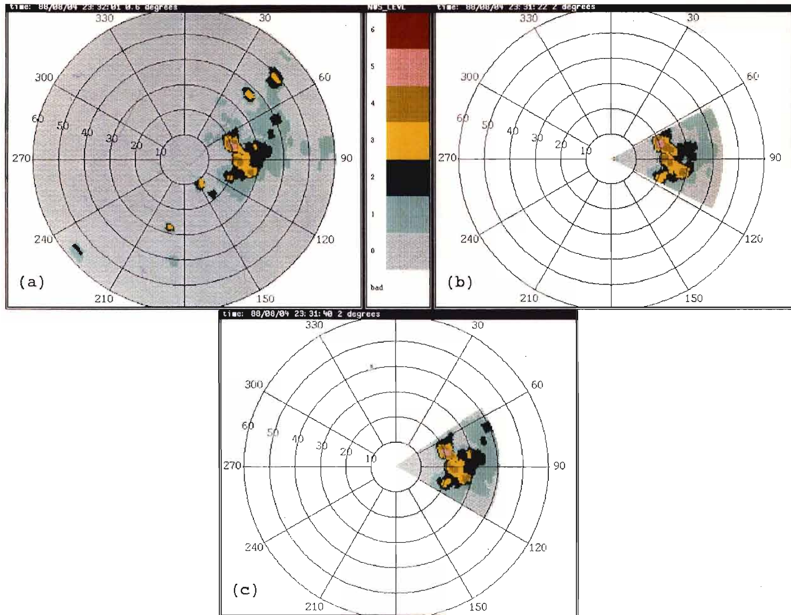
Figure 3-4. Comparison between (a) ASR-9 six-level, (b) simulation, and (c) emulation data, convective storm, 4 August 1988. Inspection indicates excellent agreement among the three data products, with the best agreement between the ASR-9 and FL-3 emulation data.
