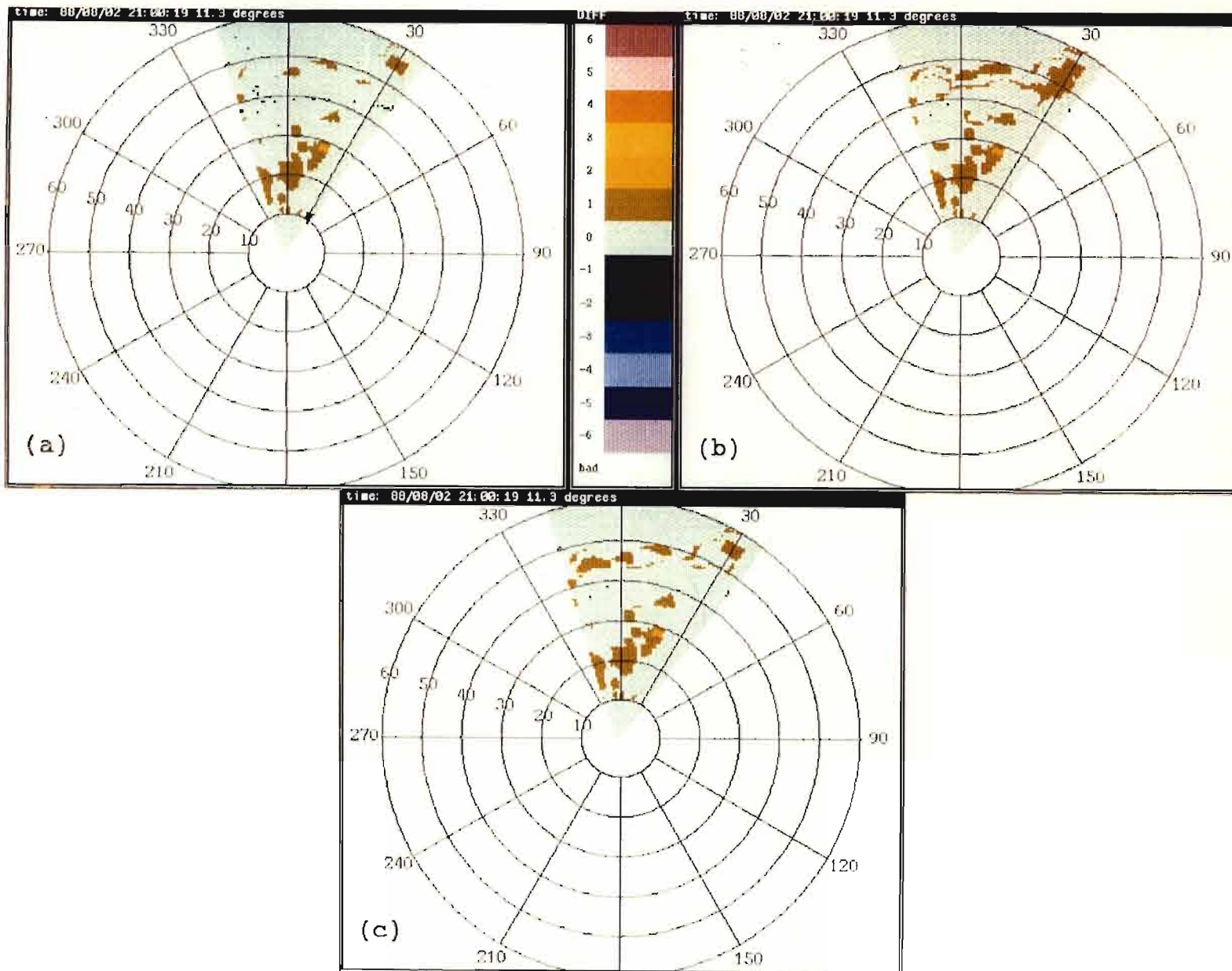
Figure 3-20. Reflectivity difference between ASR-9 two-level and (a) MIT based maximum, (b) average, and (c) horizon-scan data, convective storm, 2 August 1988. Statistics show that the ASR-9 data agree best with the maximum reflectivity data, with less agreement with the horizon-scan and average reflectivity data.
