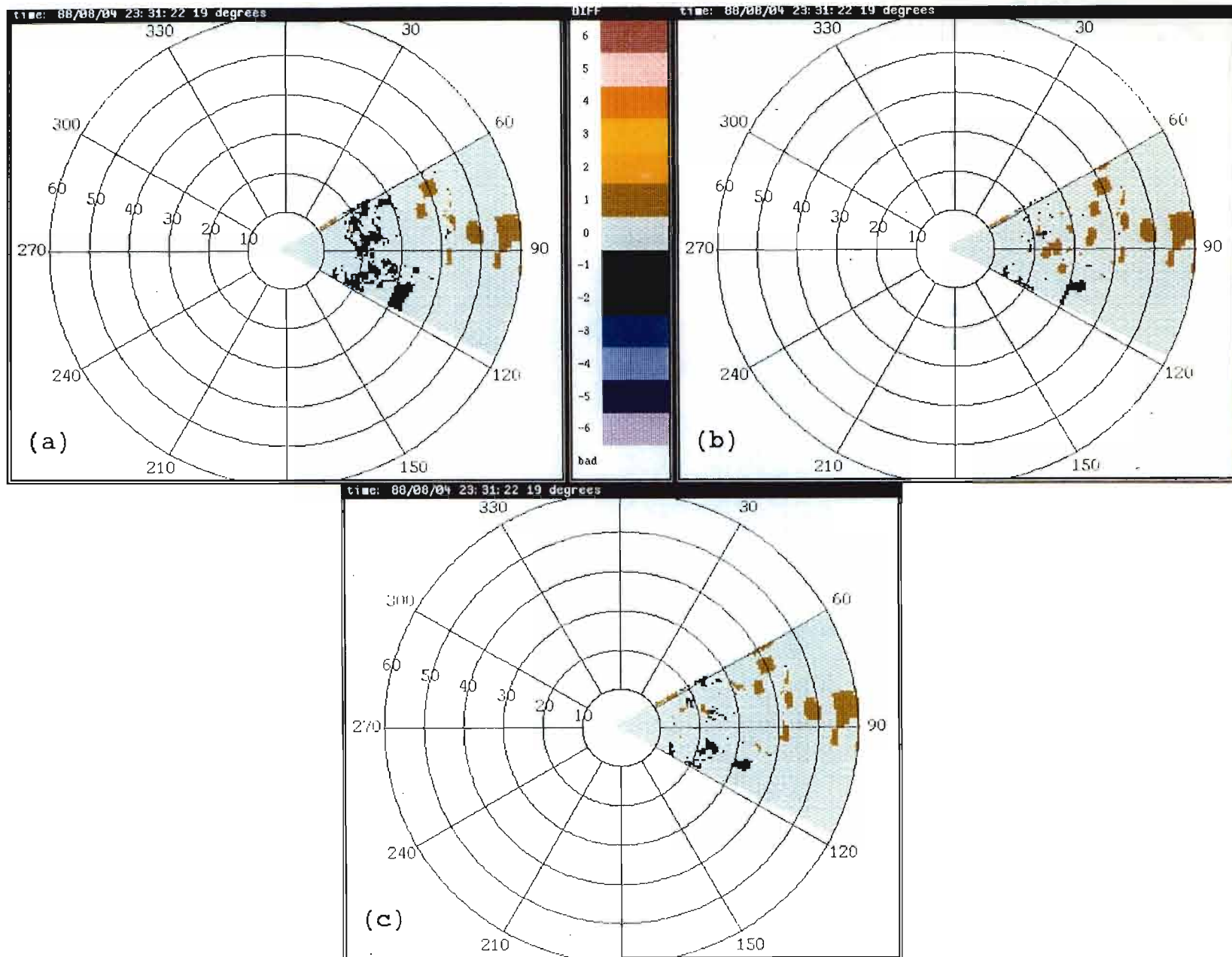
Figure 3-23. Reflectivity difference between ASR-9 six-level and (a) MIT based maximum, (b) average, and (c) horizon-scan data, convective storm, 4 August 1988. Statistics show that the ASR-9 data agree best with the average and horizon-scan reflectivity data, while the maximum data is sometimes two levels higher than the ASR-9 data.
