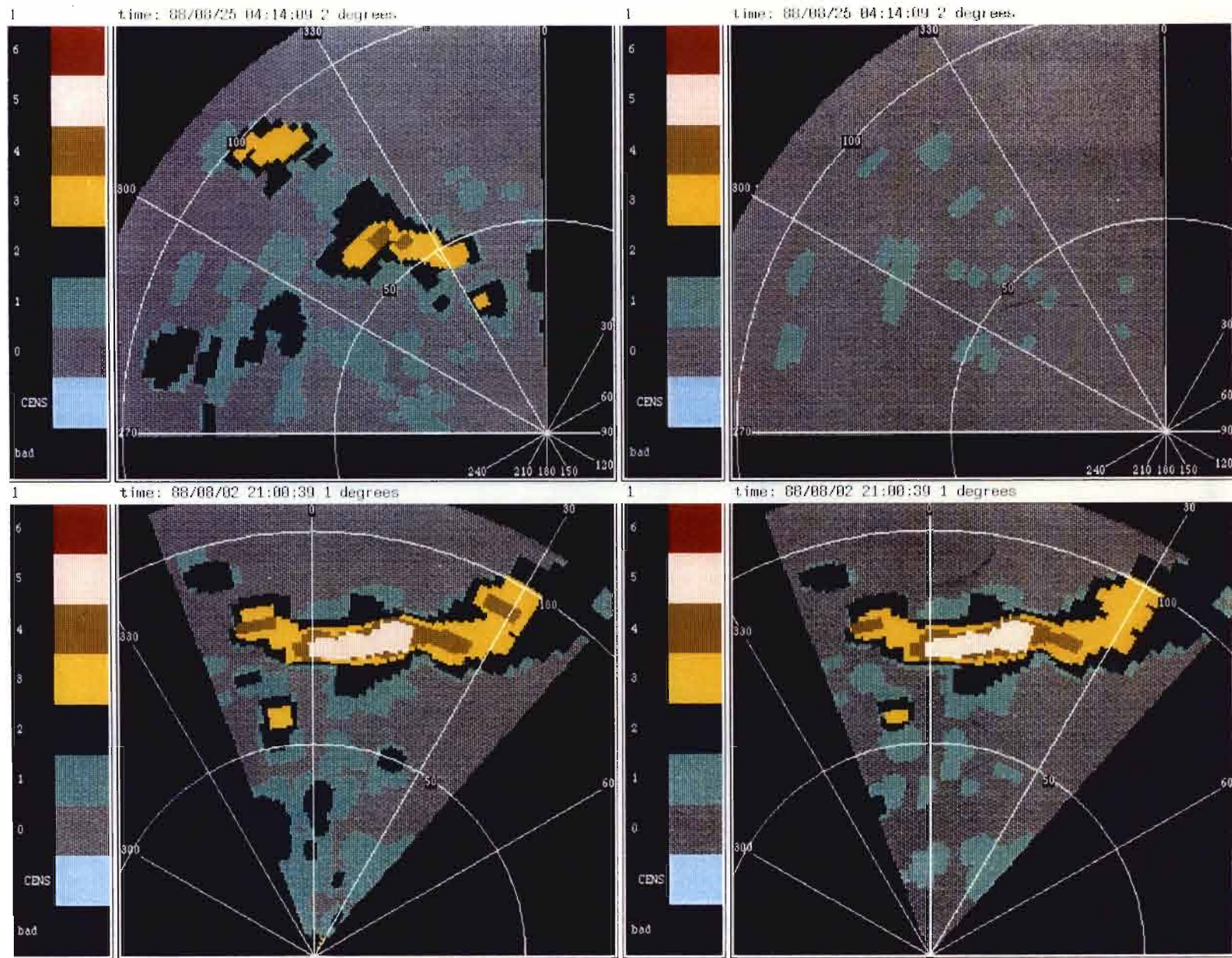
Figure I-6. FL-3 based emulation of ASR-9, showing effect of spectrum width based AP filter on both AP and weather. (a) AP, nominal spatial filter parameters. (b) AP, spectrum width based filter. (c) Weather, nominal spatial filter parameters. (d) Weather, spectrum width based filter. AP is significantly reduced while weather is generally unaltered.
