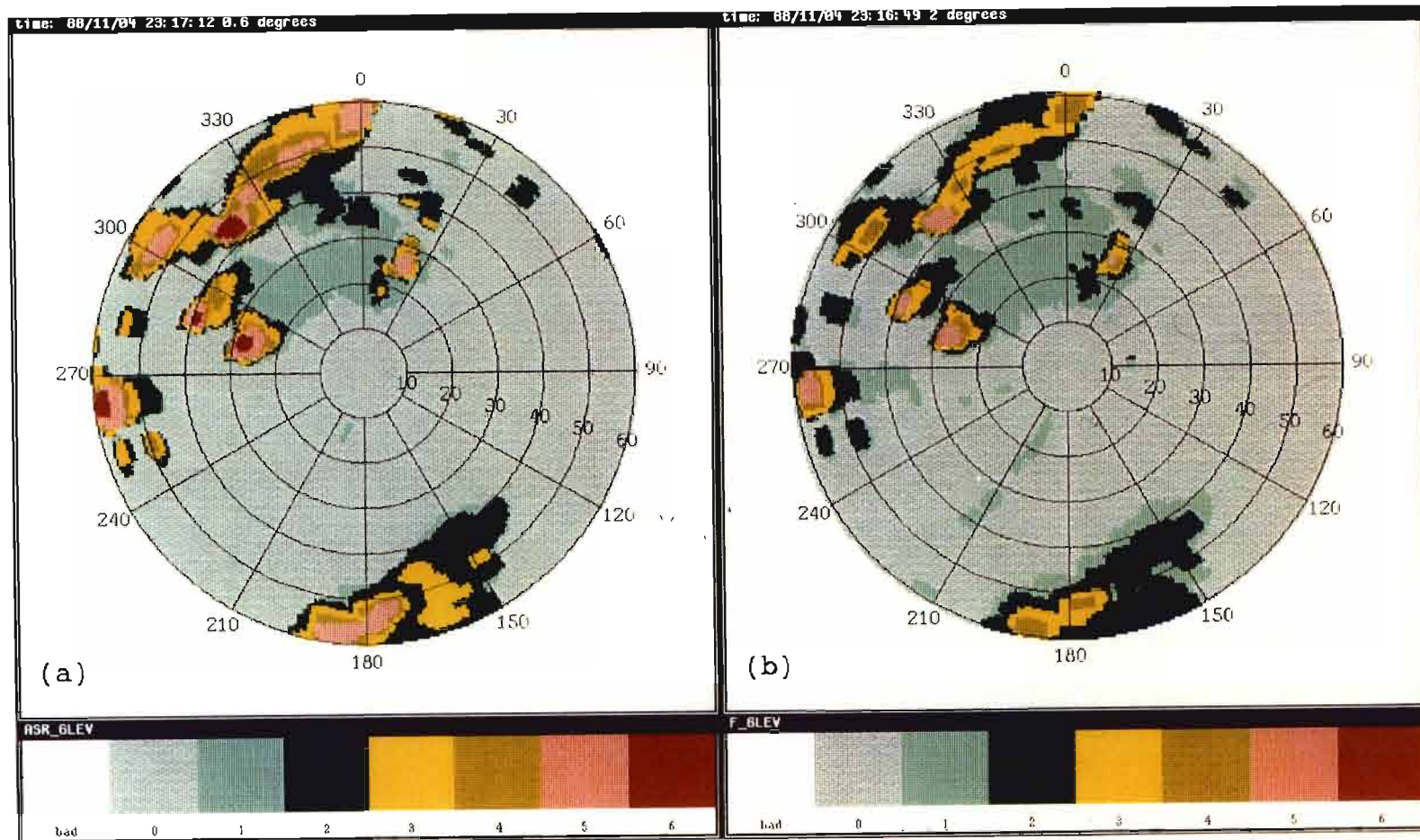
Figure 3-12. Comparison between (a) ASR-9 six-level CP and (b) emulation data, cold front, 4 November 1988. Although the PPIs show good spatial agreement, several of the ASR-9 weather contours are one level higher than the emulation data.
