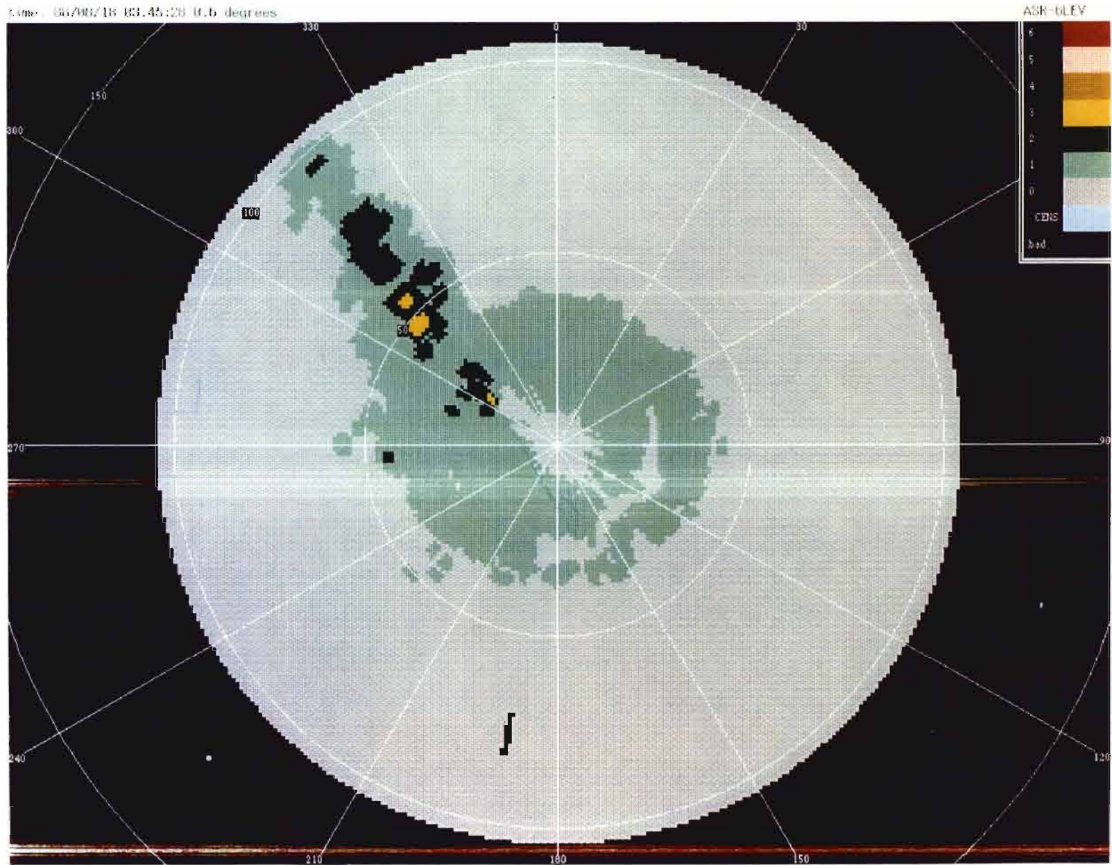
Figure I-1. ASR-9 weather channel six-level output recorded during anomalous propagation event on 18 August 1988.
