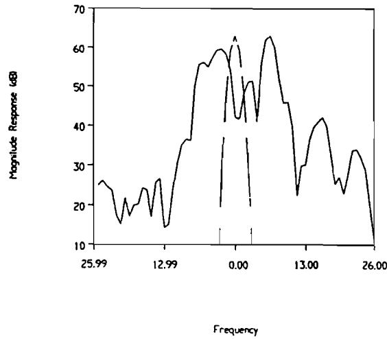
Figure I-4. Typical spectral characteristics of clutter, AP, and zero mean velocity weather; (a) Clutter spectrum, (b) AP spectrum, (c) Weather spectrum.
