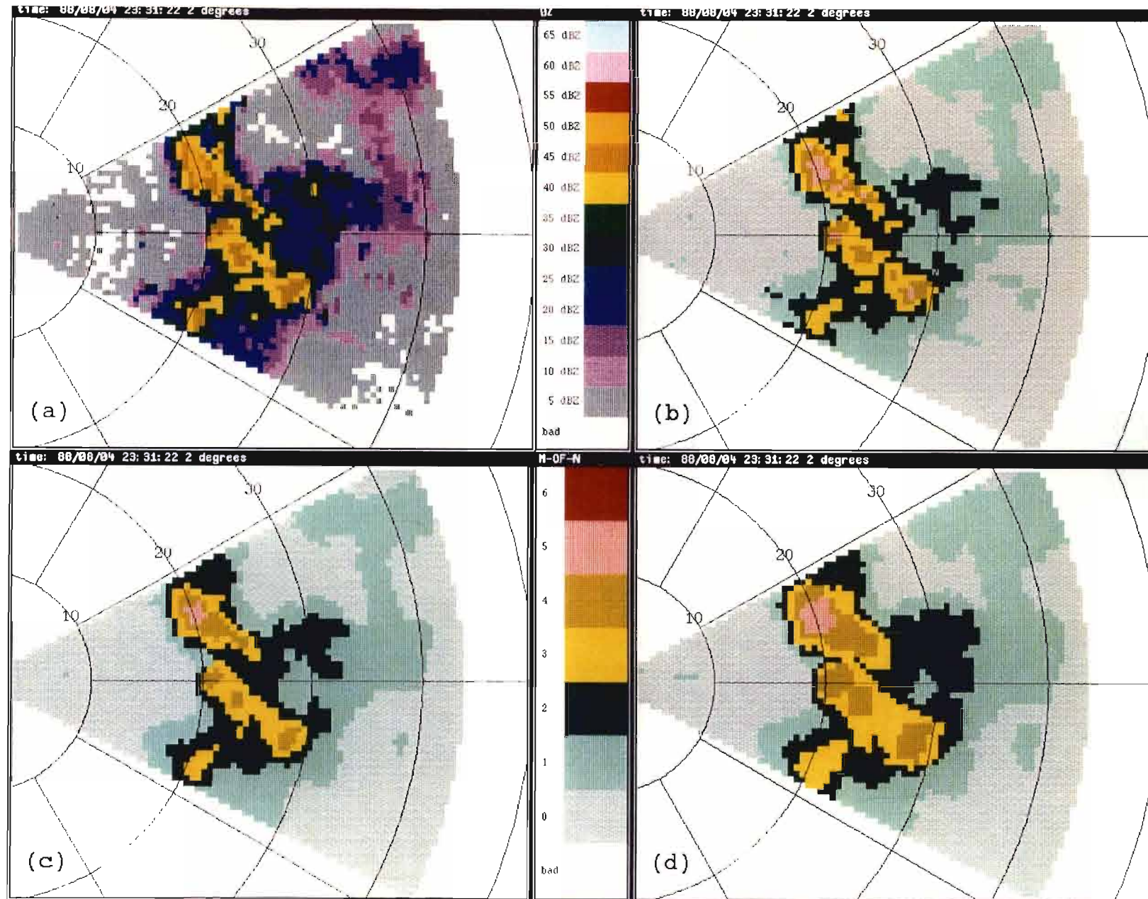
Figure C-7. Output of the ASR-9 weather channel processor simulation after: (a) Fan beam integration of MIT reflectivity data, (b) M-of-N processor, (c) First spatial filter, (d) Second spatial filter (final product)
