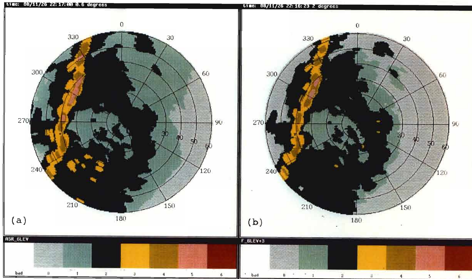
Figure 3-16. Comparison between (a) ASR-9 six-level LP and (b) emulation data increased by 3 dB, squall line, 26 November 1988. Inspection indicates much better agreement between the two radars when emulation data is increased by 3 dB.
