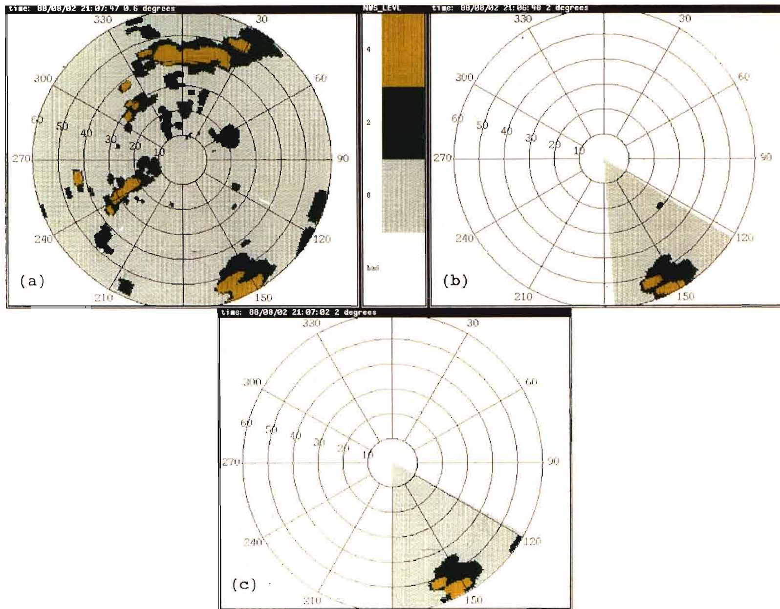
Figure 3-2. Comparison between (a) ASR-9 two-level, (b) simulation, and (c) emulation data, convective storm, 2 August 1988. Inspection indicates good agreement among the three data products.
