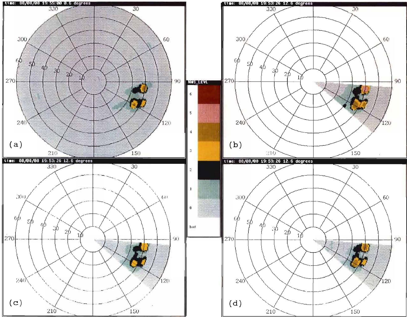
Figure 3-25. Comparison between (a) ASR-9 six-level and (b) MIT based maximum, (c) average, and (d) horizon-scan data, convective storm, 8 August 1988. Inspection indicates that the ASR-9 data agree best with the average and horizon-scan reflectivity data, suggesting that the ASR-9 beam fill correction storm model is not appropriate for this storm event.
