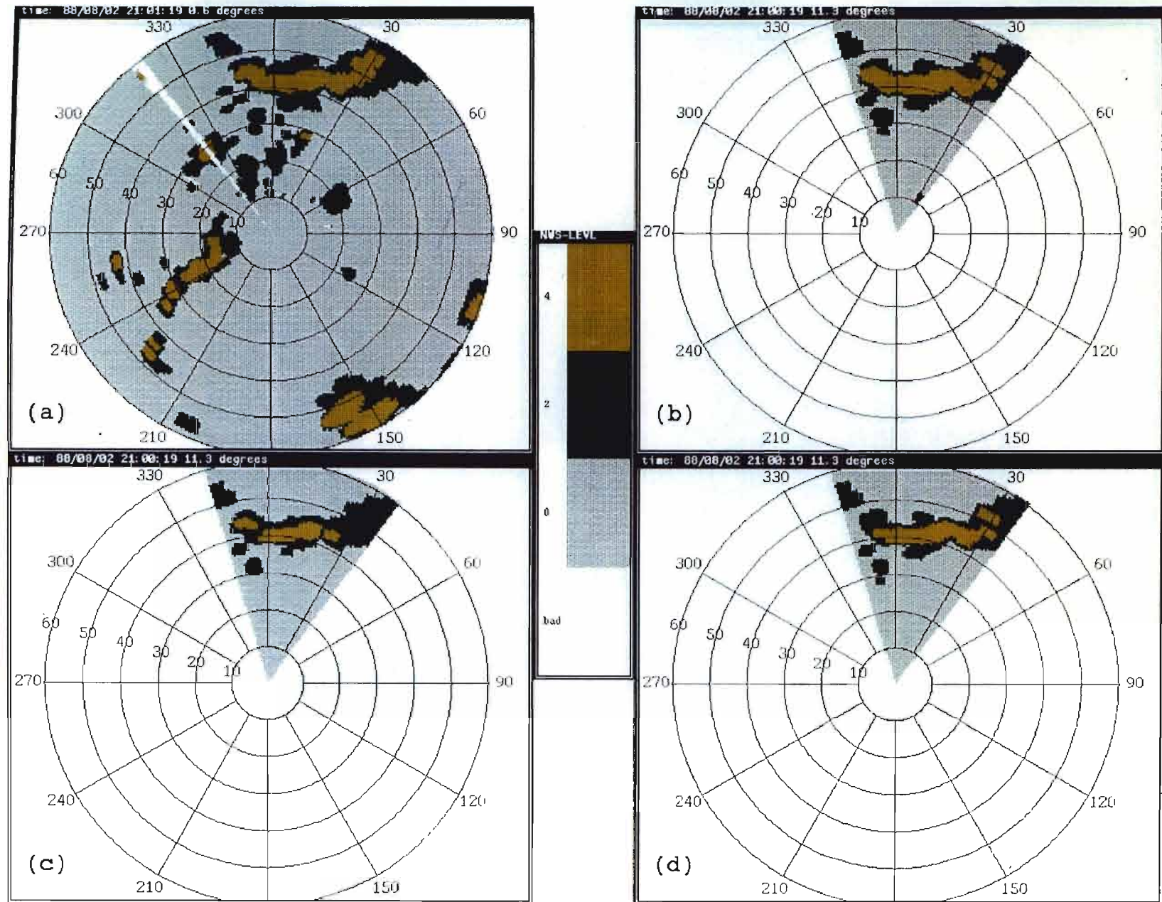
Figure 3-19. Comparison between (a) ASR-9 two-level and (b) MIT based maximum, (c) average, and (d) horizon-scan data, convective storm, 2 August 1988. Inspection indicates that the ASR-9 data agree best with the maximum reflectivity data, suggesting that the ASR-9 beamfill correction storm model is appropriate for this storm event.
