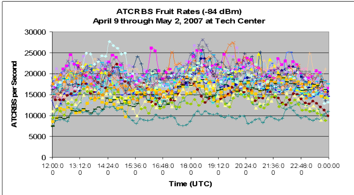
Figure A-8. WJHTC ATRBS Fruit Measured on the Ground
