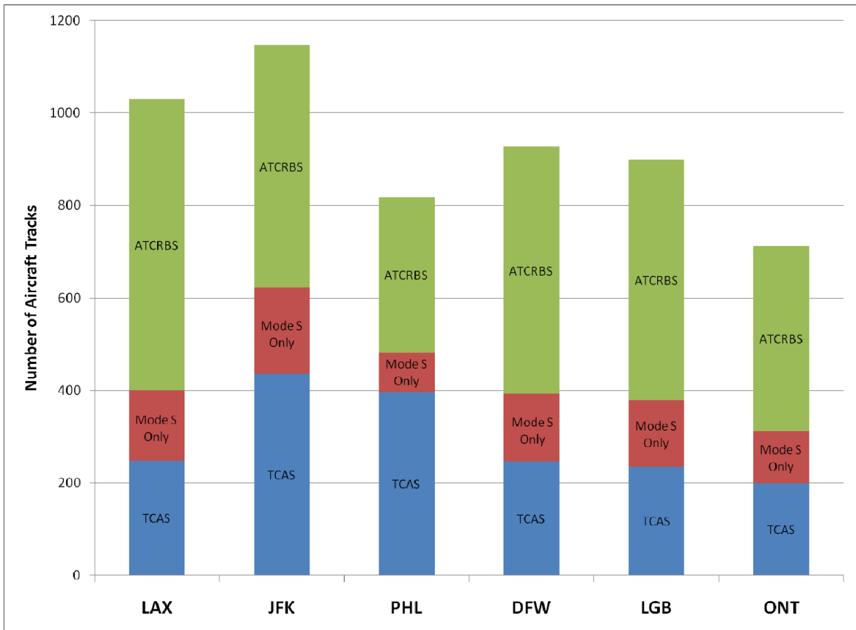
Figure 7. Aircraft Track Equipages
