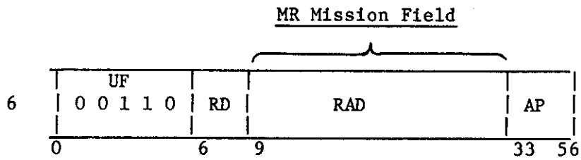
(a) RBX Squitter Format
