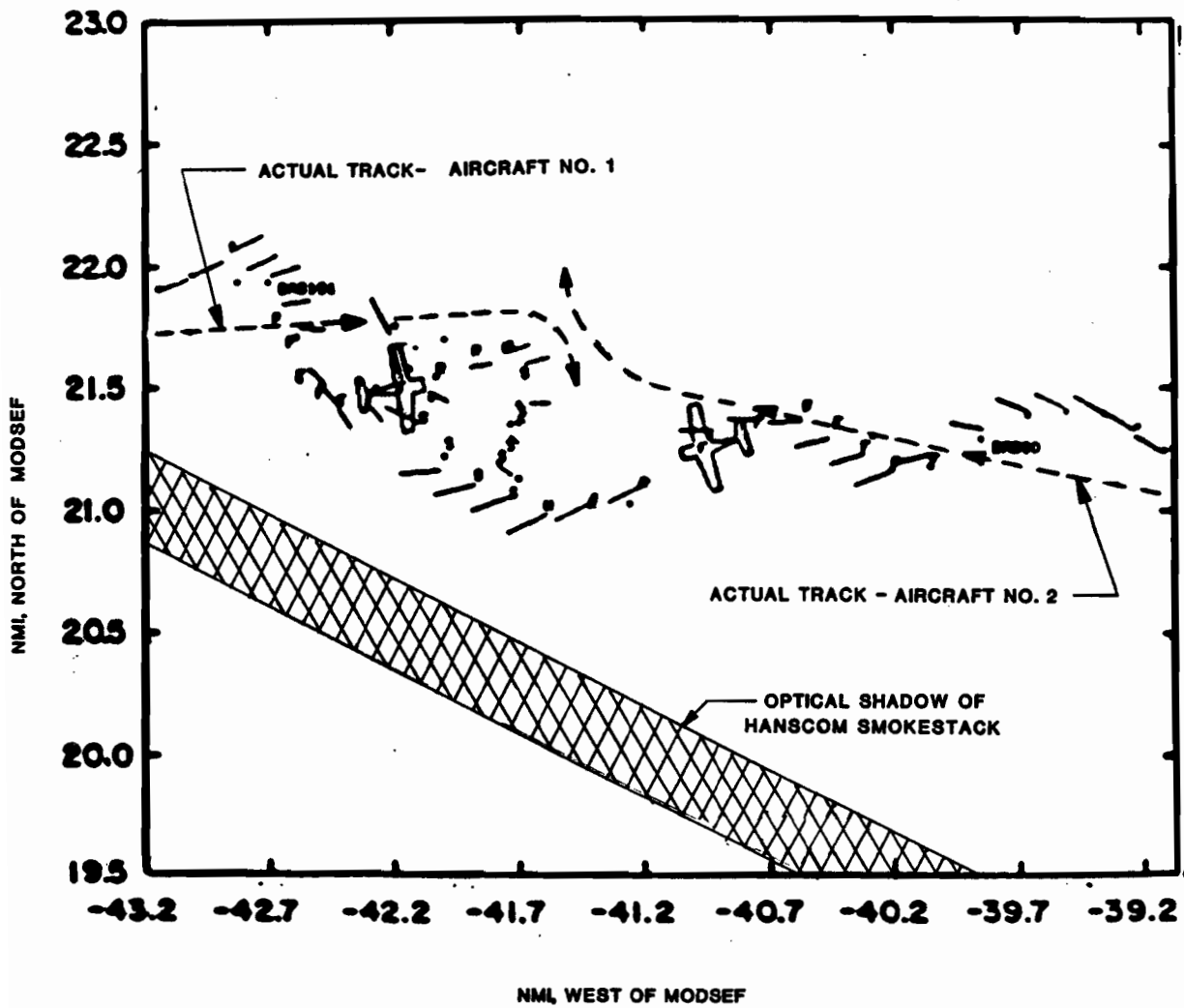
Fig. 6. Plot of an Encounter Exercise Showing the Effect of Diffraction From a Vertical Obstacle on Aircraft Surveillance.
