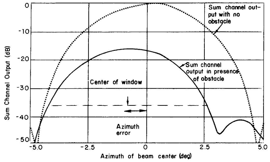
Fig. A-3. Effect of shadow of Prudential building on sum channel output.
