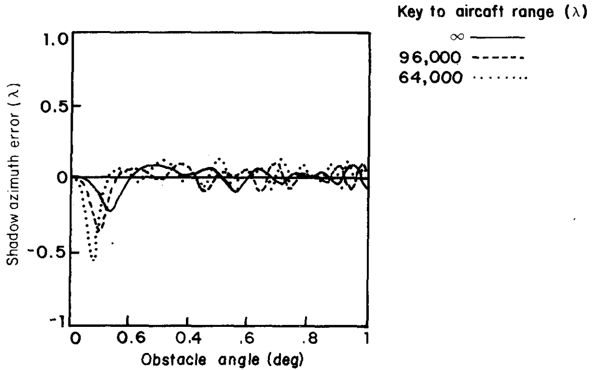
Fig. 3-6. Shadow azimuth error vs obstacle azimuth for an aircraft at 3 ranges; obstacle is at 32,000 λ range, is 140 λ wide.
