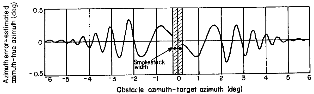
Fig. 1-2. Azimuth estimation error vs obstacle position. Obstacle, which corresponds to Hanscom Field smokestack as seen from DABSEF, is 10 feet wide and at a 1500-foot range ( \lambda = 1 ft).
