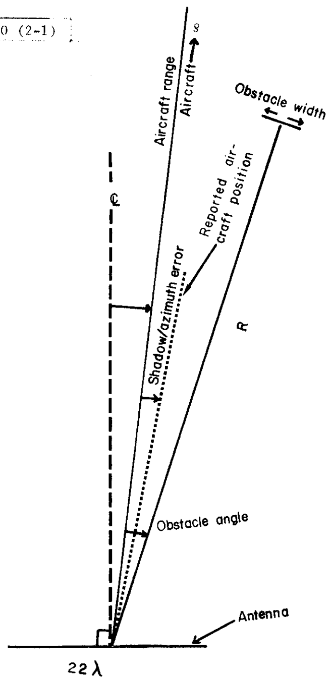
Fig. 2-1. Parameters used in study of shadow azimuth error.
