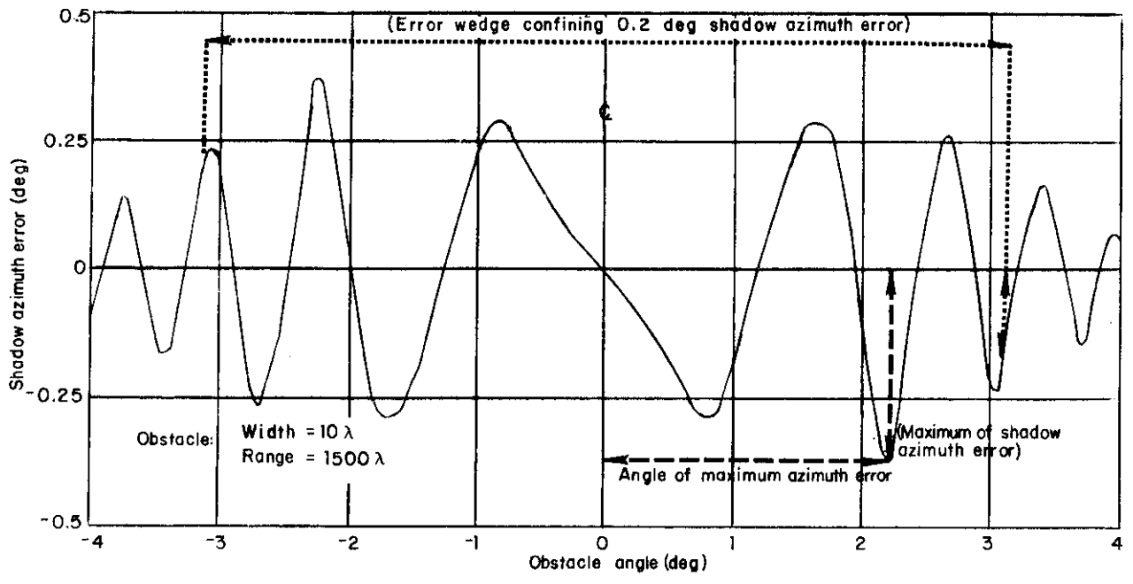
Fig. 3-1. Shadow azimuth error vs obstacle angle (illustration of key features of spatial distribution of the error).
