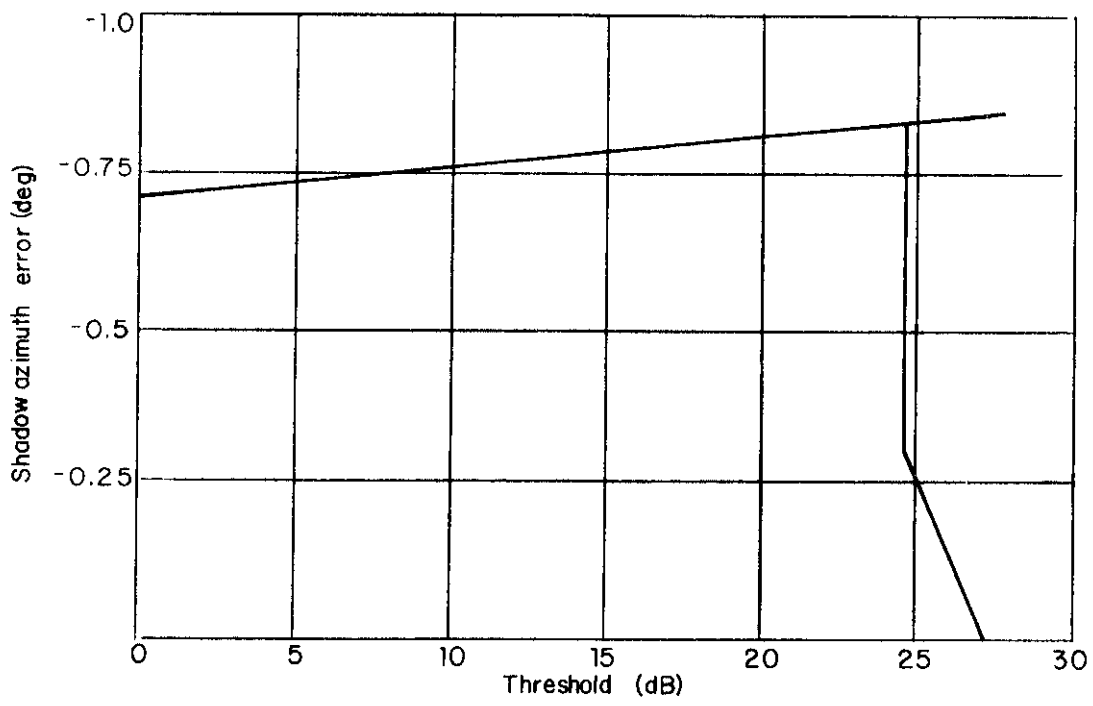
Fig. 4-4. Sliding window azimuth error vs threshold; obstacle is Prudential building.
