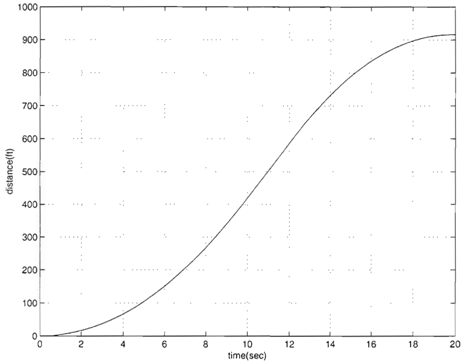
Figure 56. Distance vs. time for nominal takeoff rejected at t_{evade} = 10 seconds.
