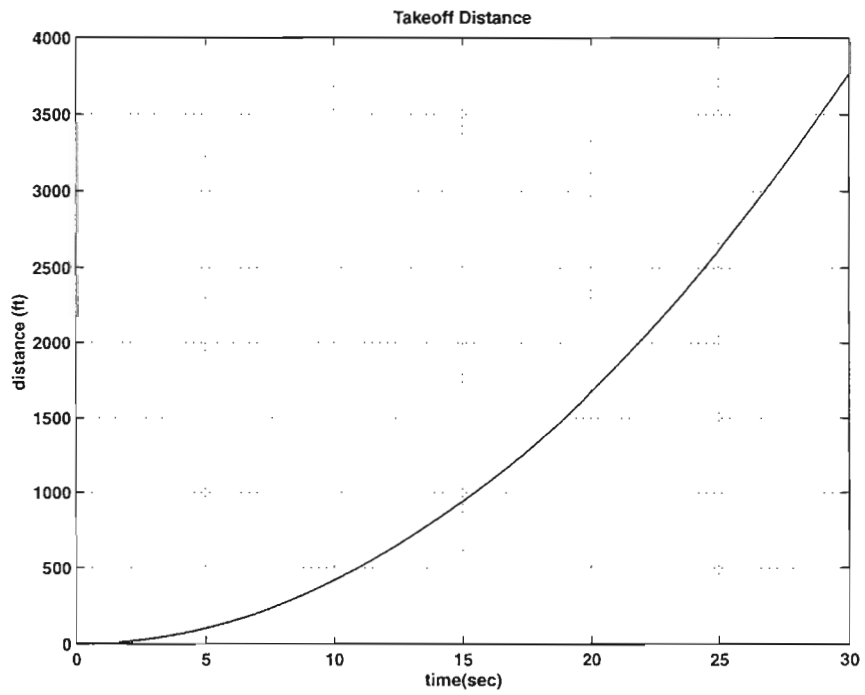
Figure 30. Nominal takeoff aircraft takeoff distance.
