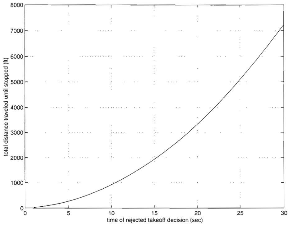
Figure 57. Total runway used versus t_{evade} , time evasive action began for the nominal takeoff profile.
