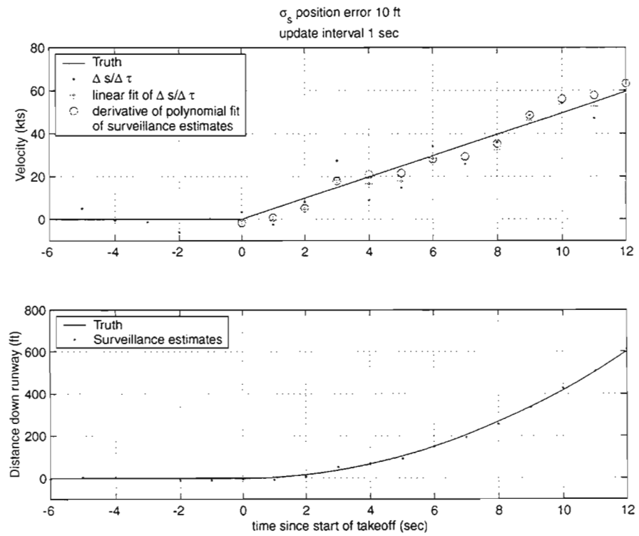
Figure 40. Monte Carlo trial of velocity estimates with \sigma_s = 10 feet and \Delta\tau = 1 seconds.
