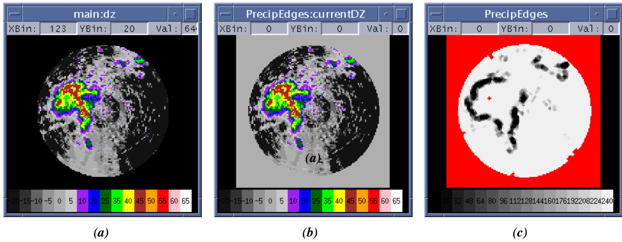
Figure 41. Example computation of the precipitation edges interest image ( PrecipEdges ). (a) Reflectivity image . (b) Modified copy of reflectivity image after setting outer edge values to 45 (2.5 dBZ) . (c) Final PrecipEdges interest image after FTC and inverting the interest scores to produce the "negative" interest image . Data are from 07/21/99 21:16:23 GMT at Austin, TX
