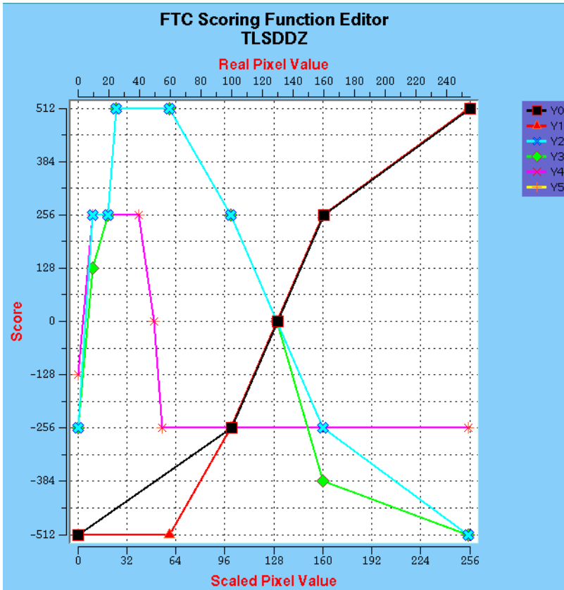
Kernel #1: SD
