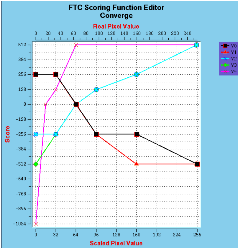
Kernel #1: conv
