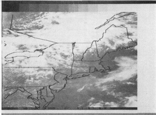
Fig. 3-12: VISIBLE SATELLITE IMAGE - 21 JULY 83, 2:00 P.M. (1800 GMT)
