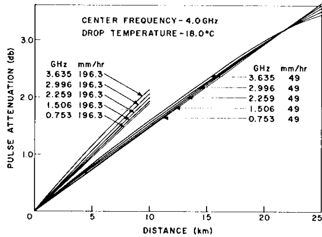
Fig. 8. Pulse attenuation vs. distance.
