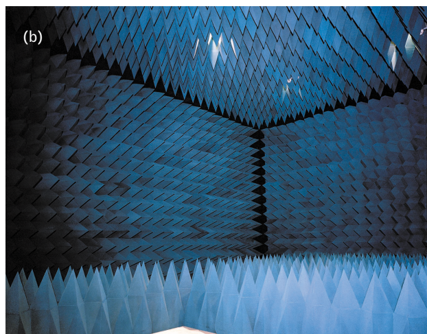
FIGURE 17. (a) Lincoln Laboratory's ground-test facility for adaptive phased-array antenna evaluation in space-based-radar applications. (b) This facility has interior walls covered with radiation-absorbing material, which enables full-scale real-time testing of radar capability at a test distance of approximately one aperture diameter.
