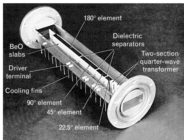
FIGURE 12. A Westinghouse production model of a four-bit C-band ferrite phase shifter, with the waveguide cover removed.
