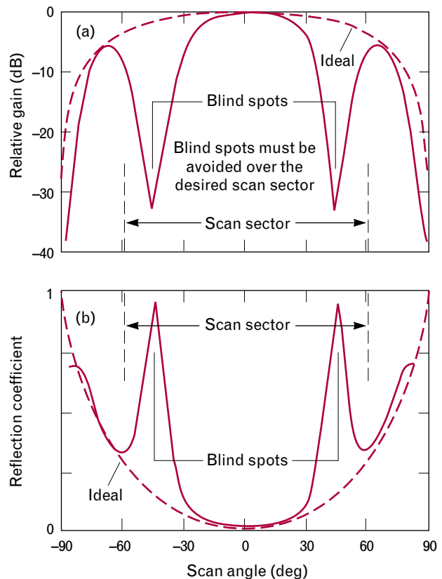
FIGURE 4. Conceptual images of blind-spot occurrence in a phased-array antenna. These results are typical of an array designed without regard for array mutual-coupling effects. A blind spot occurs when either (a) the array element pattern has a null or (b) the element reflection coefficient has unity magnitude. The blind spot is often caused by array mutual coupling, which tends to direct the radiation in the plane of the array as a surface wave, rather than as a wave propagating away from the array. Careful design of the array element shape, size, and spacing can prevent the occurrence of blind spots.
