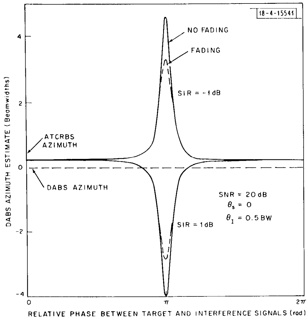
Fig. 3. Azimuth estimate in the presence of interference.
