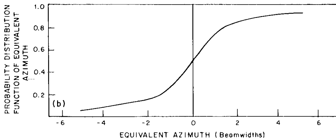
Fig. 1b. Probability distribution function of equivalent azimuth.
