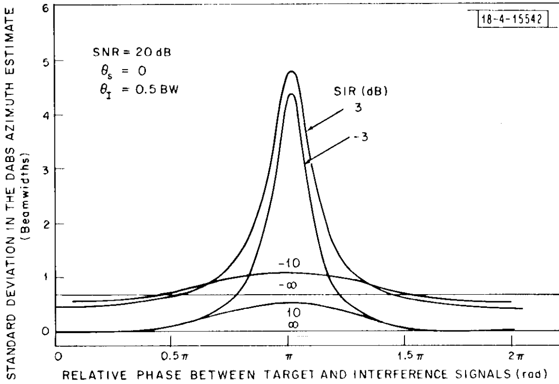
Fig. 4. Variance of the azimuth estimate in the presence of interference.
