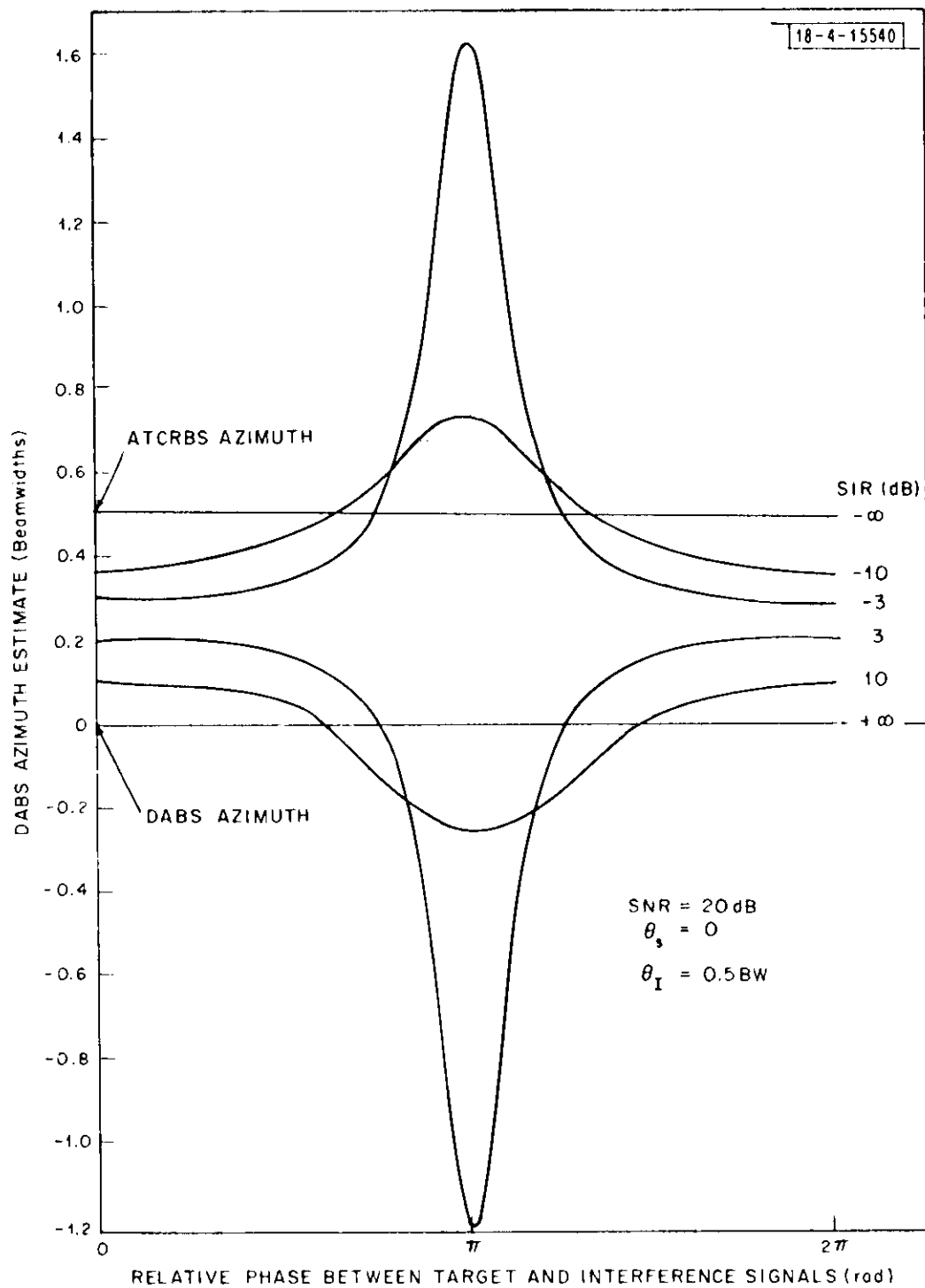
Fig. 2. Azimuth estimate in the presence of interference.
