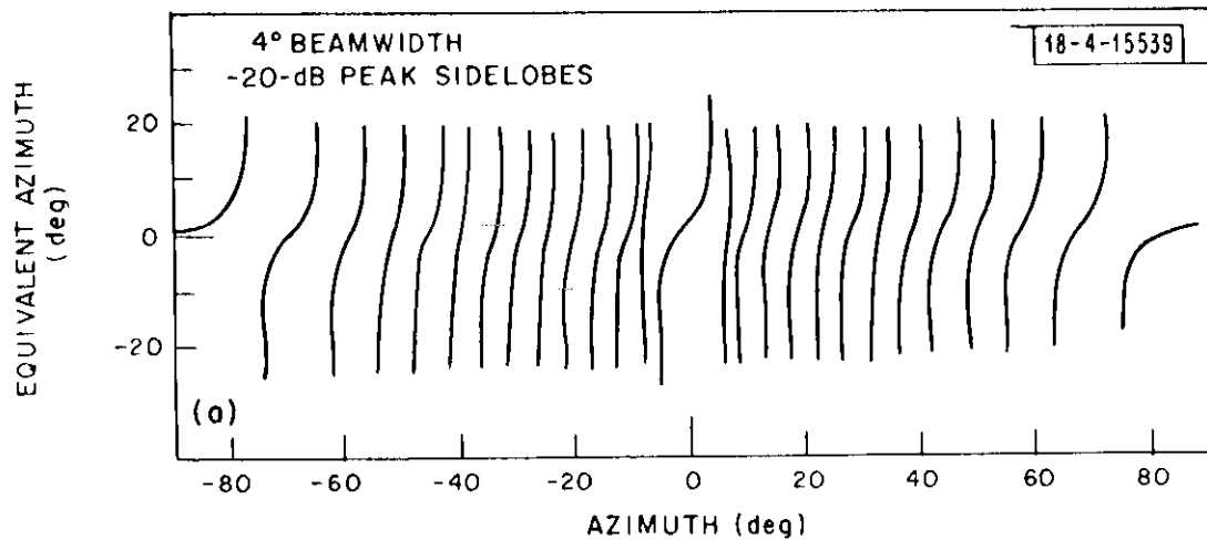
Fig. 1a. Equivalent azimuth using the monopulse function.
