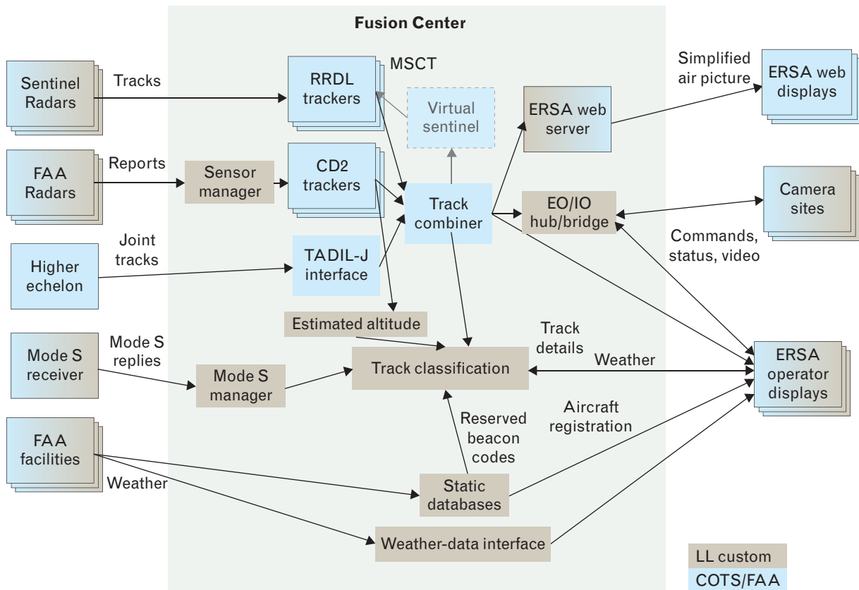
FIGURE 10. Fusion-center data flow. Data are initially handled by the sensor manager. The track classification component evaluates the sensor, Mode S, and static databases, determines threat levels, and presents the data to the operators.
