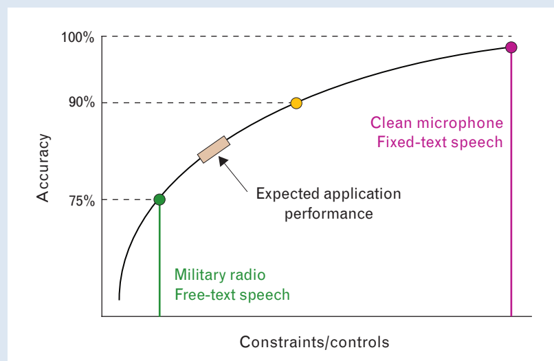
FIGURE B. Nominal trade-off of speaker-authentication accuracy versus data and application constraints and controls.
