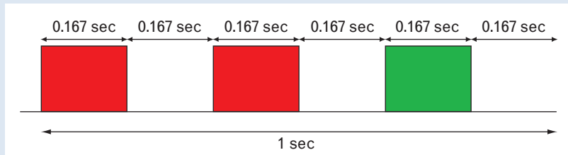
FIGURE B. Pulsed-signal waveform for VWS. This signal ordering is distinct from all other airport signals that pilots receive during routine operations.
