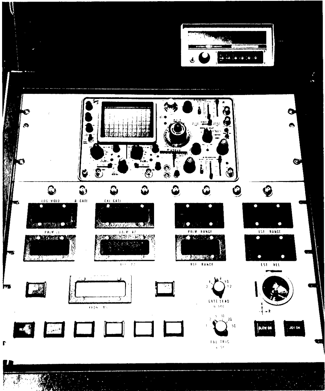
Fig. 28. Operator's console.
