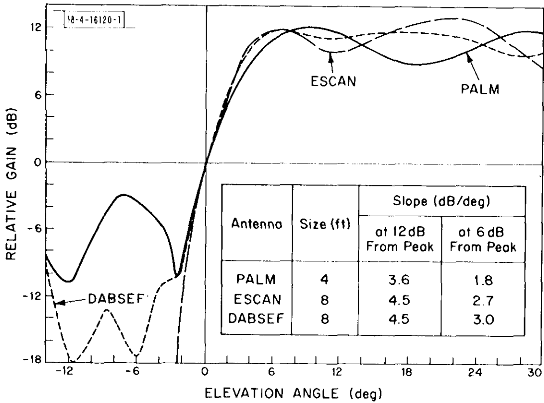
Fig. 6. Measured antenna patterns at 1090 MHz.
