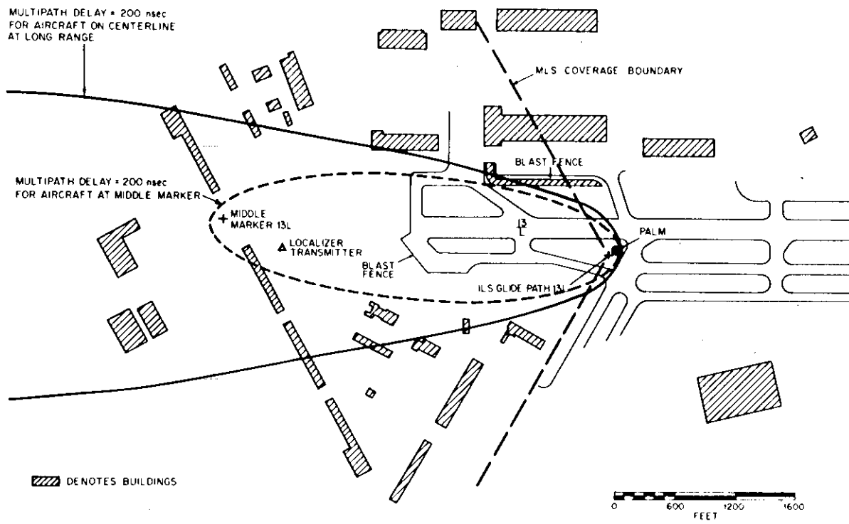
Fig. 8. Time delay discrimination at JFK runway 13L.
