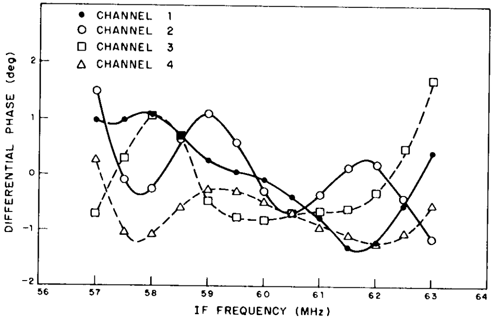
Fig. 26. Channel differential amplitude and phase response.
