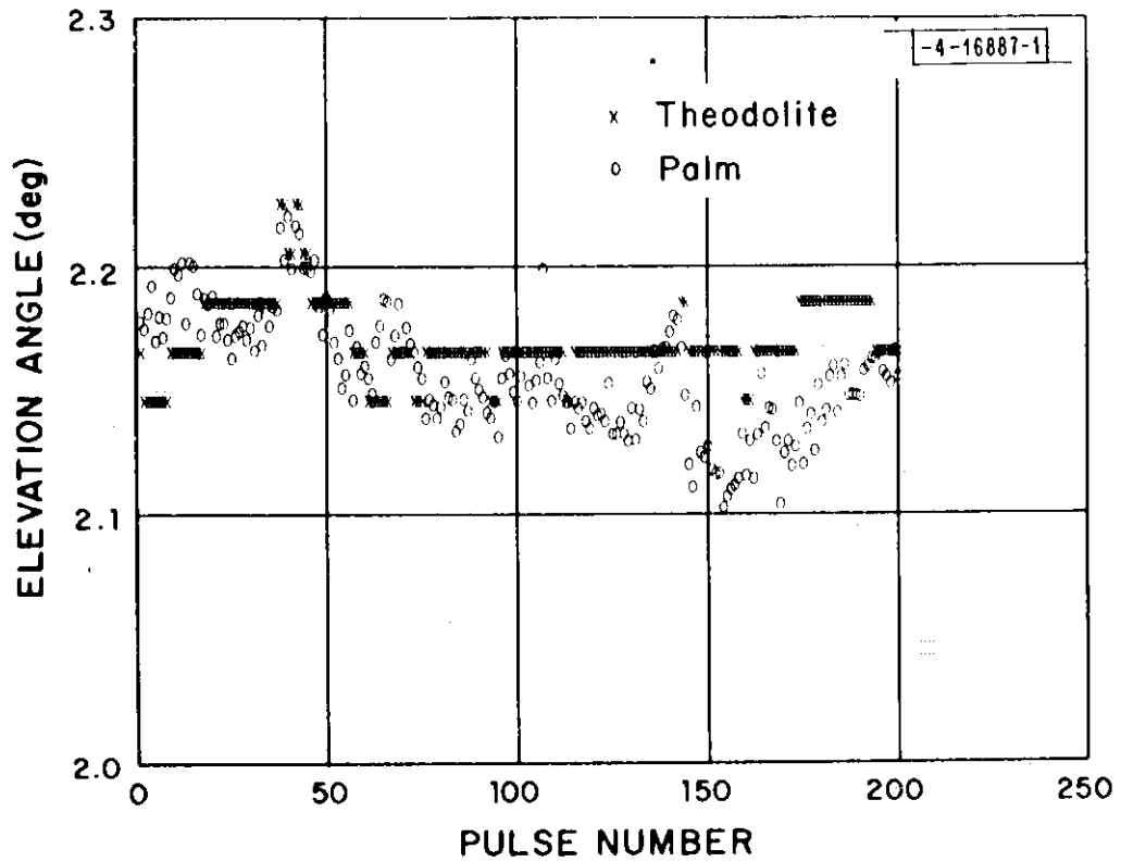
Fig. 34. Elevation angle estimates versus pulse number (time).
