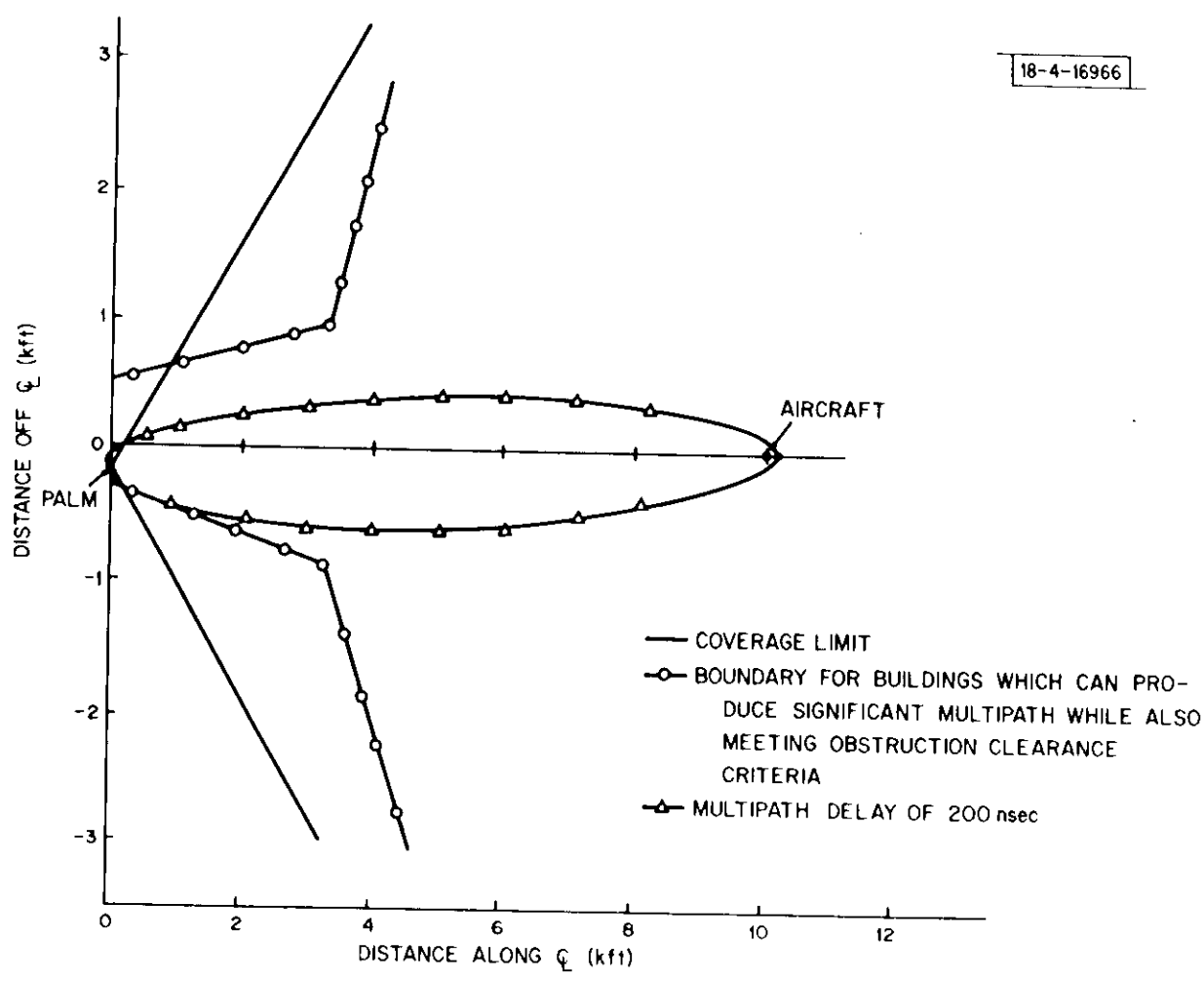
PALM time delay discrimination against theoretically possible hangar elevation multipath threats.
