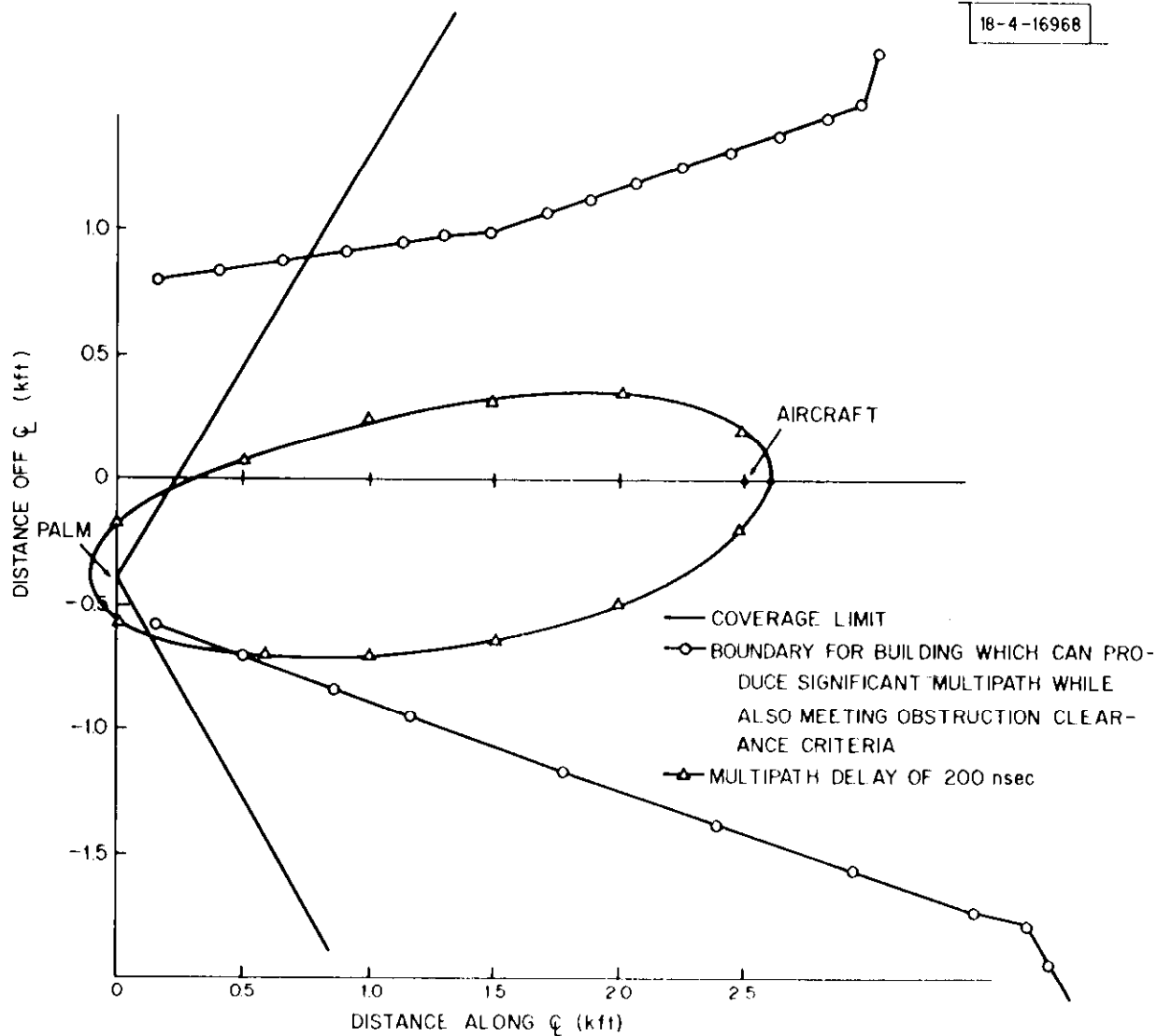
PALM time delay discrimination against theoretically possible hangar elevation multipath threats.
