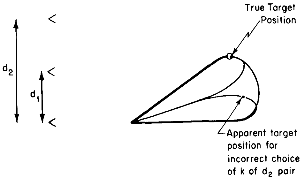
Fig. 14. Ambiguity resolution.
