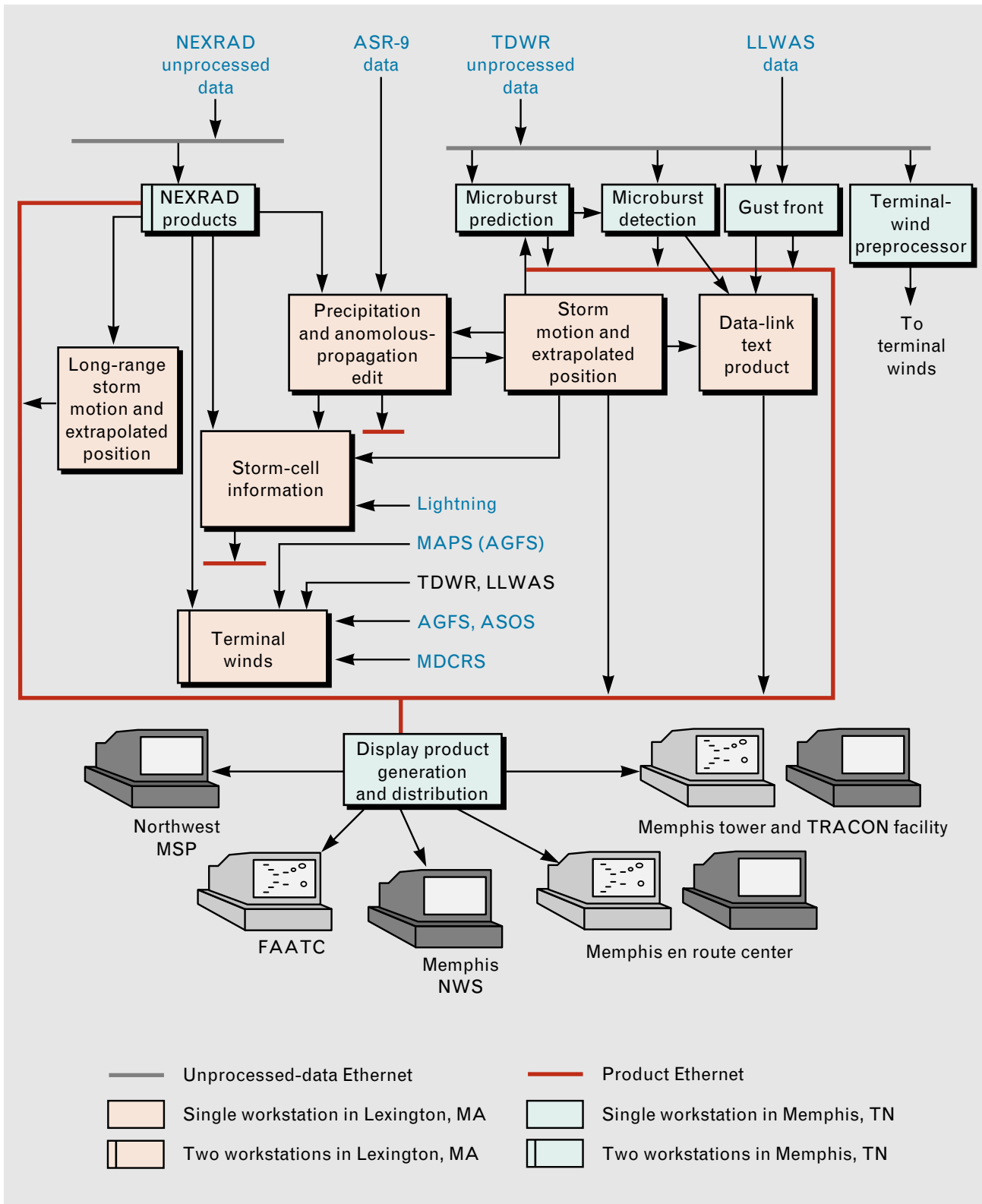
FIGURE 6. Real-time system architecture used for demonstrating ITWS in Memphis, Tennessee, in 1994. Green and red boxes represent workstations that were resident in Memphis and Lexington, Massachusetts, respectively. Data sources are indicated in blue.
