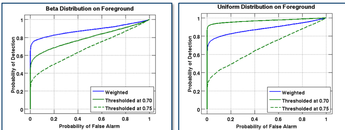
Figure 13. Detection performance when thresholding weighted edges.
