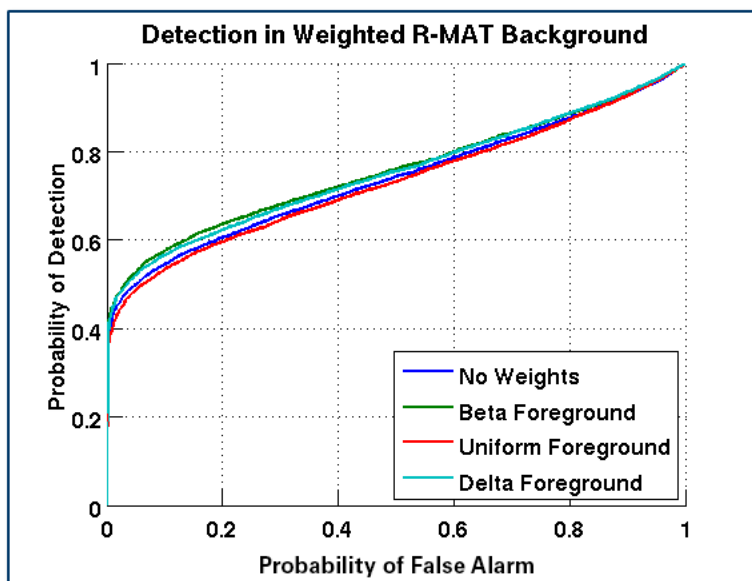
Figure 12. Detection performance with weighted edges.
