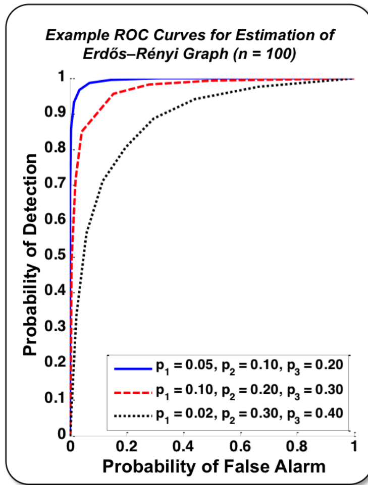
Figure 7. Recovery of an Erdős-Rényi random graph with uniform edge errors. The simple structure of the problem yields a decision rule based on which edges exist in each of the three observations. Edge error probabilities are shown in the legend.
