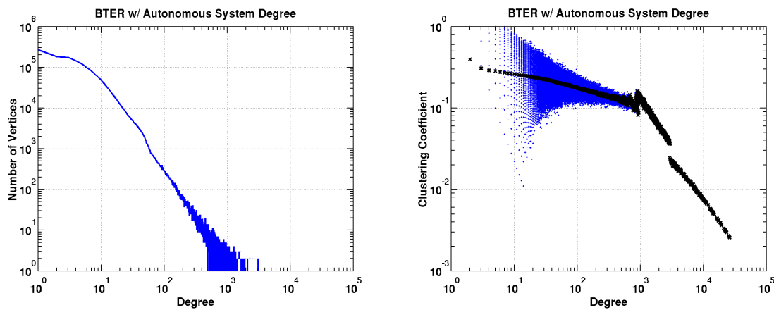
Figure A.3. Vertex statistics of the BTER simulation (with Skitter degree distribution) dataset: degree (left) and clustering coefficient (right). Eigentrality and PageRank were not computed at the time of completion of this report.
