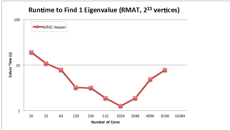
Figure 17. Strong scaling of parallel eigendecomposition. Computation time per core increases after 1024 cores, likely due to communication overhead.
