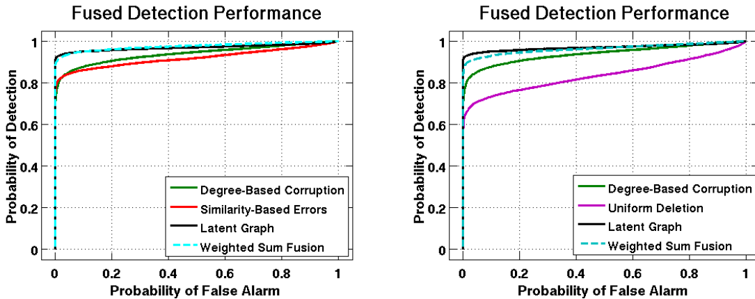
Figure 10. More difficult cases of multi-observation fusion. A graph with greater degree-based corruption is fused with a graph with similarity-based errors (left) and uniform edge removal (right). Fusion with the graph with similarity-based errors recovers equal detection performance to the latent graph, while fusion with the graph with deleted edges yields a small gap in performance.
