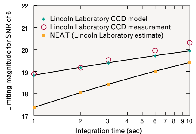
FIGURE 6. Limiting magnitude for a signal-to-noise (SNR) ratio of 6 as a function of integration time for the Lincoln Laboratory CCD and the Near-Earth Asteroid Tracking (NEAT) system. For a specified integration time, the Lincoln Laboratory CCD system detects fainter asteroids having higher magnitudes.
