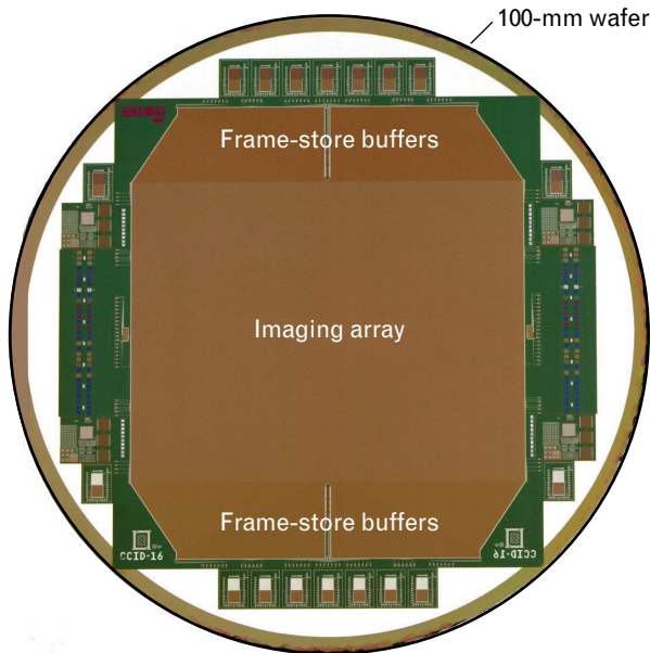
FIGURE 5. Five-million-pixel Lincoln Laboratory CCD chip. This chip is constructed by using a back-illumination process and features a 2560 \times 1960 -pixel focal-plane array. Four frame-store buffers hold an image after integration, allowing the active imaging array to conduct the next integration while the current image is read from the frame-store buffers.
