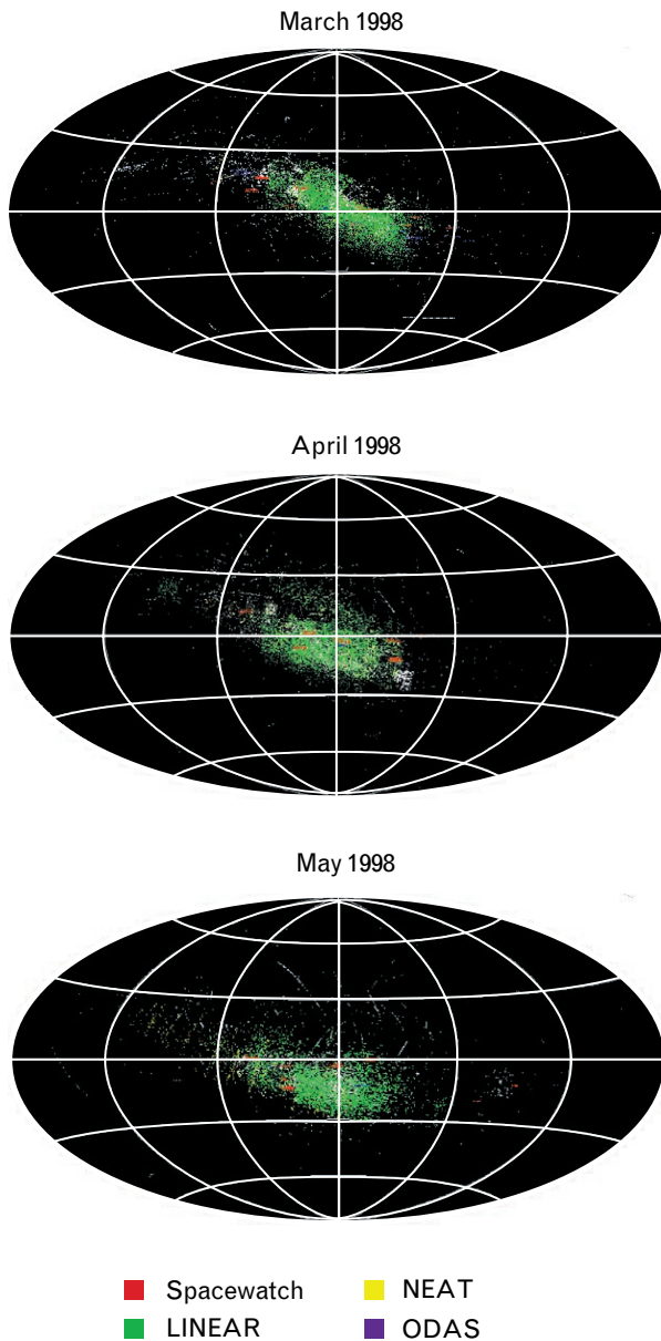
FIGURE 13. MPC sky plots showing detections of asteroids reported by the major search programs Spacewatch, LINEAR, NEAT, and ODAS (a joint effort between the Observatoire de la Côte D'Azur in Nice, France, and the Institute of Planetary Exploration in Berlin-Adlershof, Germany). The LINEAR program outperformed other search programs during the three-month period.
