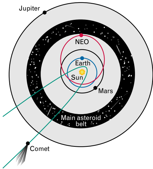
FIGURE 1. Inner solar system showing the orbits of asteroids and comets in the main asteroid belt between Mars and Jupiter (relative orbits drawn to scale). Most asteroids in the main belt have nearly circular orbits and so do not pose a threat to Earth. Asteroids with highly elliptical orbits that cross or approach Earth's orbit are called near-Earth objects (NEOs).
