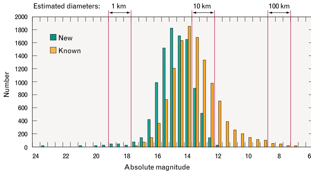
FIGURE 12. Histogram of asteroids detected by LINEAR through 1997, including new discoveries and known objects. The peak of the population discovered by LINEAR is approximately two visual magnitudes fainter than the peak for the known population.
