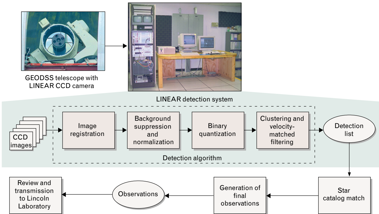
FIGURE 7. Process flow at the Experimental Test Site (ETS) for the LINEAR detection system, which acquires and processes a series of CCD images of the sky to detect moving objects. The detection list is matched against a star catalog to produce a set of final NEO observations, which are then sent to Lincoln Laboratory.
