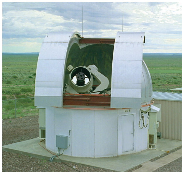
FIGURE 4. ETS telescope used to test the Lincoln Laboratory large-format CCD camera and search for asteroids. The telescope is identical to an operational GEODSS telescope.
