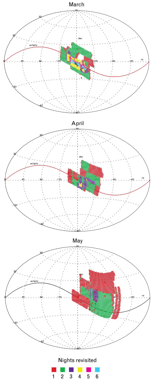
FIGURE 10. Equatorial plot of the sky covered by LINEAR during opposition in March, April, and May of 1998. The plots are color coded to indicate the number of times the sky area was covered during the month.
