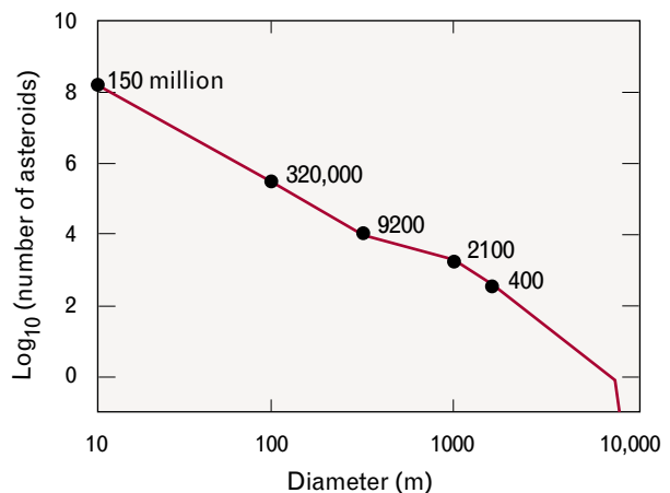
FIGURE 2. Estimated population of Earth-crossing asteroids with diameters above a given size. About 10% of asteroids with diameters larger than 1 km are known.
