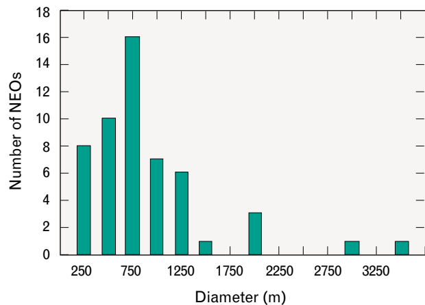
FIGURE 11. Histogram of the size distribution of NEOs discovered by LINEAR through March 1998.
