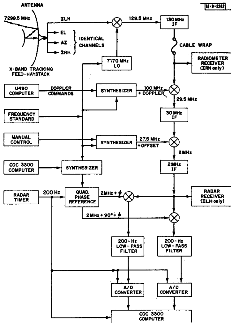
Fig.II-1. X-band receiver system.
