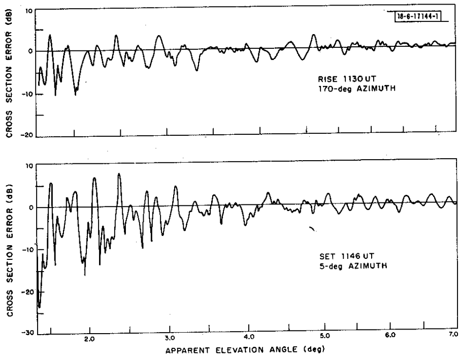
Fig. IV-3. L-band radar observations of a rise and set of a 1-m 2 calibration sphere (LCS-4, Object No. 5398).
