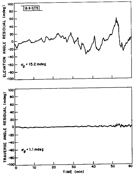
Fig. III-12. Elevation and traverse angle residuals, low-angle data.
