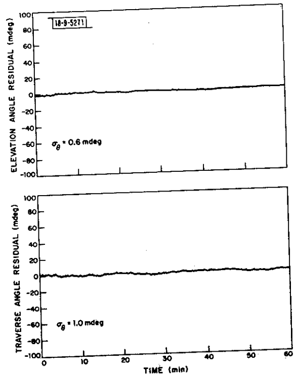
Fig. III-8. Elevation and traverse angle residuals, high-angle data.
