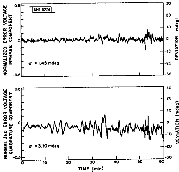
Fig. III-11. Normalized elevation angle error voltages, low-angle data.
