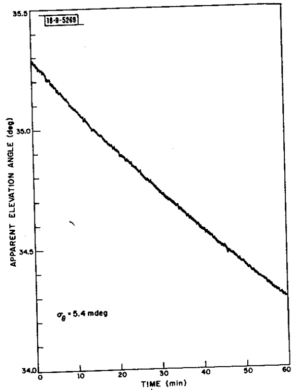
Fig. III-6. Apparent elevation angle at UHF, high-angle data.
