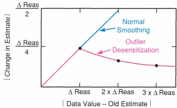
Fig. 15—Outlier-desensitization smoothing algorithm. The red curve is the function, f , described in the equation: \text{new estimate} - \text{old estimate} = f(\text{data value} - \text{old estimate}) .
