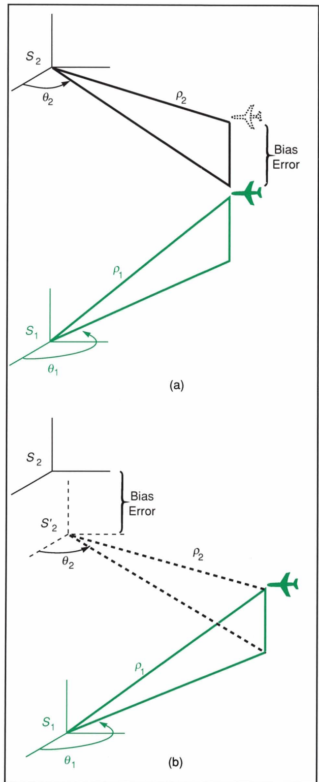
Fig. 13—Bilateration scenarios. (a) Standard. (b) Incremental. S_1 represents the location of sensor 1 and S_2 the location of sensor 2.
